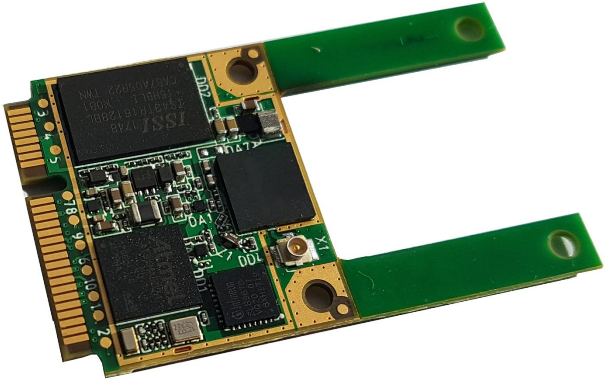
EUT Internal 3d top view – without shielding (photos provided by applicant)
