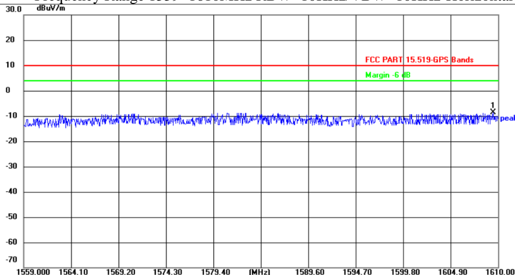
Frequency Range 1559~1610MHz RBW=10KHz/VBW=10KHz-Horizontal
