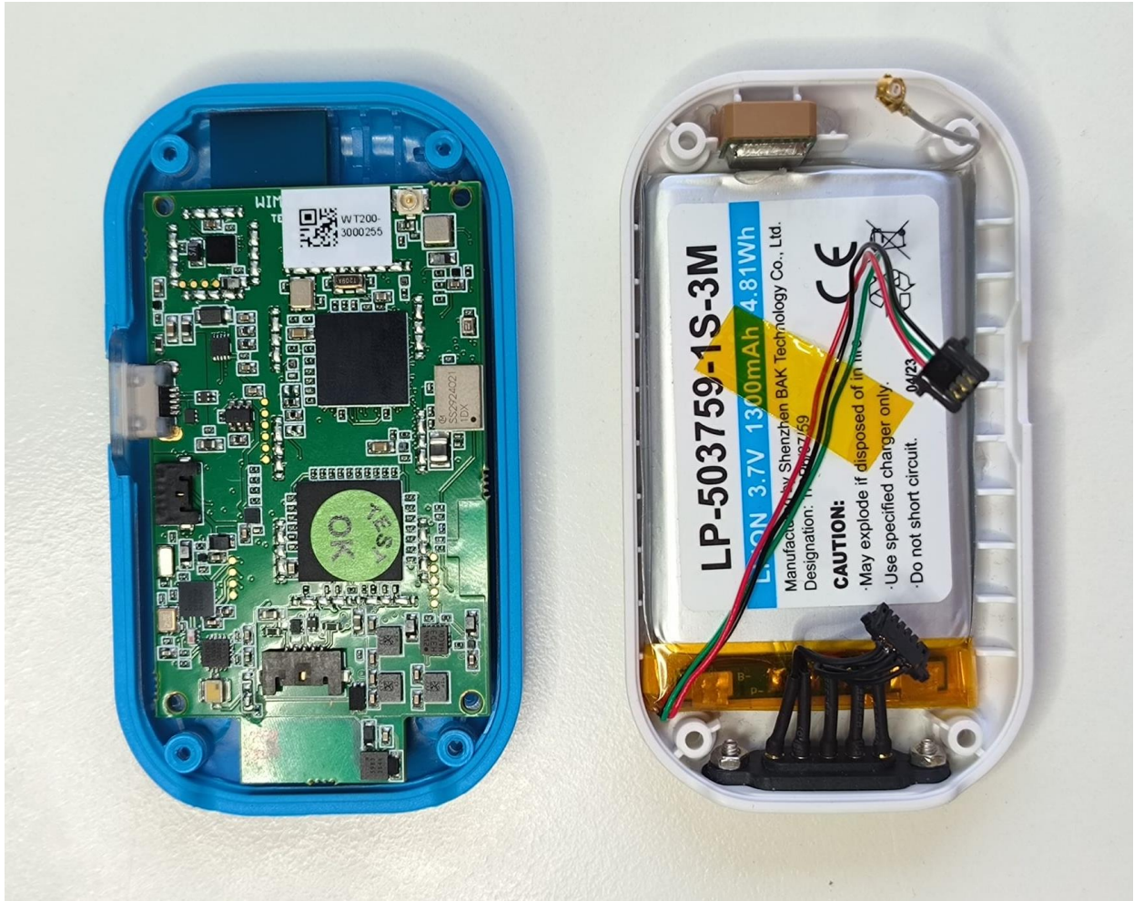
Image 2 –WIMU PRO EVO internal
