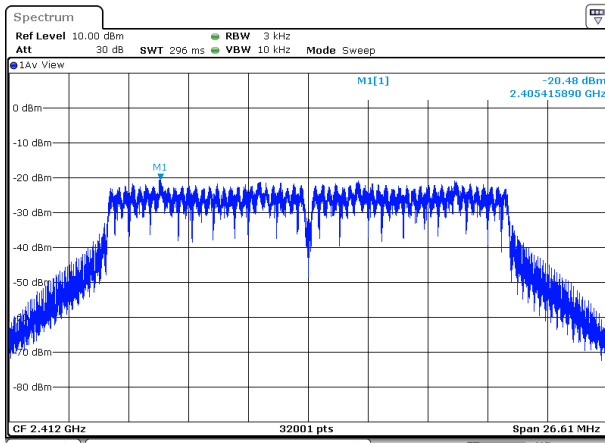
(802.11n20) PSD plot on channel 1
