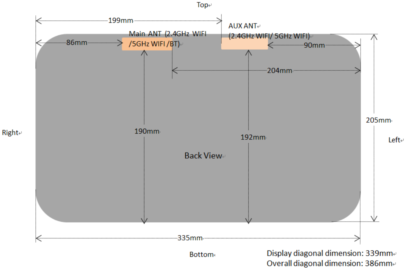
Fig.14.1 EUT Antenna Locations
