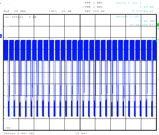
2DH5 on time (Count Pulses) Plot on Channel 39
