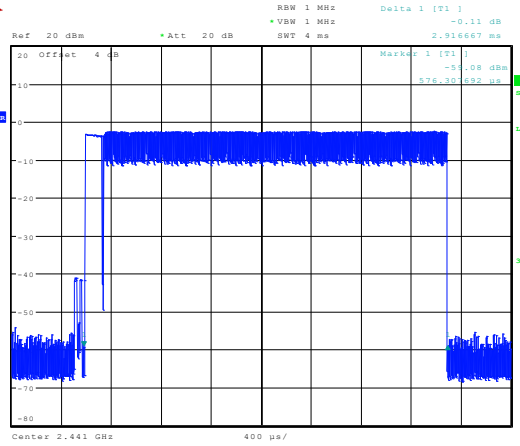
2DH5 on time (One Pulse) Plot on Channel 39
