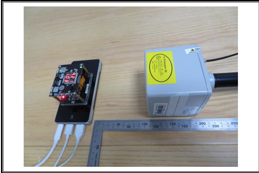
E- FIELD AND H- FIELD STRENGTH MEASUREMENT SETUP-2
