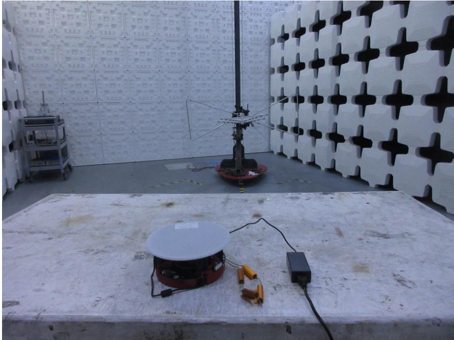
Below 1GHz
