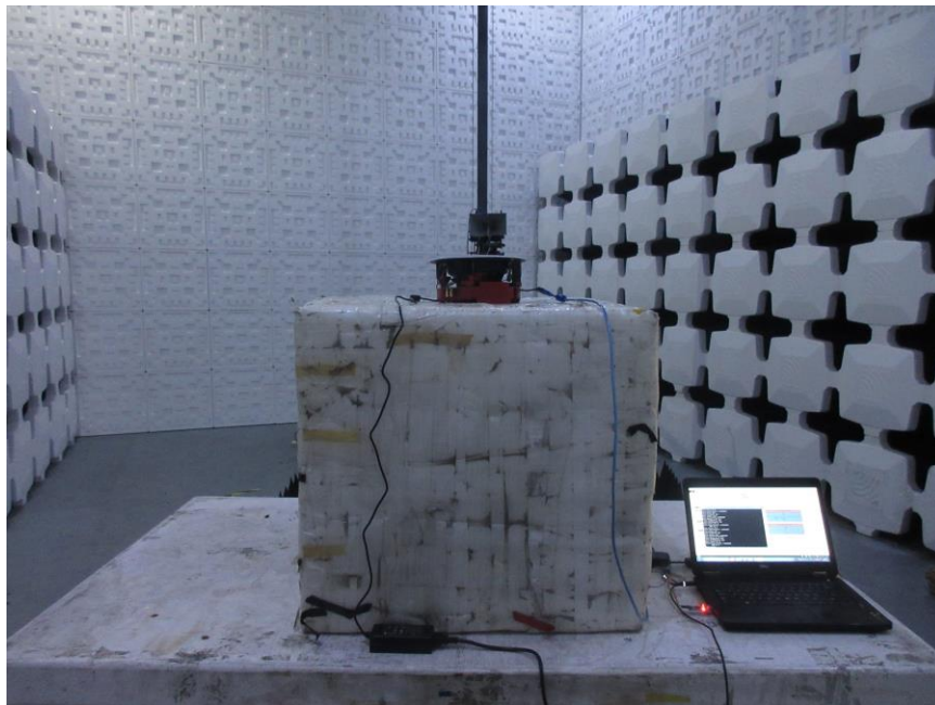
Above 1GHz
