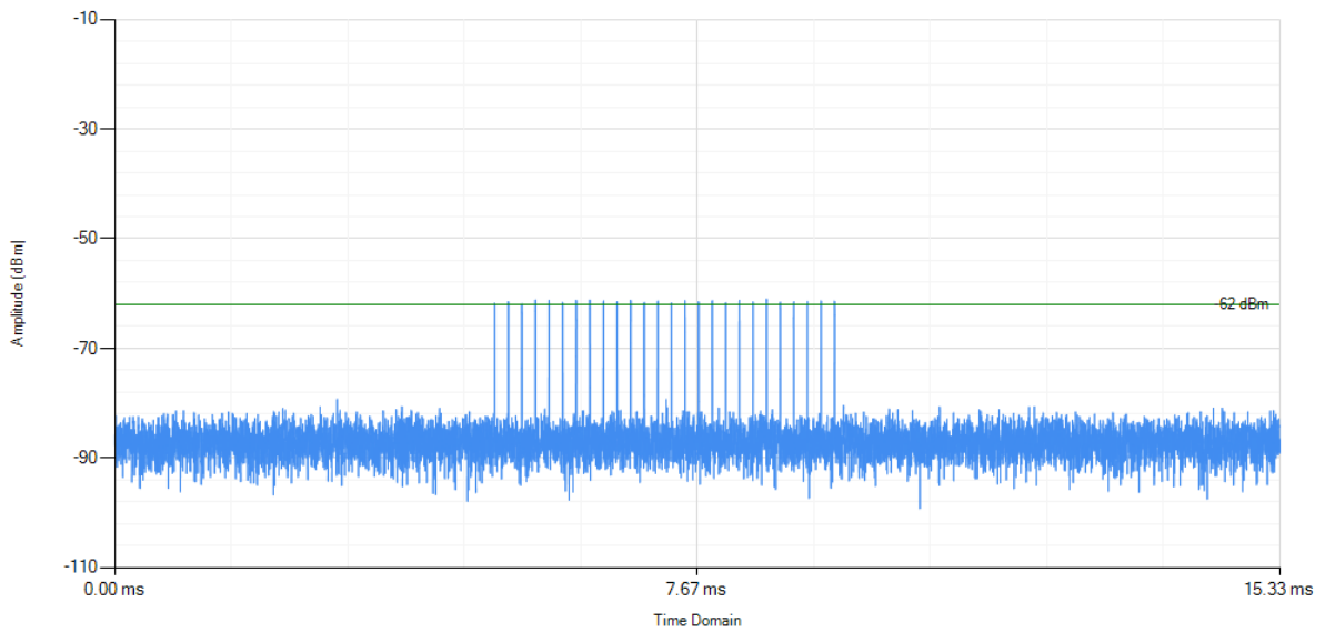
Radar Type 2
