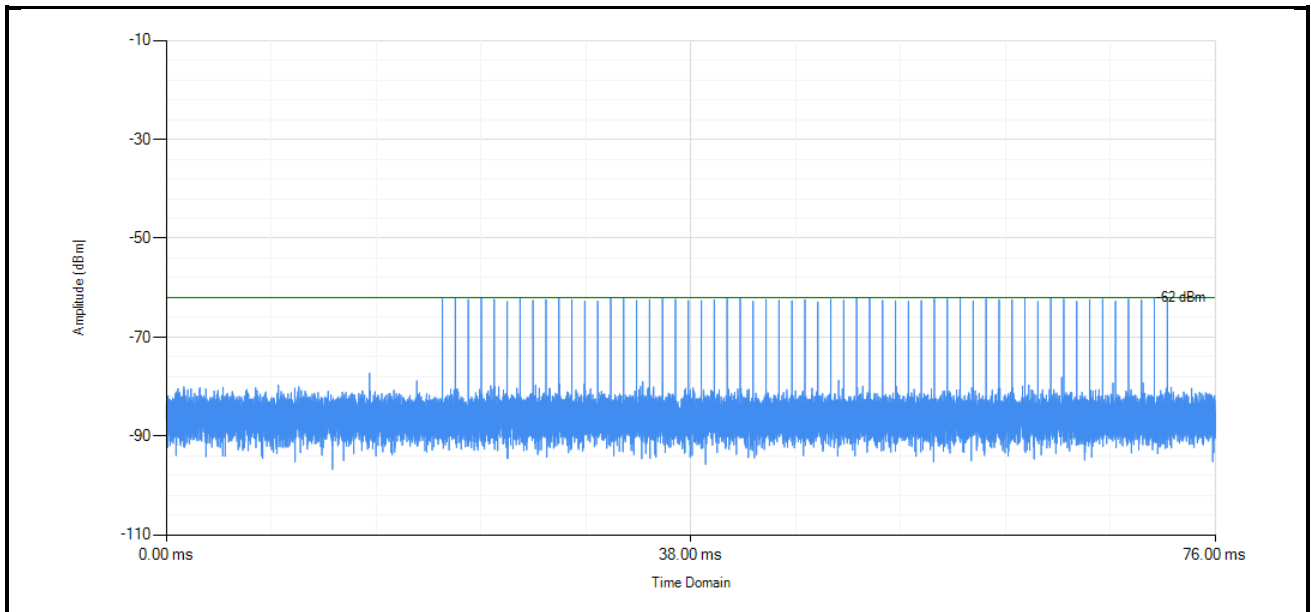
Radar Type 1
