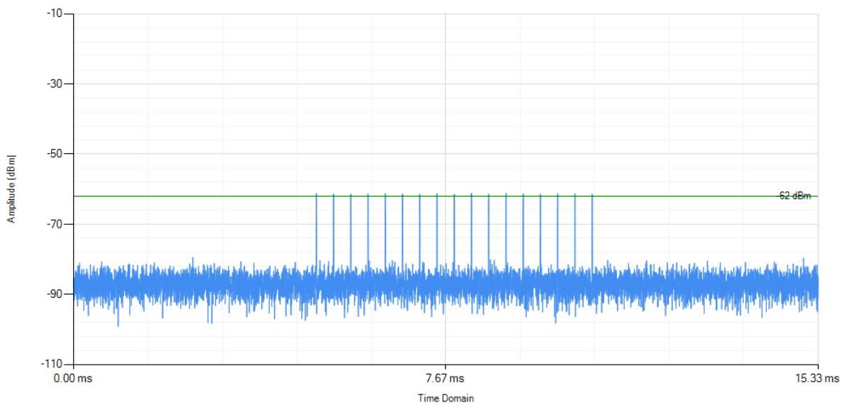
Radar Type 3
