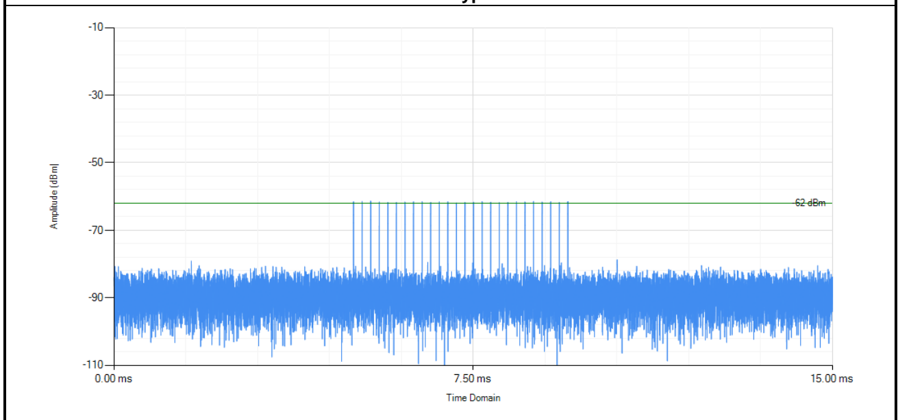
Radar Type 2
