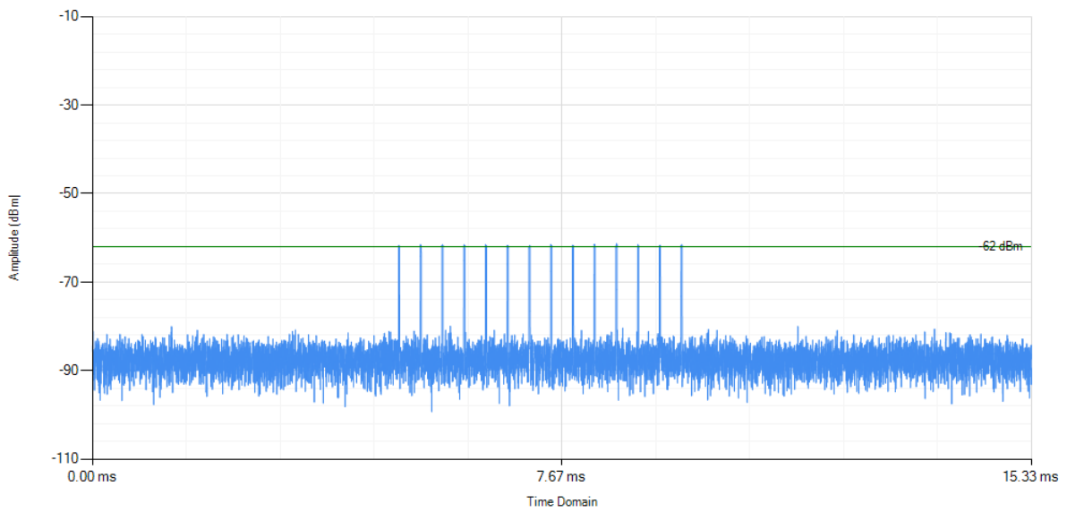
Radar Type 4
