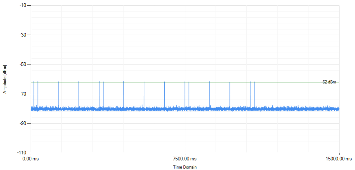
Radar Type 5
