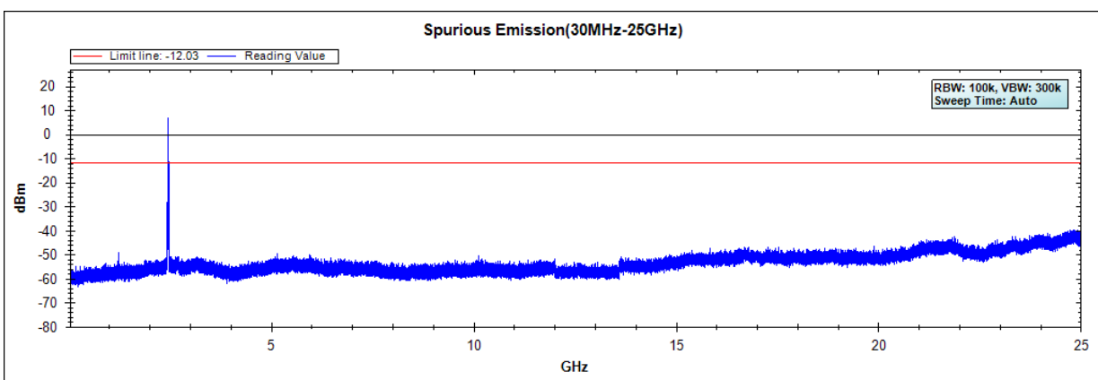
Channel 11 (2462MHz)
