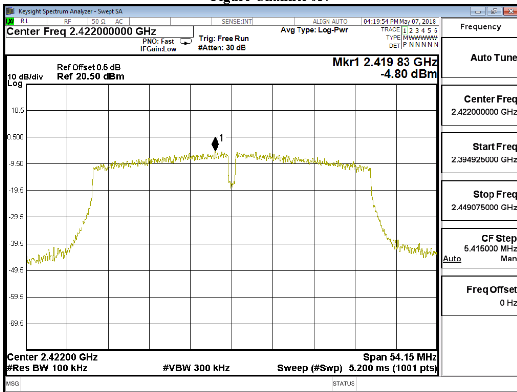
Figure Channel 03:
