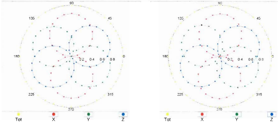
f=600 MHz,TEM
