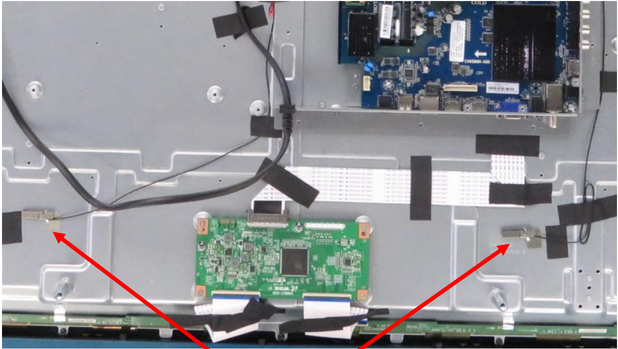
Antenna Location
