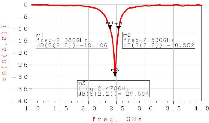
❖Return Loss
