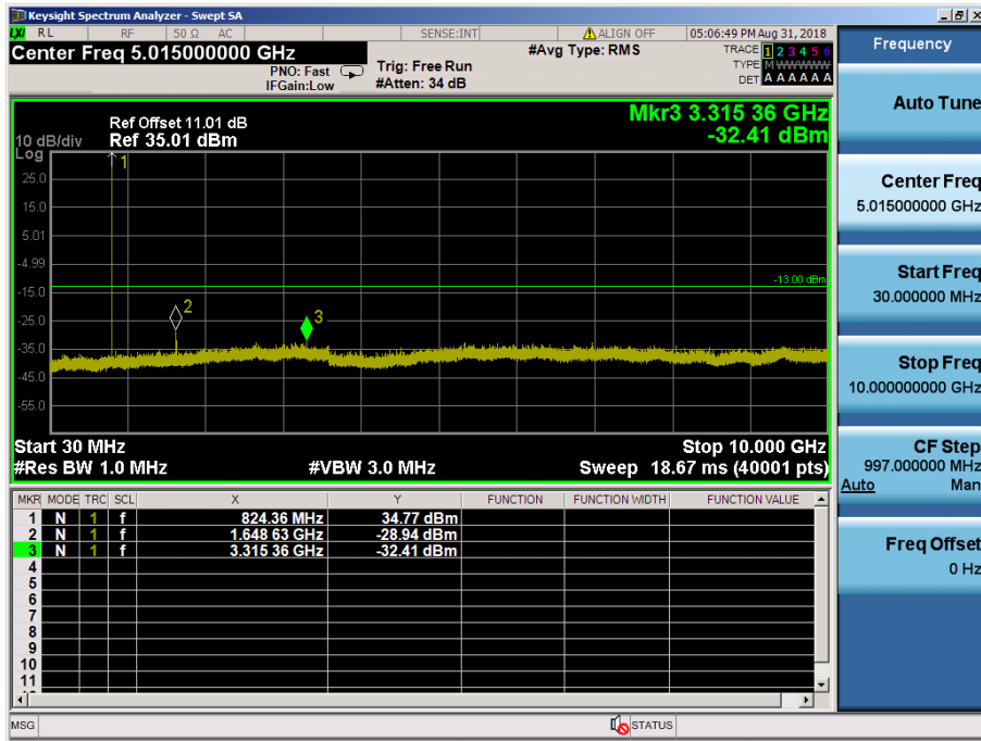
GPRS850 & Channel: 128
