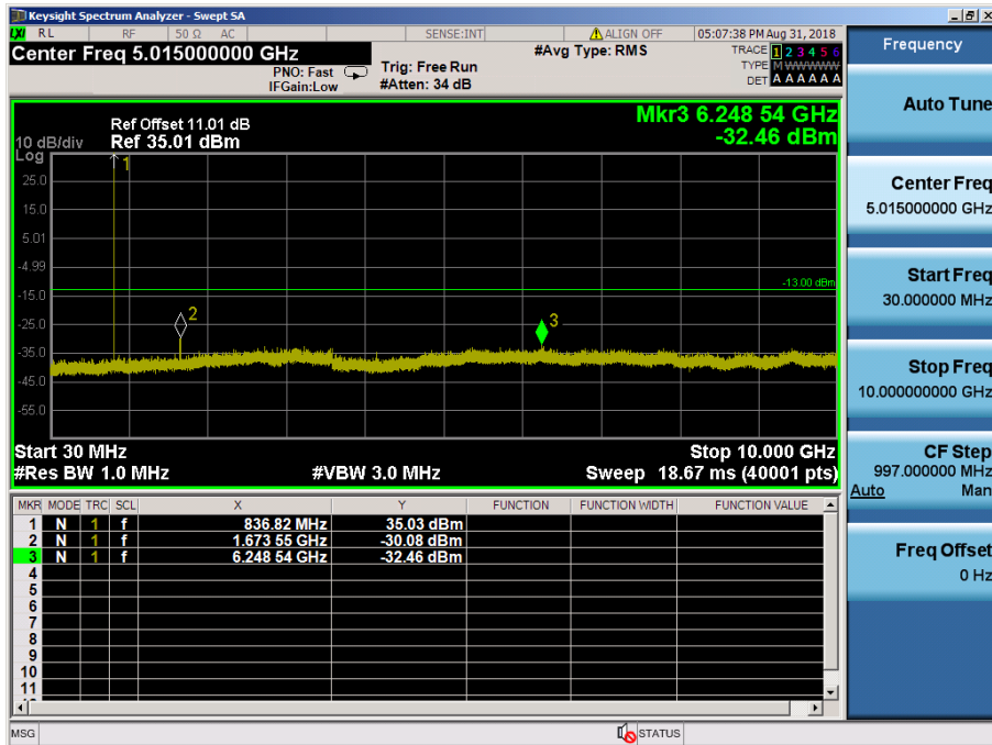
GPRS850 & Channel: 190
