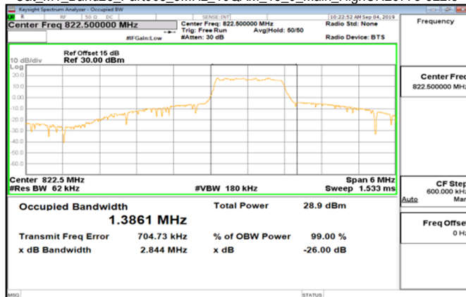
Cat_M1_Band26_Part90s_3MHz_16QAM_15_0_Main_HighCH26775-822.5
