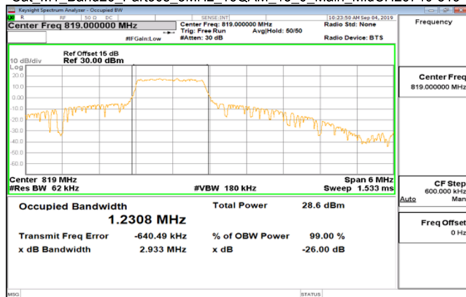
Cat_M1_Band26_Part90s_3MHz_16QAM_15_0_Main_MidCH26740-819
