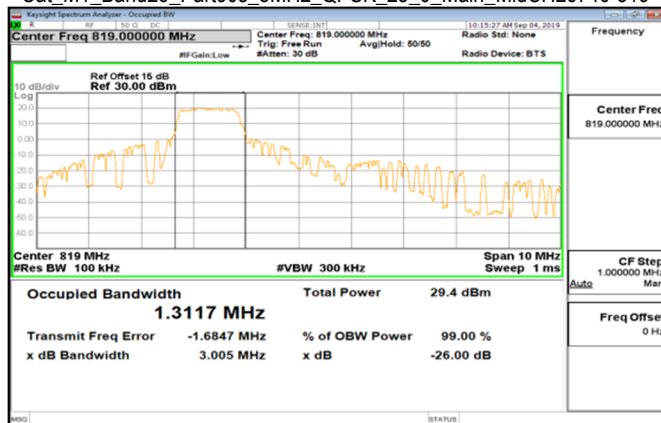
Cat_M1_Band26_Part90s_5MHz_QPSK_25_0_Main_MidCH26740-819
