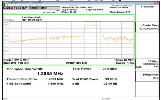
Cat_M1_Band26_Part90s_5MHz_16QAM_25_0_Main_HighCH26765-821.5
