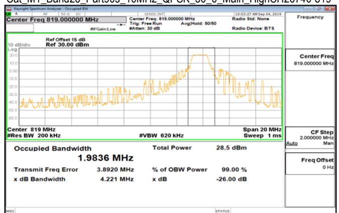
Cat_M1_Band26_Part90s_10MHz_QPSK_50_0_Main_HighCH26740-819
