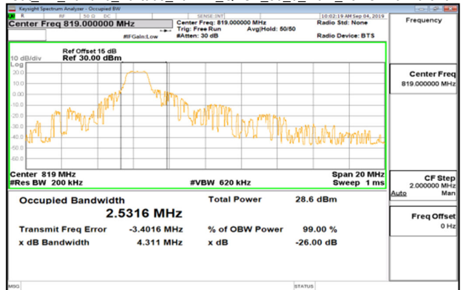
Cat_M1_Band26_Part90s_10MHz_QPSK_50_0_Main_LowCH26740-819
