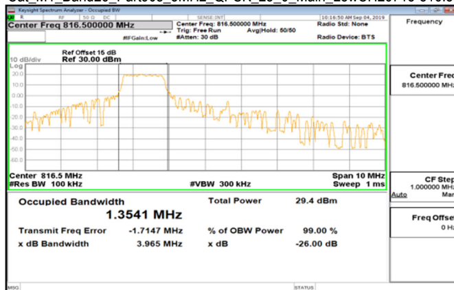
Cat_M1_Band26_Part90s_5MHz_QPSK_25_0_Main_LowCH26715-816.5
