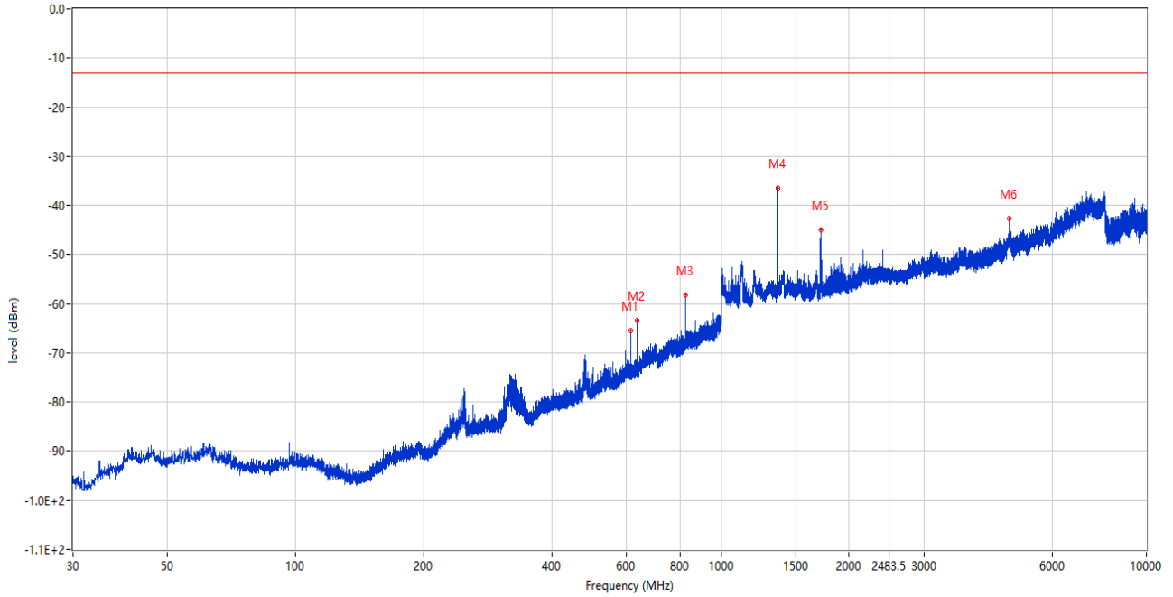
RSE (RF) _FCC PART22&24&27_LTE Band 71 _680_30MHz-10GHz_
