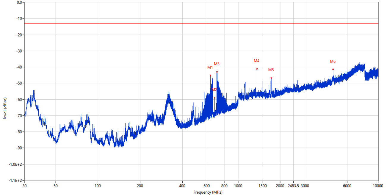
RSE (RF) _FCC PART228&24&27_LTE Band 71 _680_30MHz-10GHz_
