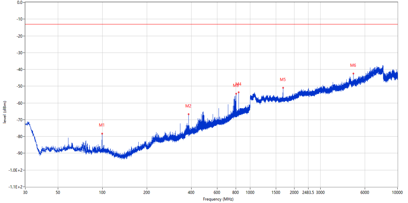
RSE (RF) _FCC PART22&24&27_GSM 850 & CDMA BC0 & WCDMA Band5 & LTE Band 5 & 26_814-849_30MHz-10GHz
