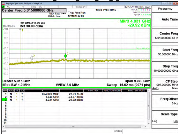
Band5_1.4MHz_QPSK_RB1_0_CH20525
