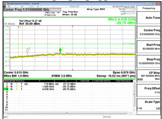
Band12_5MHz_QPSK_RB1_0_CH23155
