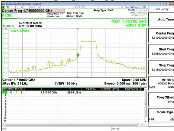
Band4_5MHz_QPSK_RB6_0_CH19975
