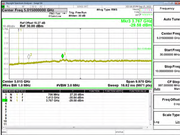
Band12_3MHz_QPSK_RB1_0_CH23165
