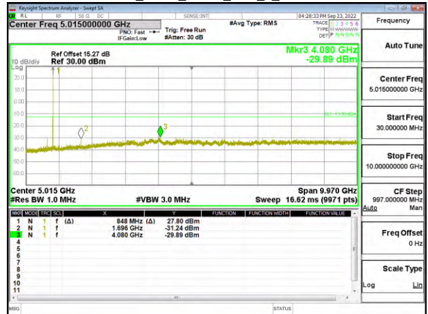
Band5_5MHz_QPSK_RB1_0_CH20625
