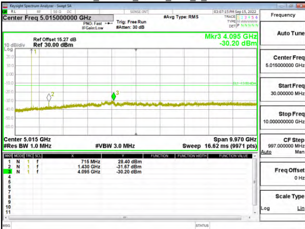
Band12_1.4MHz_QPSK_RB1_0_CH23173
