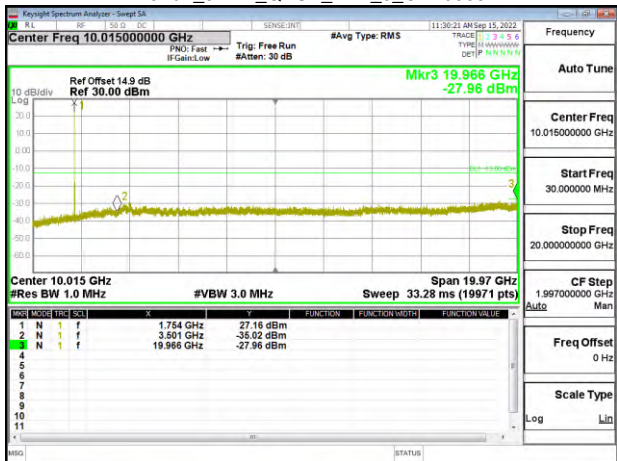
Band4_3MHz_QPSK_RB1_0_CH20385
