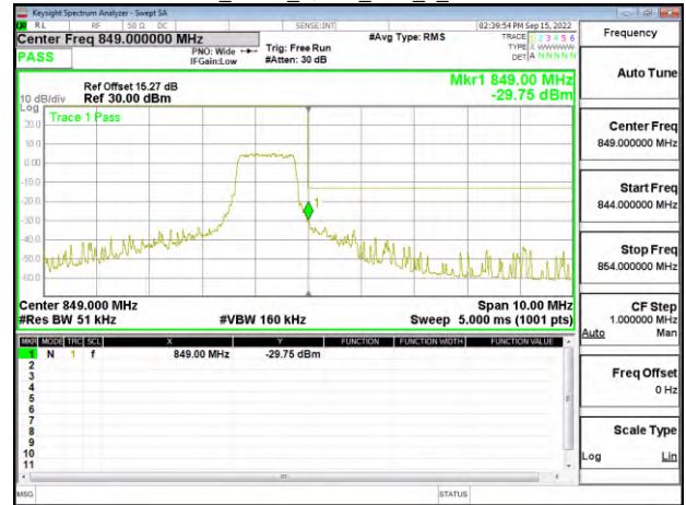
Band5_5MHz_QPSK_RB6_0_CH20625
