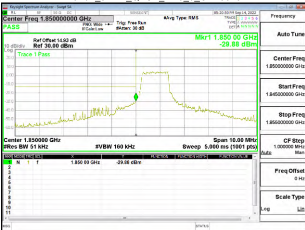
Band2_5MHz_QPSK_RB6_0_CH18625
