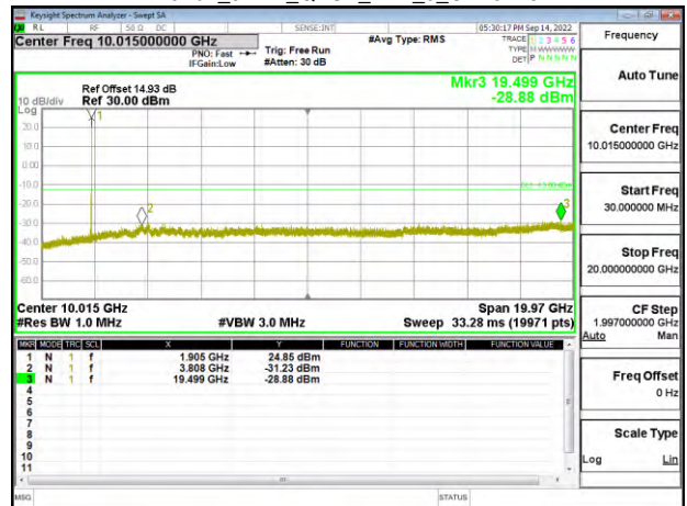
Band2_5MHz_QPSK_RB1_0_CH19175
