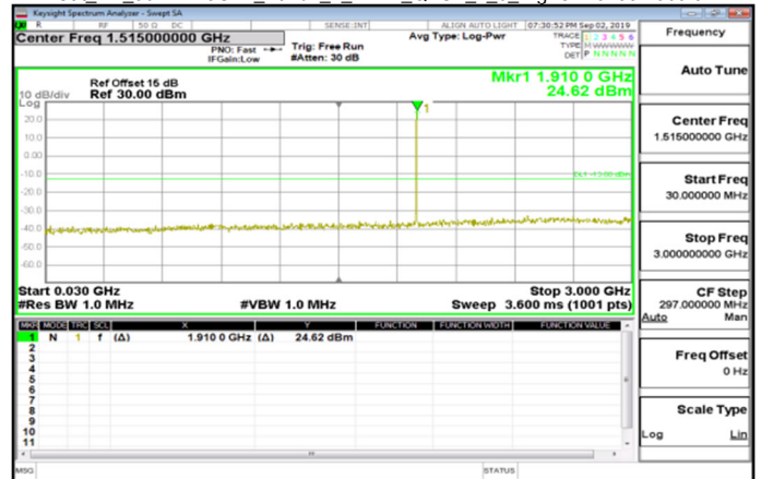
Cat M1_30MHz~3GHz_Band2_1_4MHz_QPSK_1_0_HighCH19193-1909.3
