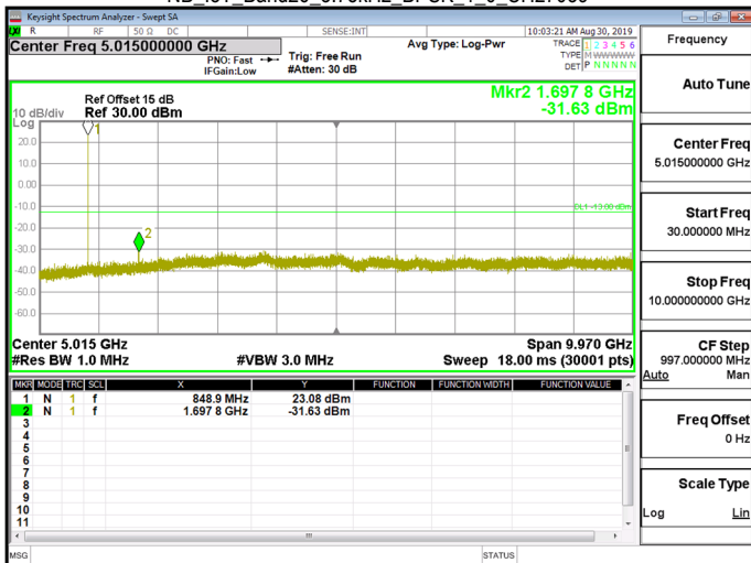
NB_IoT_Band26_3.75kHz_BPSK_1_0_CH27039
