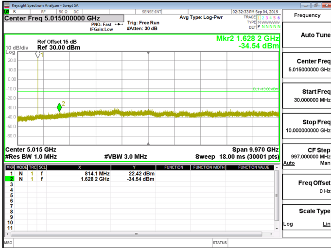
NB_IoT_Band26_Part90s_3.75kHz_BPSK_1_0_CH26740
