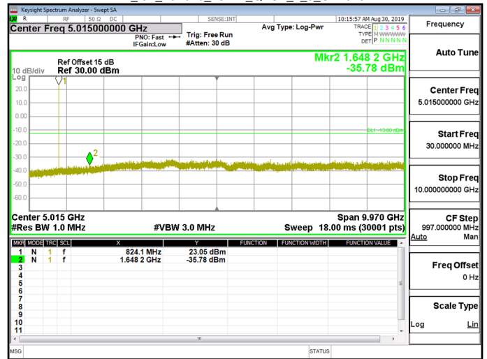
NB_IoT_Band26_15kHz_QPSK_1_0_CH26915
