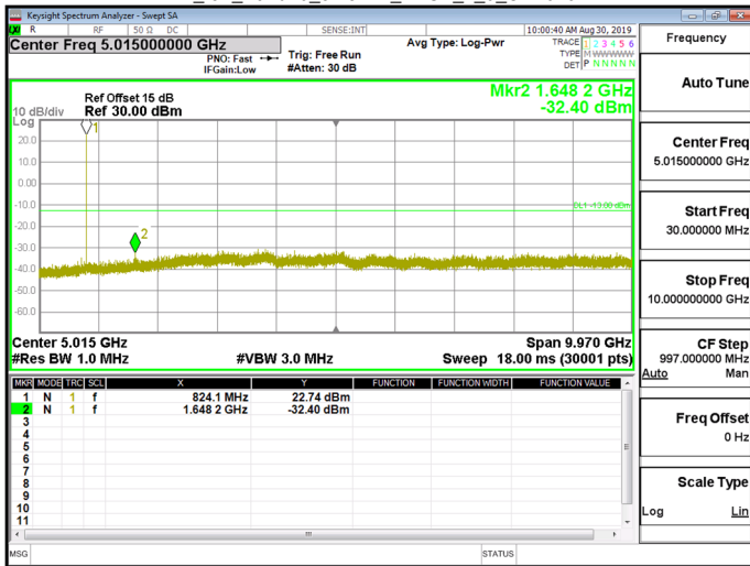
NB_IoT_Band26_3.75kHz_BPSK_1_0_CH26915
