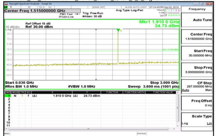
Cat_M1_30MHz~3GHz_Band2_3MHz_QPSK_1_0_HighCH19185-1908.5
