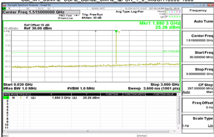
Cat_M1_30MHz~3GHz_Band2_3MHz_QPSK_1_0_MidCH1890-1880
