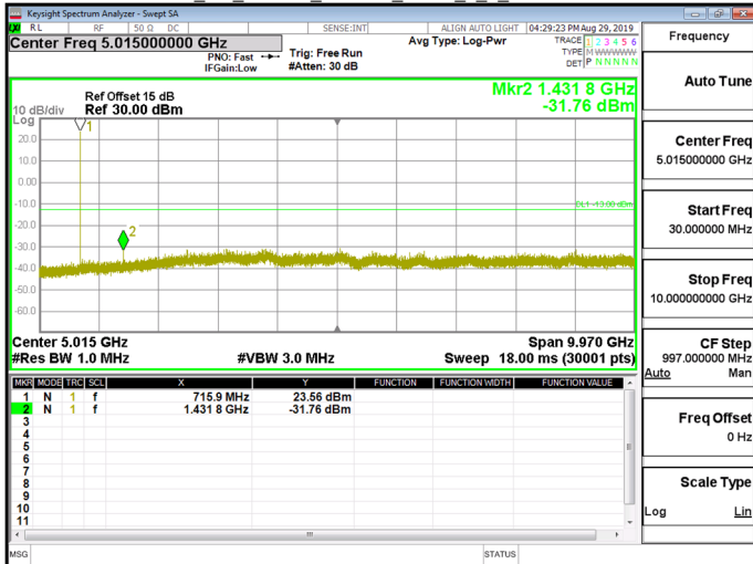
NB_IoT_Band12_3.75kHz_BPSK_1_0_CH23179
