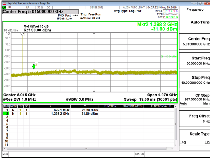
NB_IoT_Band12_3.75kHz_BPSK_1_0_CH23095
