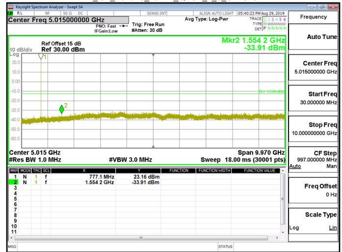
NB_IoT_Band13_15kHz_QPSK_1_0_CH23230
