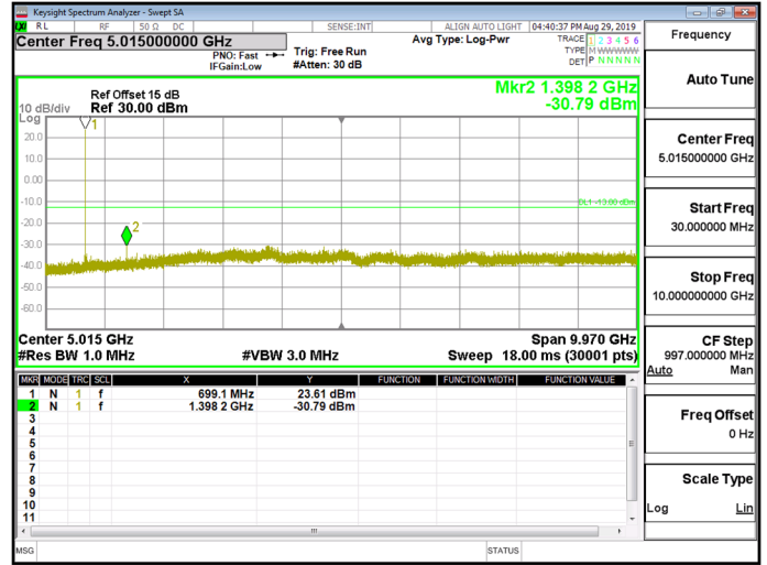
NB_IoT_Band12_15kHz_QPSK_1_0_CH23095
