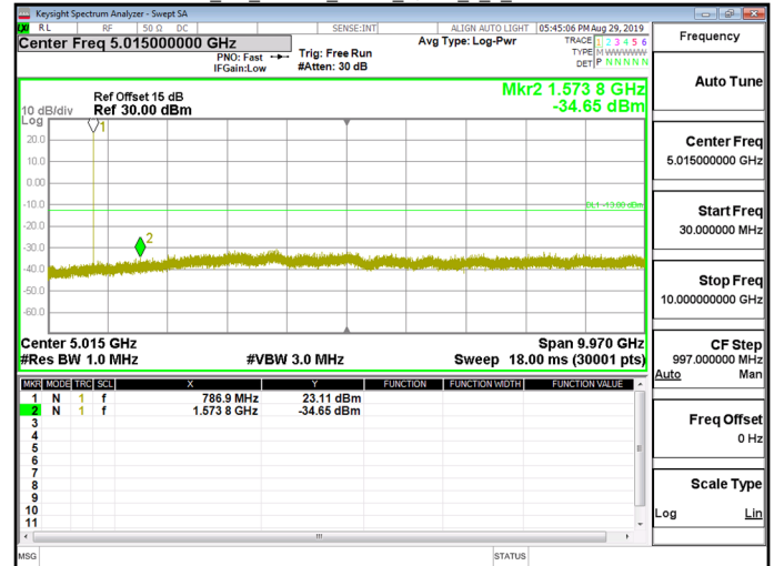
NB_IoT_Band13_15kHz_QPSK_1_0_CH23279
