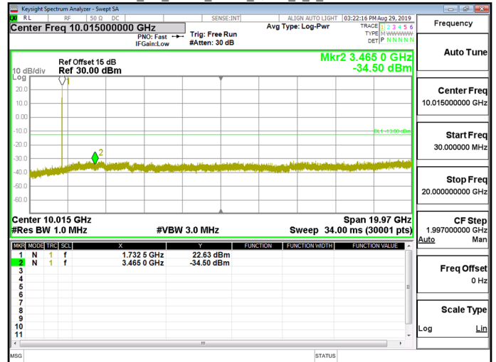
NB_IoT_Band4_15kHz_QPSK_1_0_CH20399
