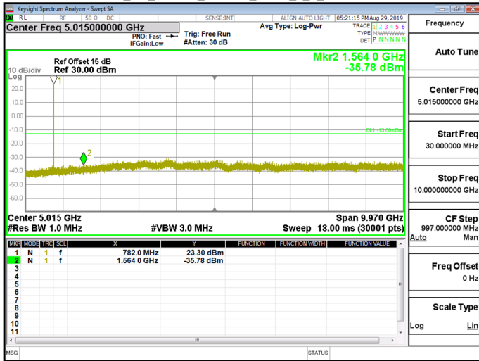
NB_IoT_Band13_3.75kHz_BPSK_1_0_CH23279
