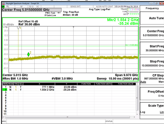
NB_IoT_Band13_3.75kHz_BPSK_1_0_CH23230
