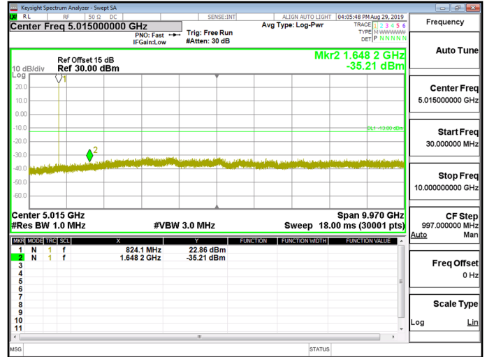
NB_IoT_Band5_15kHz_QPSK_1_0_CH20525
