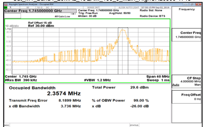
Cat M1_Band4_20MHz_16QAM_100_0_Main_HighCH20300-1745
