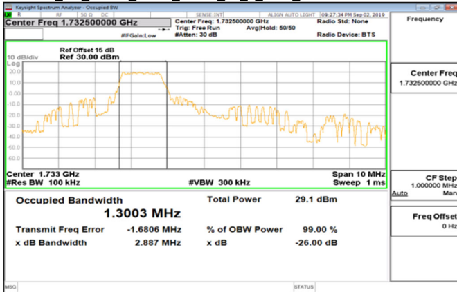
Cat_M1_Band4_5MHz_QPSK_25_0_Main_MidCH20175-1732.5
