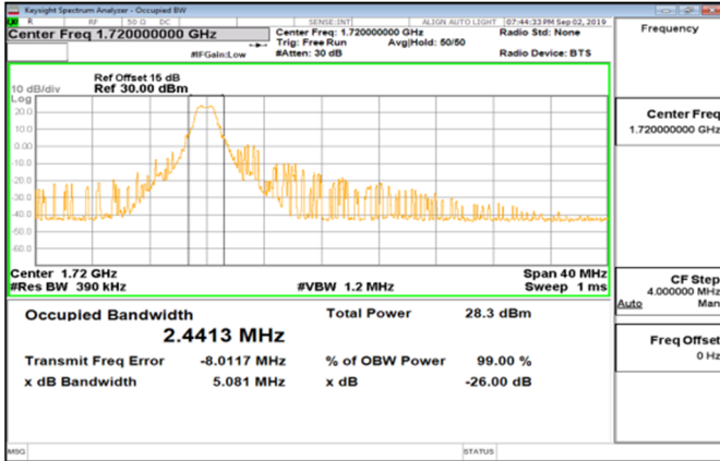
Cat M1_Band4_20MHz_QPSK_100_0_Main_LowCH20050-1720
