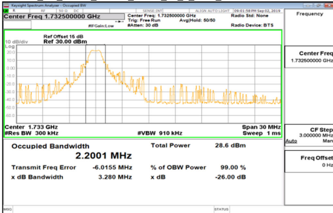
Cat_M1_Band4_15MHz_QPSK_75_0_Main_MidCH20175-1732.5
