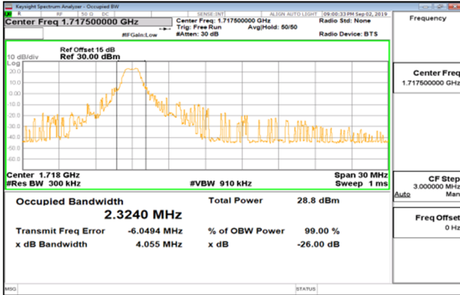
Cat_M1_Band4_15MHz_QPSK_75_0_Main_LowCH20025-1717.5
