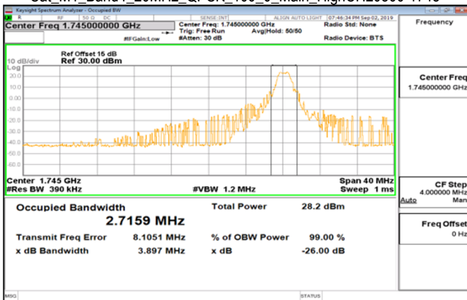
Cat M1_Band4_20MHz_QPSK_100_0_Main_HighCH20300-1745
