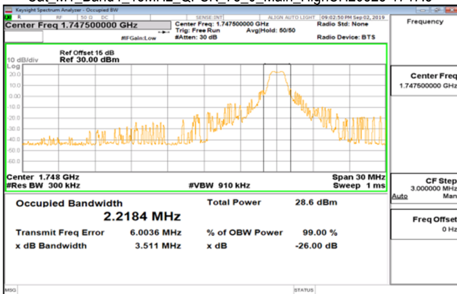
Cat_M1_Band4_15MHz_QPSK_75_0_Main_HighCH20325-1747.5
