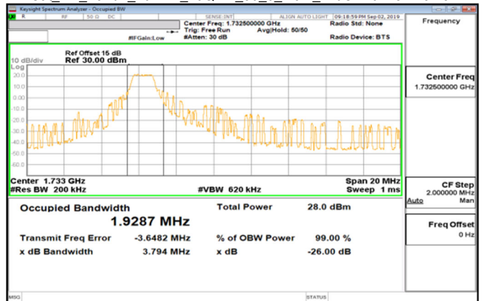
Cat_M1_Band4_10MHz_16QAM_50_0_Main_MidCH20175-1732.5
