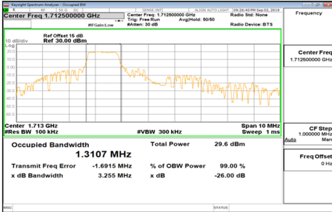
Cat_M1_Band4_5MHz_QPSK_25_0_Main_LowCH1975-1712.5
