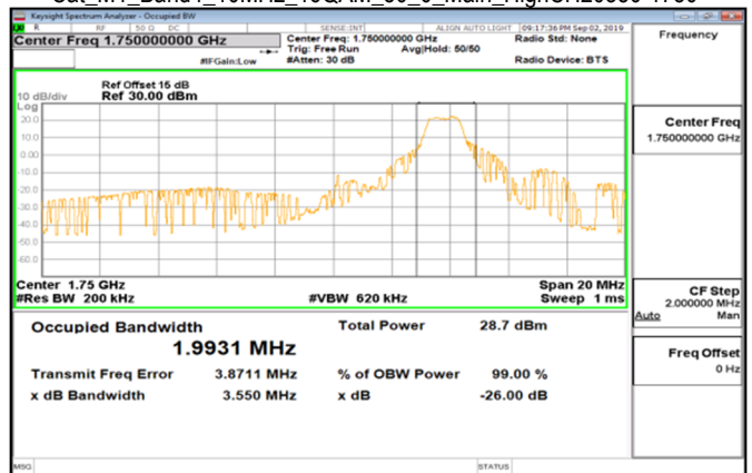
Cat_M1_Band4_10MHz_16QAM_50_0_Main_HighCH20350-1750
