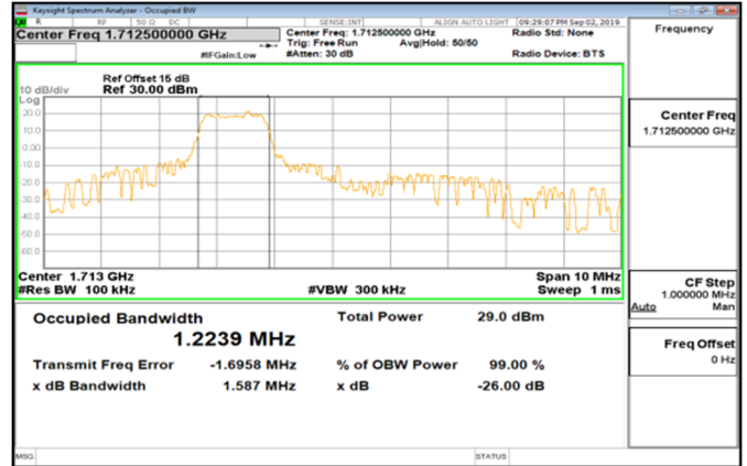
Cat_M1_Band4_5MHz_16QAM_25_0_Main_LowCH1975-1712.5
