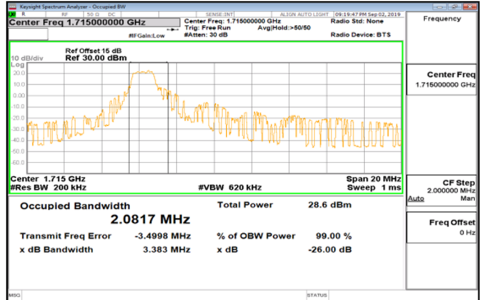
Cat_M1_Band4_10MHz_16QAM_50_0_Main_LowCH20000-1715
