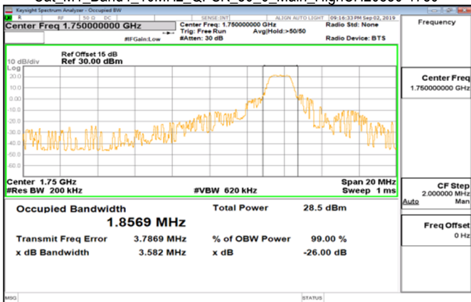
Cat_M1_Band4_10MHz_QPSK_50_0_Main_HighCH20350-1750
