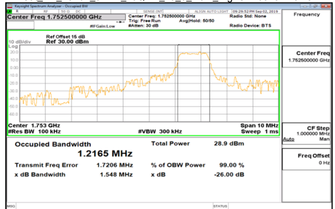
Cat_M1_Band4_5MHz_16QAM_25_0_Main_HighCH20375-1752.5
