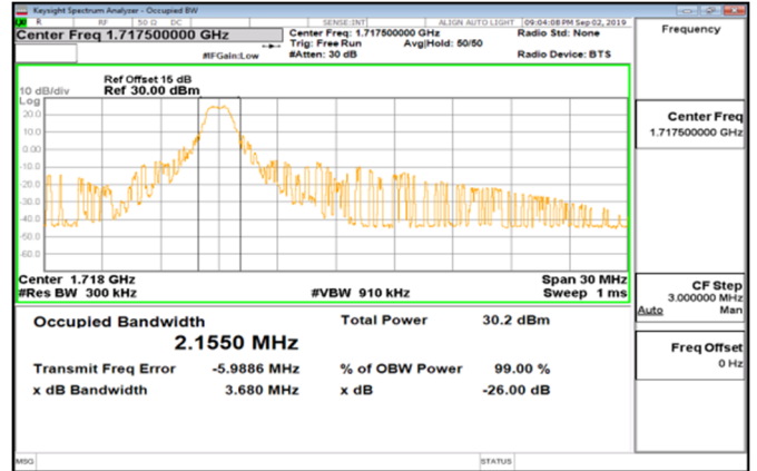
Cat_M1_Band4_15MHz_16QAM_75_0_Main_LowCH20025-1717.5
