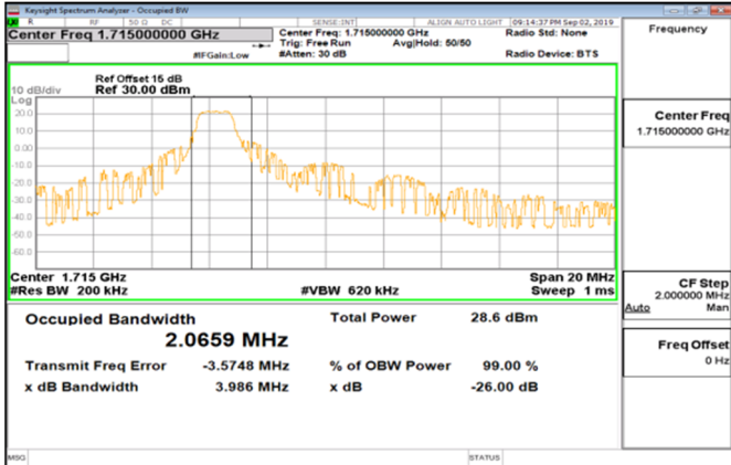
Cat_M1_Band4_10MHz_QPSK_50_0_Main_LowCH20000-1715
