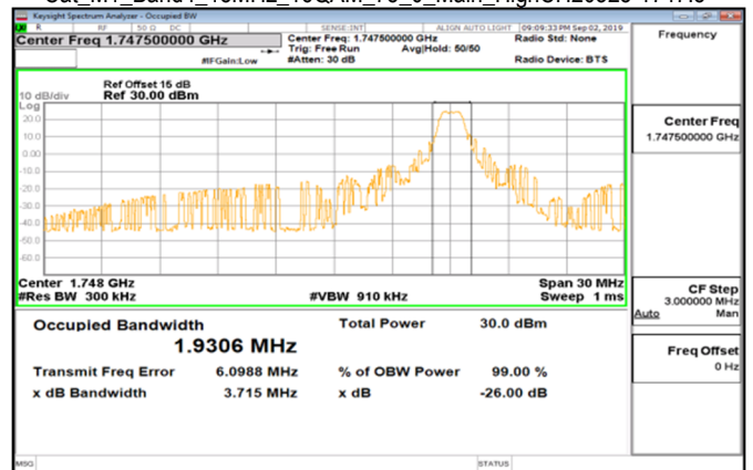
Cat_M1_Band4_15MHz_16QAM_75_0_Main_HighCH20325-1747.5
