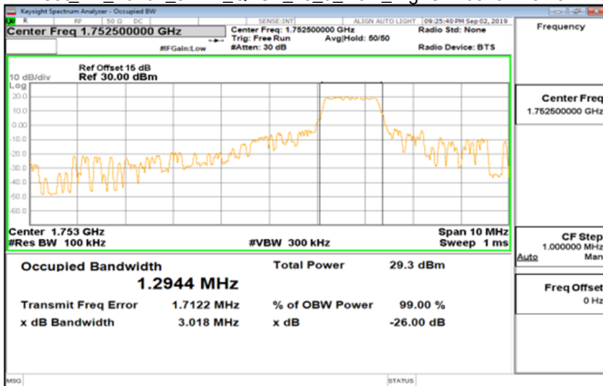
Cat_M1_Band4_5MHz_QPSK_25_0_Main_HighCH20375-1752.5
