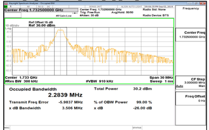
Cat_M1_Band4_15MHz_16QAM_75_0_Main_MidCH20175-1732.5
