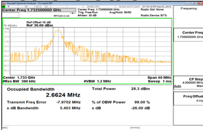
Cat M1_Band4_20MHz_QPSK_100_0_Main_MidCH20175-1732.5
