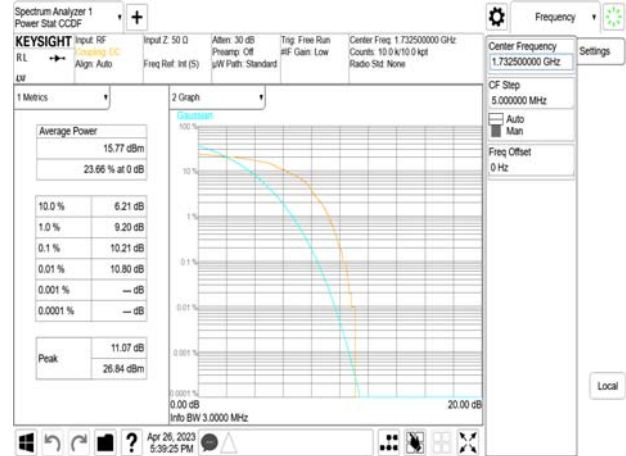
Band4_3MHz_16QAM_RB5_0_1_CH20385
