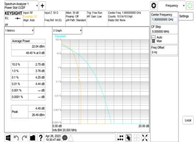
Band2_20MHz_16QAM_RB5_0_15_CH19100
