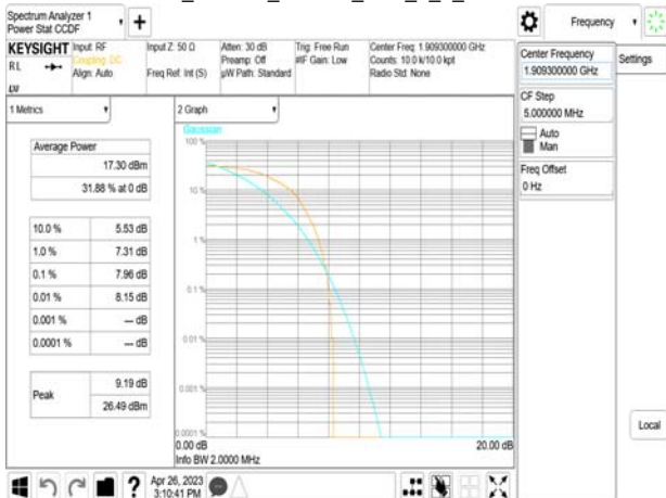
Band2_1.4MHz_16QAM_RB5_0_0_CH19193
