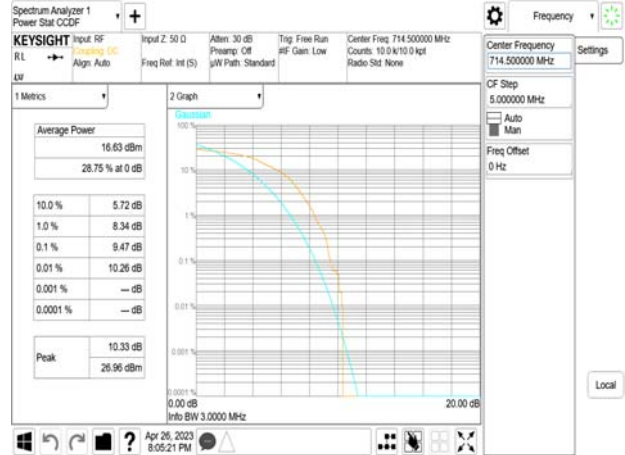
Band12_3MHz_16QAM_RB5_0_1_CH23165
