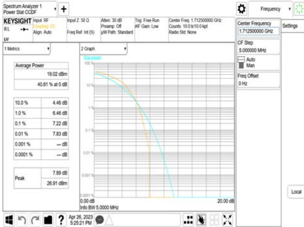
Band4_5MHz_16QAM_RB5_0_0_CH20175
