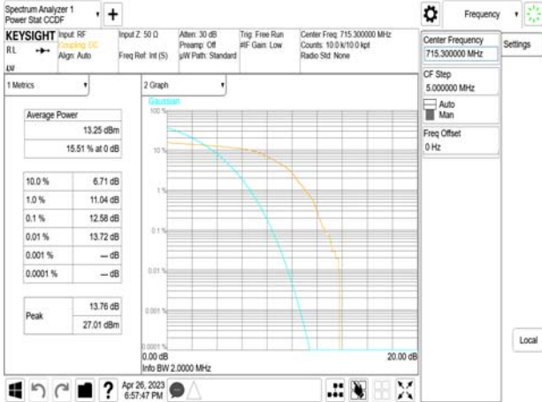
Band12_1.4MHz_16QAM_RB5_0_0_CH23173
