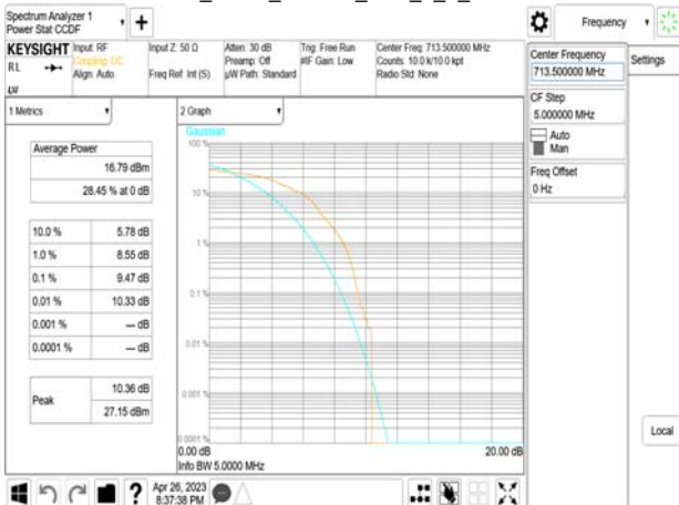
Band12_5MHz_16QAM_RB5_0_3_CH23155
