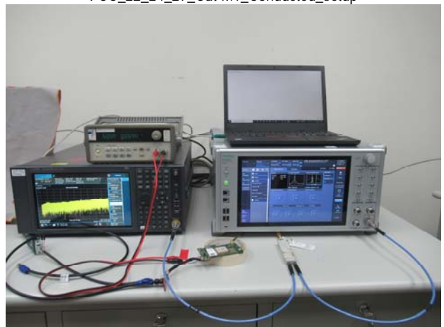
FCC_22_24_27_Cat-M1_Conducted_setup
