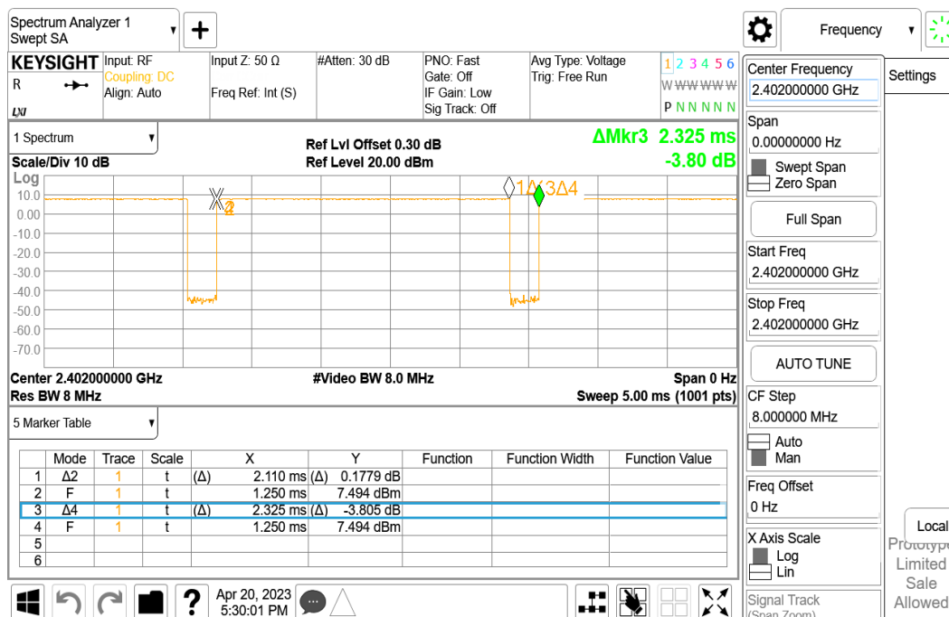
BLE_1M_LowCH00-2402
