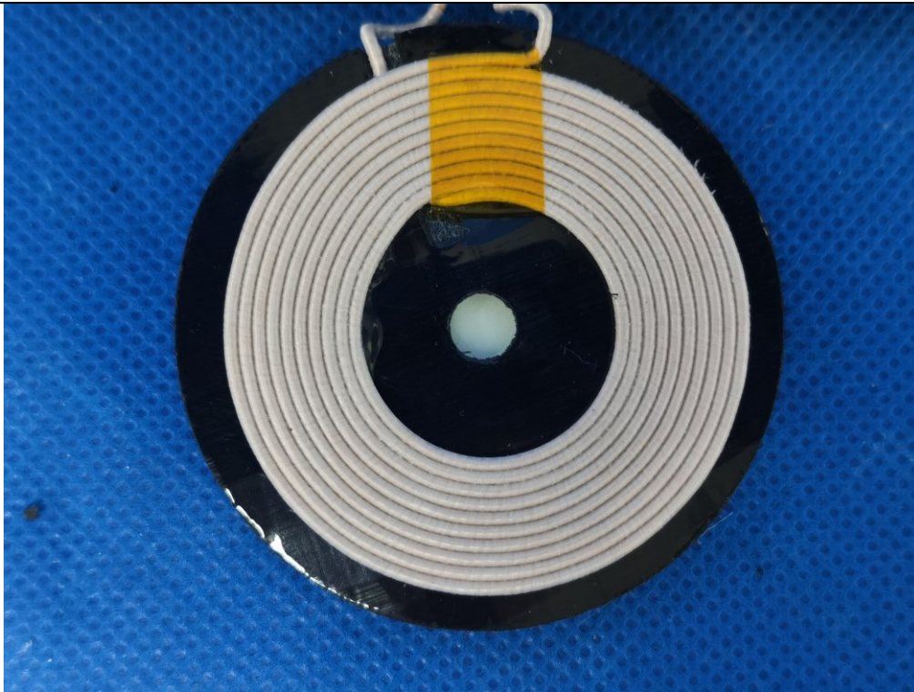
(5) EUT Photo----Antenna
