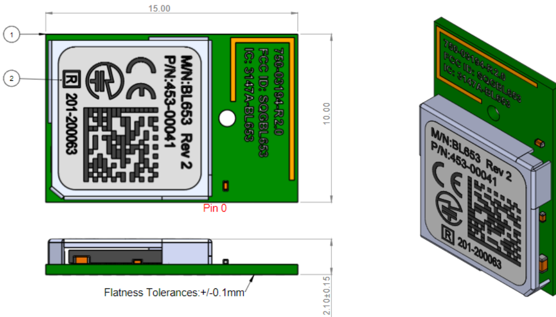
Figure 15: Mechanical Details - Trace Pin
