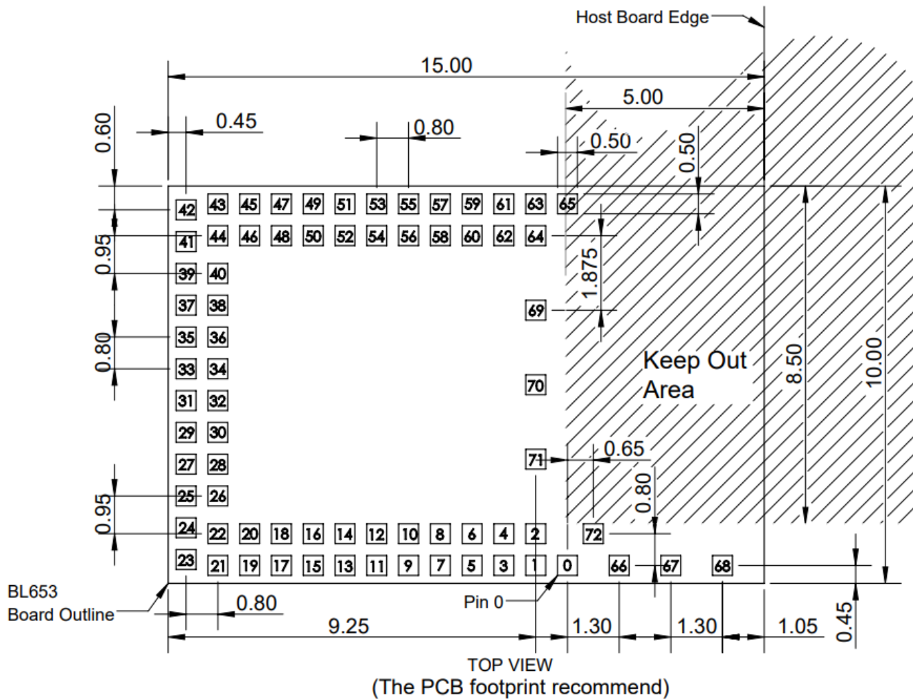
Figure 16: Land pattern and Keep-out for the 453-00039
