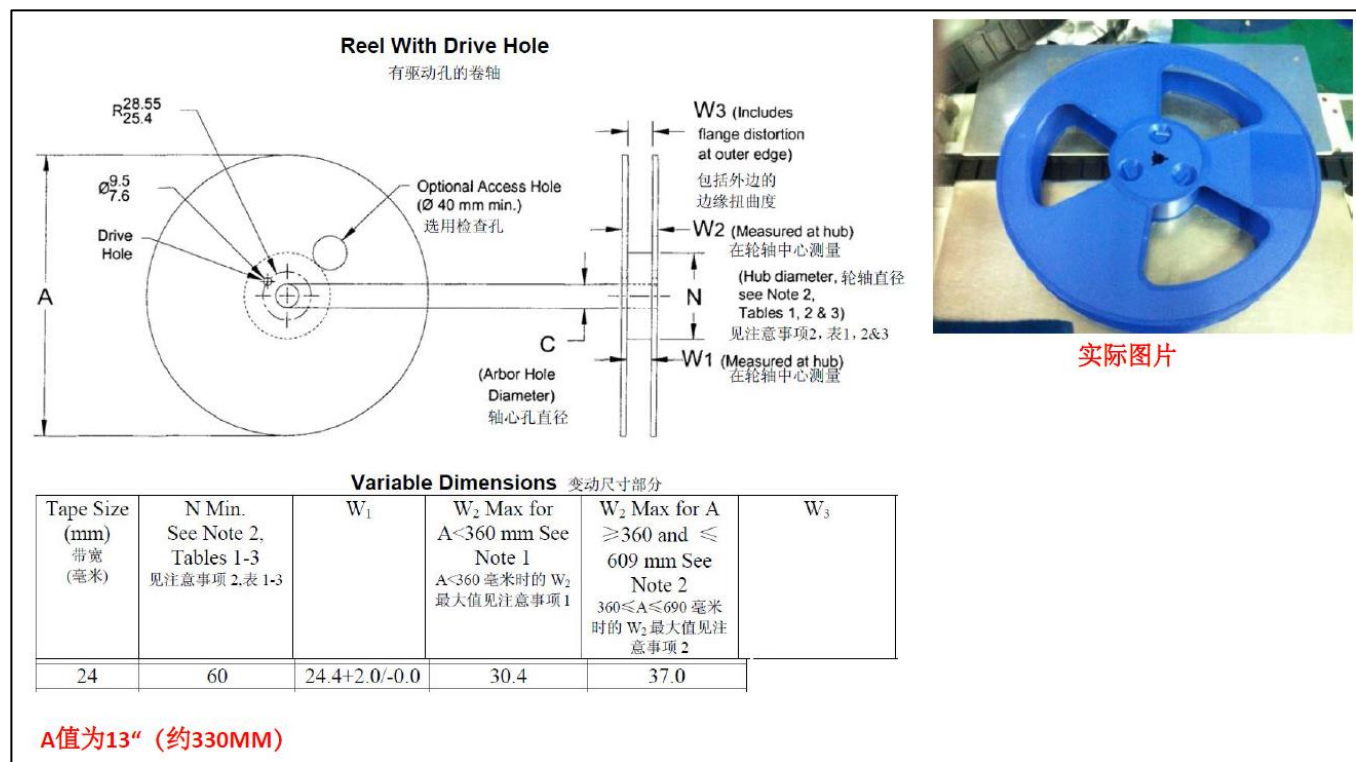
Figure 17: Reel specifications
