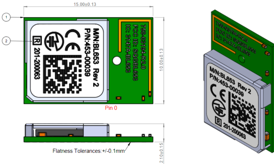
Figure 14: Mechanical Details - Integrated Antenna
