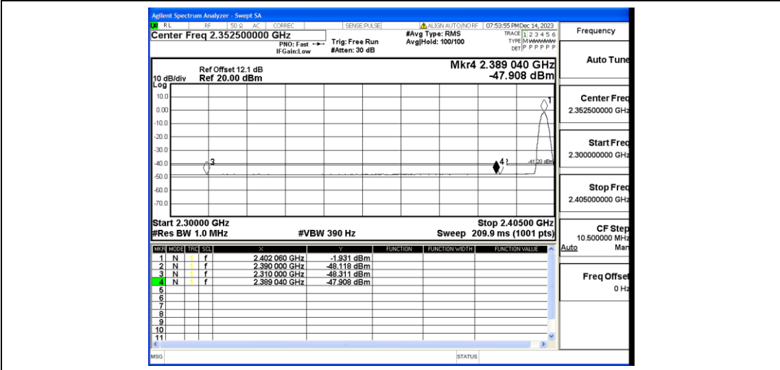
3DH5_Ant1_Low_2402_Peak
