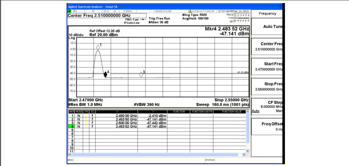
3DH5_Ant1_High_2480_Peak
