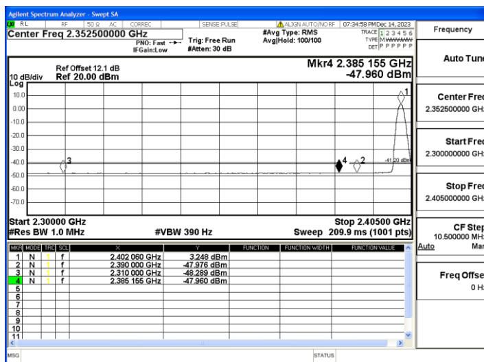
DH5_Ant1_Low_2402_Peak
