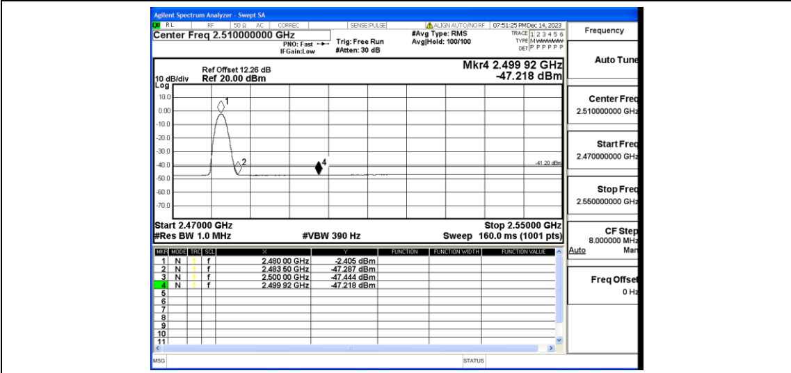
2DH5_Ant1_High_2480_Peak
