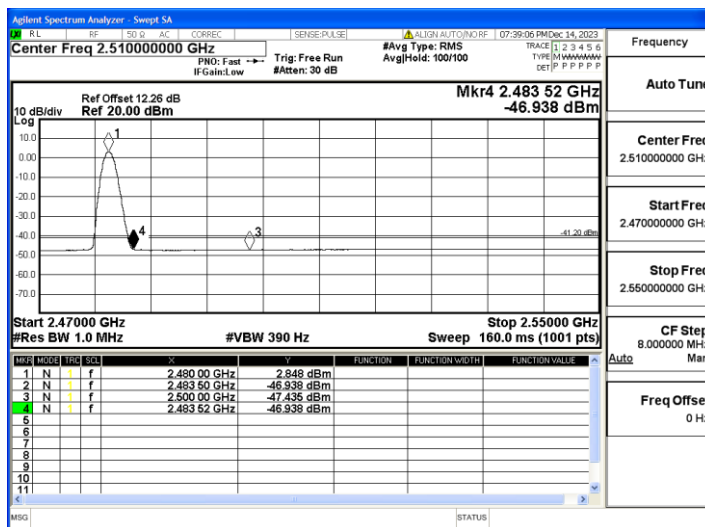
DH5_Ant1_High_2480_Peak
