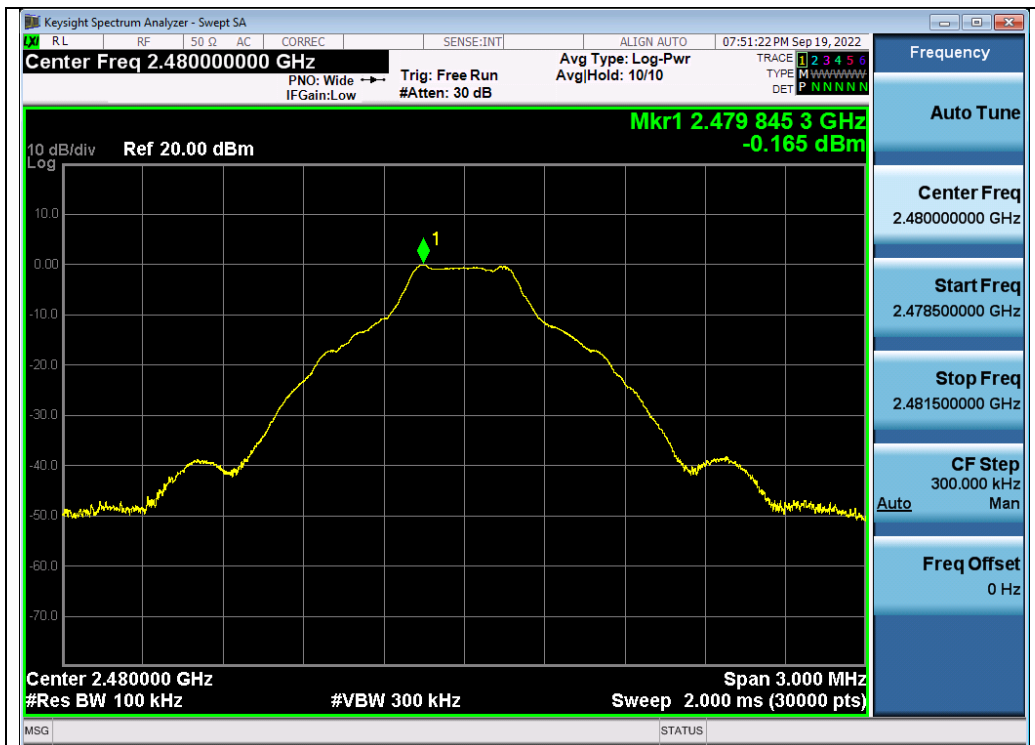
Test_Graph_BR_ANT1_2480_1Mbps_Reference Level
