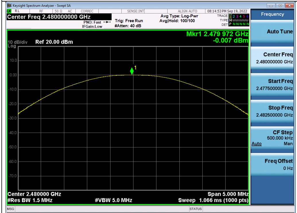
Test_Graph_EDR_ANT1_2480_3Mbps_Peak Power
