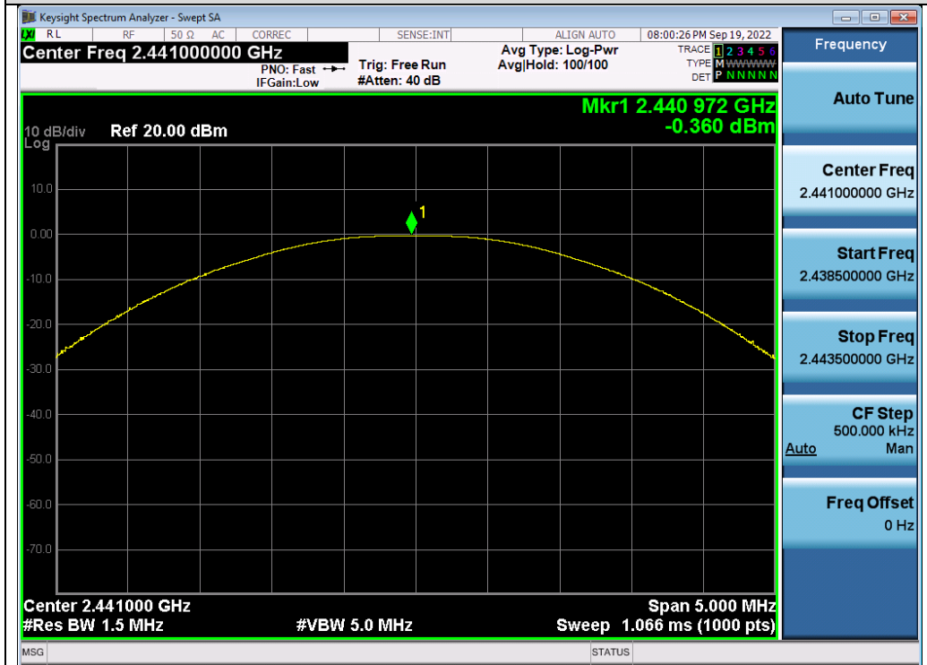
Test_Graph_EDR_ANT1_2441_2Mbps_Peak Power
