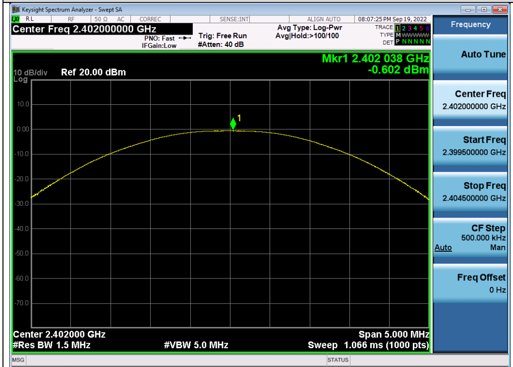
Test_Graph_EDR_ANT1_2402_3Mbps_Peak Power
