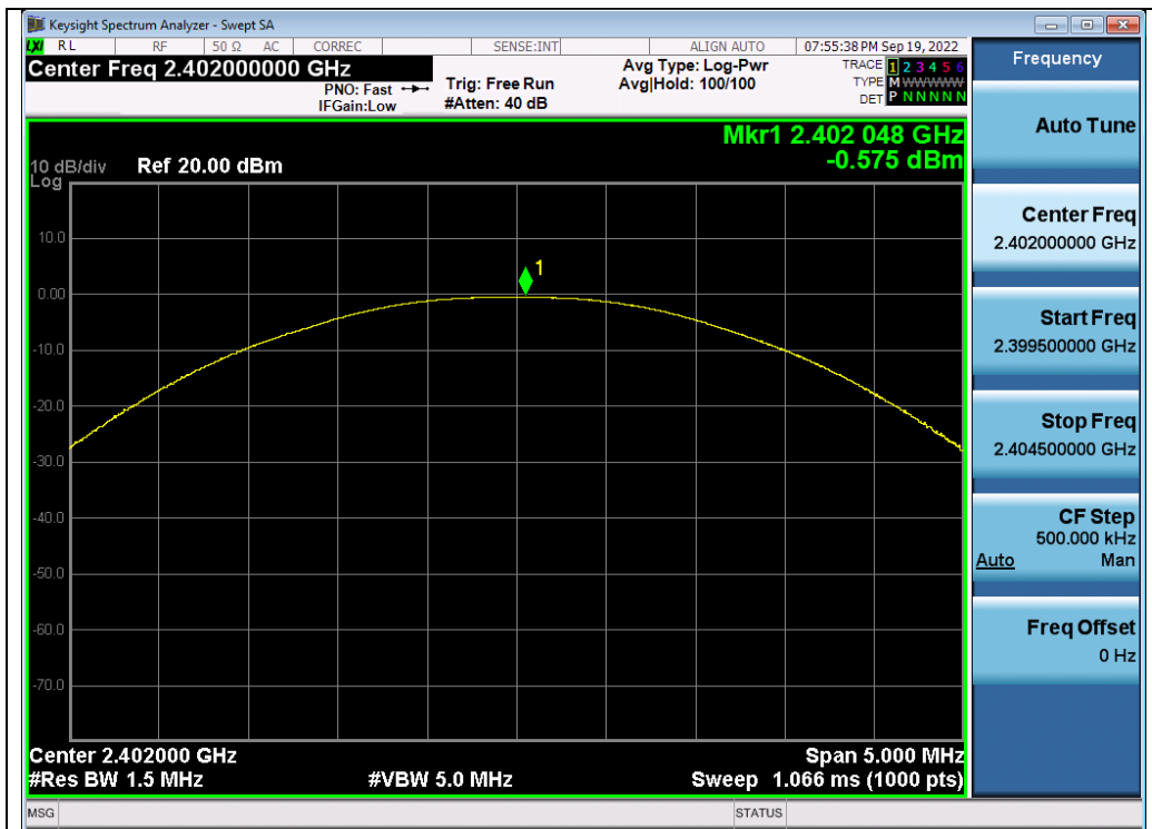
Test_Graph_EDR_ANT1_2402_2Mbps_Peak Power
