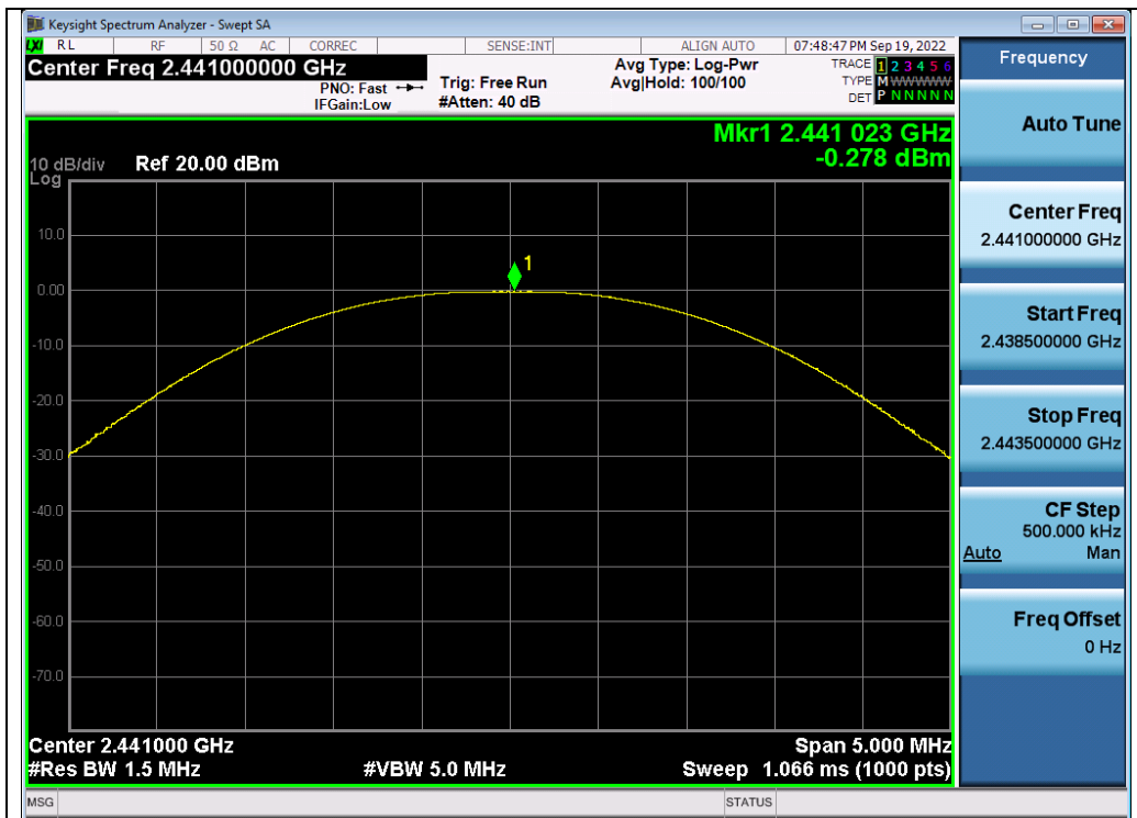
Test_Graph_BR_ANT1_2441_1Mbps_Peak Power
