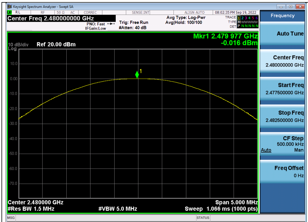
Test_Graph_EDR_ANT1_2480_2Mbps_Peak Power
