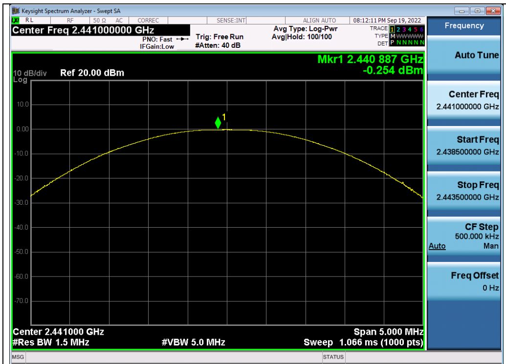
Test_Graph_EDR_ANT1_2441_3Mbps_Peak Power
