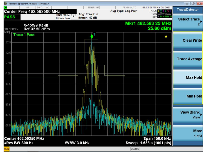
Channel 1: 462.5625MHz
