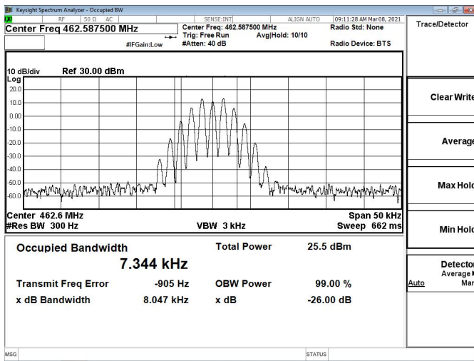
Channel 2: 462.5875MHz
