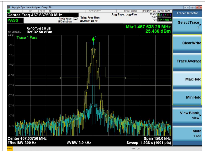
Channel 11: 467.6375MHz
