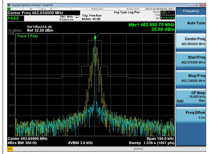
Channel 19: 462.6500MHz
