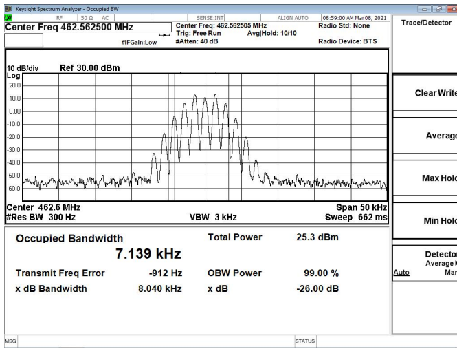
Channel 1: 462.5625MHz
