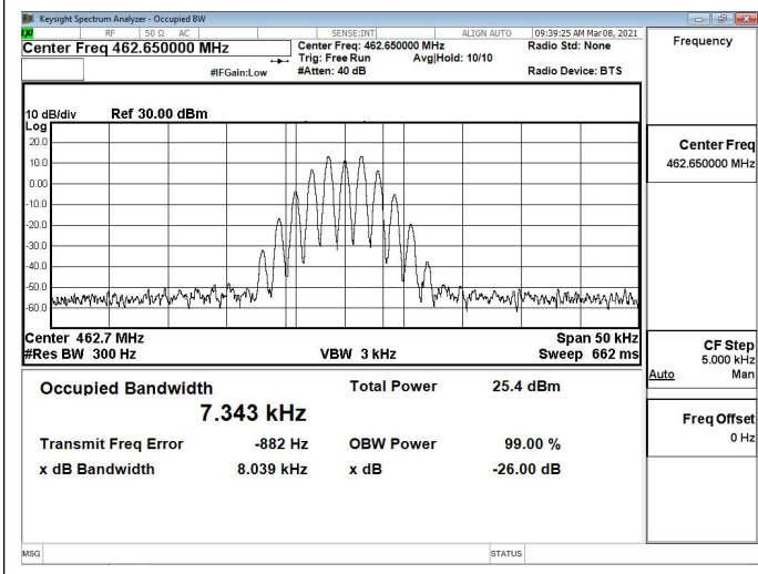
Channel 19: 462.6500MHz
