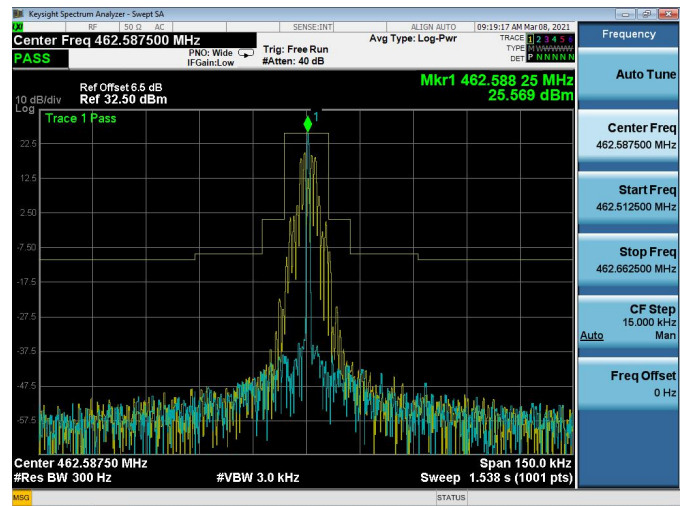
Channel 2: 462.5875MHz
