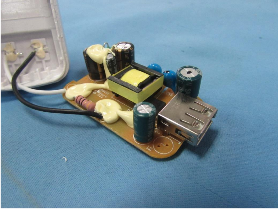
Internal view of adapter
