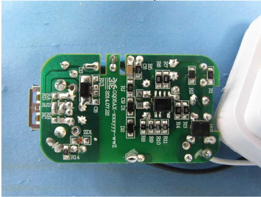
PCB view of adapter
