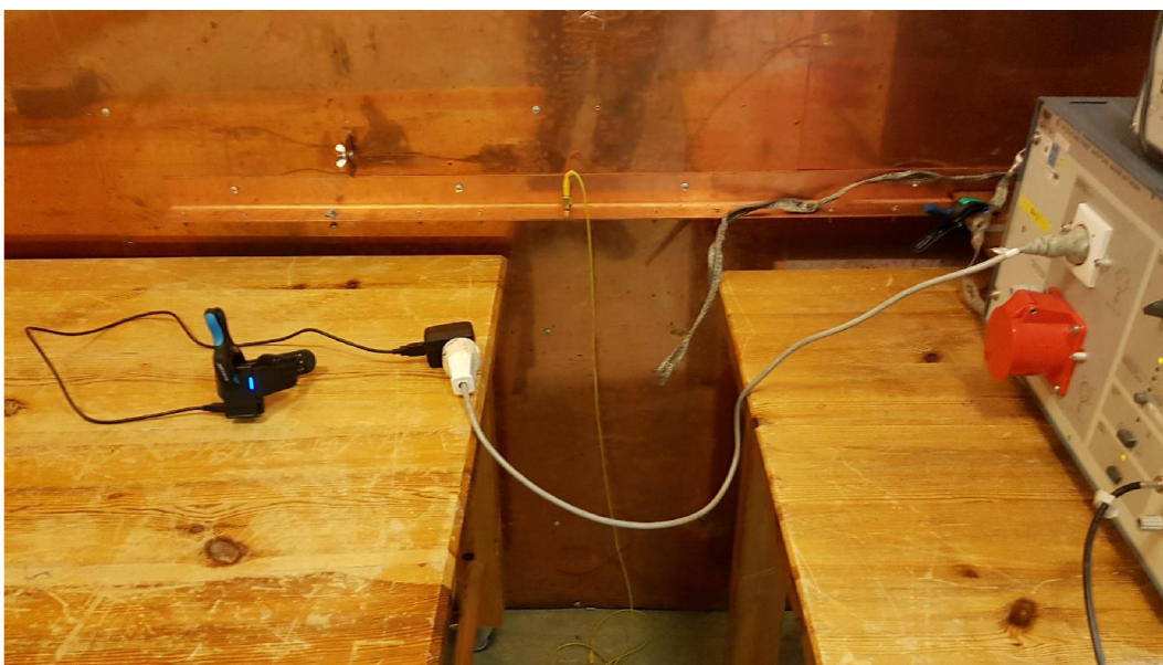
Test set up conducted emission 150 kHz – 30 MHz
