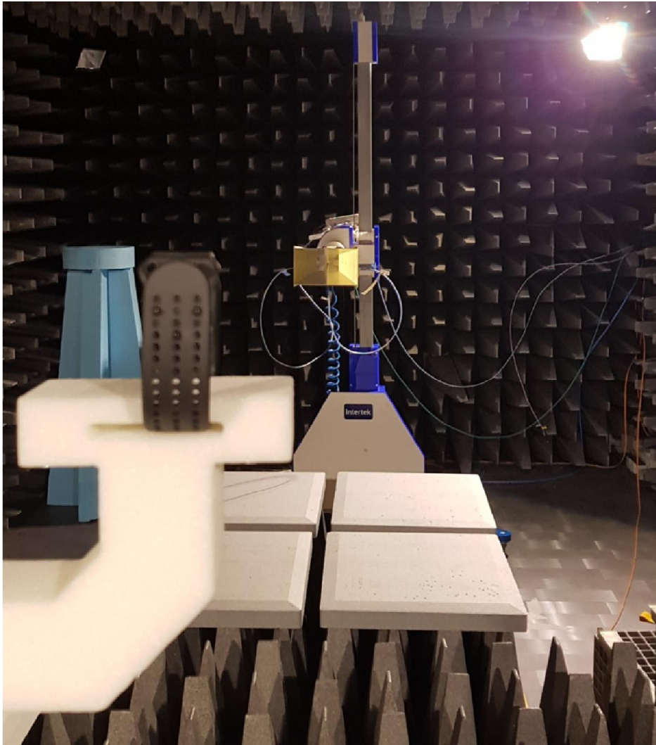
Test set up radiated emission > 1GHz
