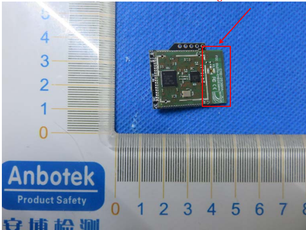
Zigbee Antenna
