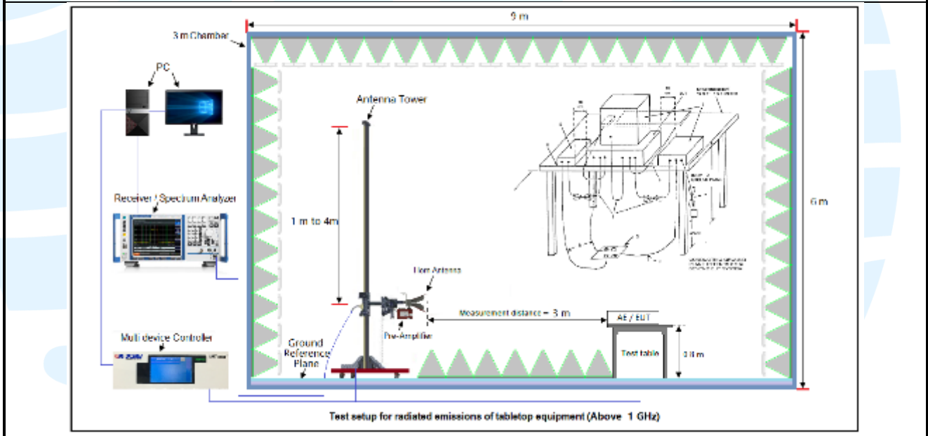
Figure 2. Above 1GHz
