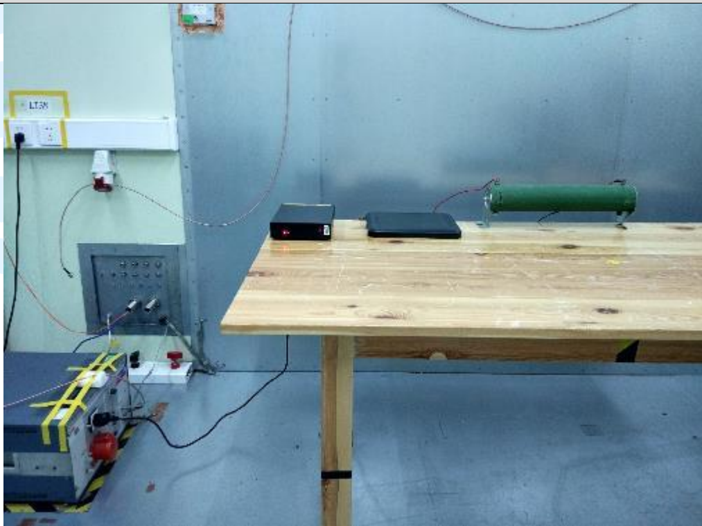
Conducted Emission Test Setu
