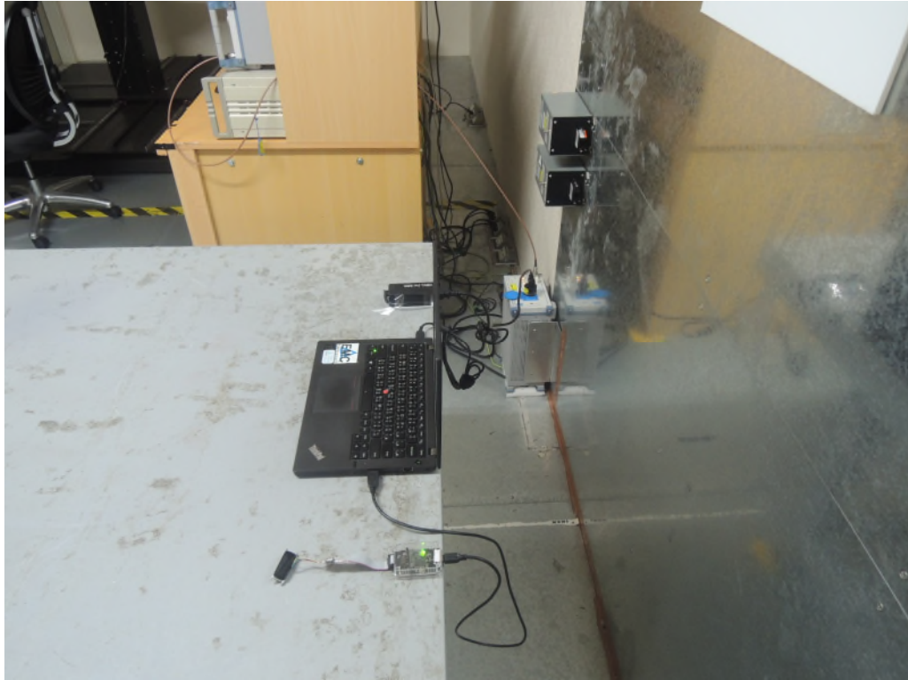
Photograph 10: Set-up for Mains Conducted testing Back
