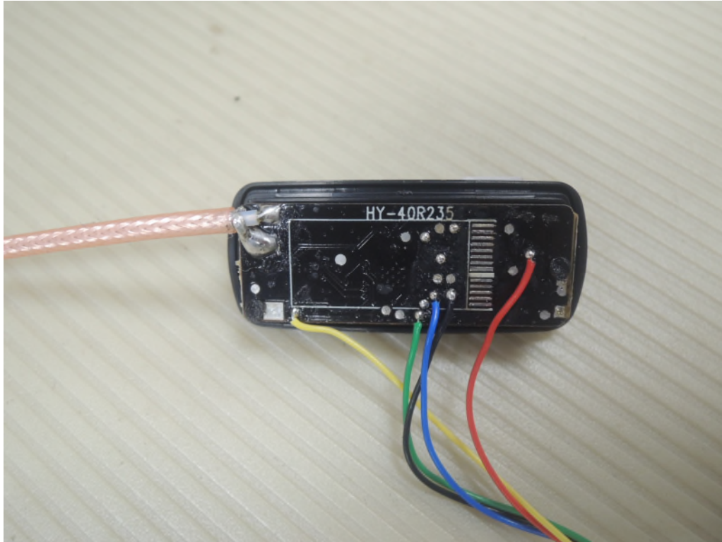
Photograph 9: Set-up for Mains Conducted testing Front
