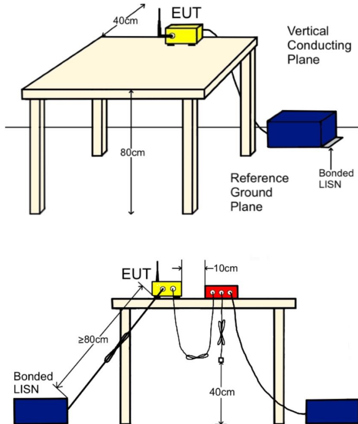
Figure 12: CEV Test Setup
