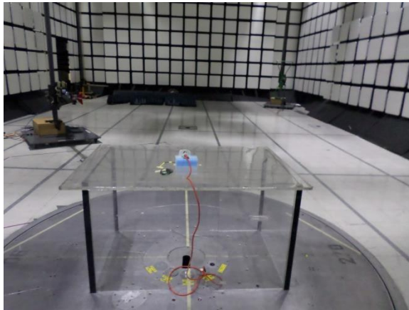
Figure 2: Radiated Spurious Emissions, 30MHz-1000MHz - Setup Rear View
