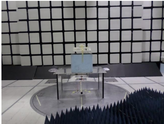
Figure 4: Radiated Spurious Emissions, 1GHz-10GHz - Setup Front View
