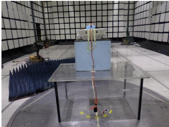
Figure 5: Radiated Spurious Emissions, 1GHz-10GHz - Setup Rear View
