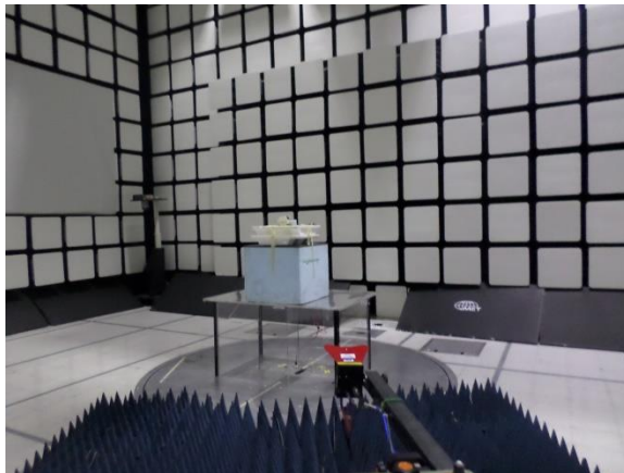
Figure 6: Radiated Spurious Emissions, 1GHz-10GHz - Setup Antenna View
