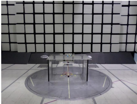
Figure 1: Radiated Spurious Emissions, 30MHz-1000MHz - Setup Front View
