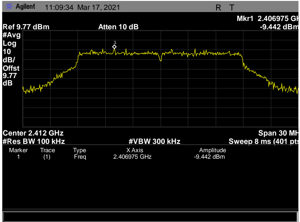
Figure 210: Power Spectral Density, 802.11n_HT20, Average PSD - 2412 MHz
