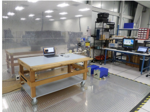
Figure 27: Conducted Emissions, Setup Front View
