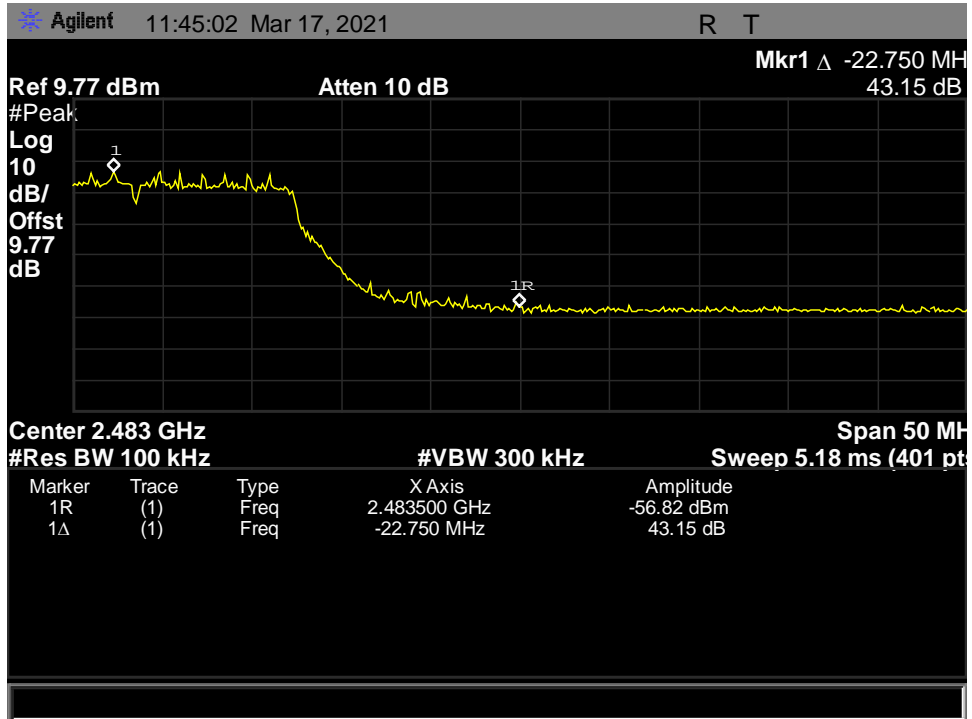
Figure 190: Radiated Band Edge, 802.11n_HT20, High- 2462 MHz
