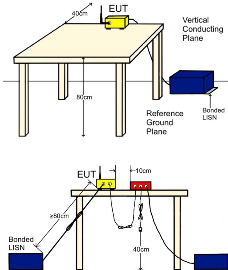
Figure 14: CEV Test Setup
