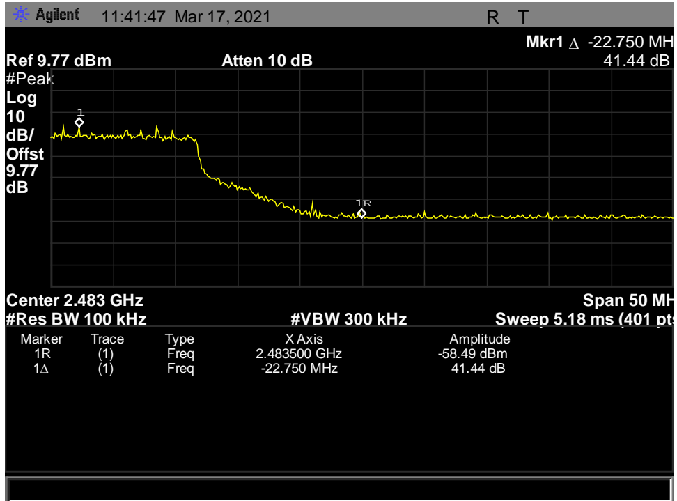
Figure 192: Radiated Band Edge, 802.11n_HT40, High- 2452 MHz
