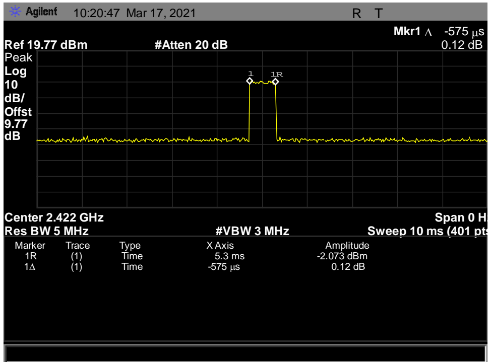
Figure 12: Duty Cycle, 802.11n_HT40, ON-Time
