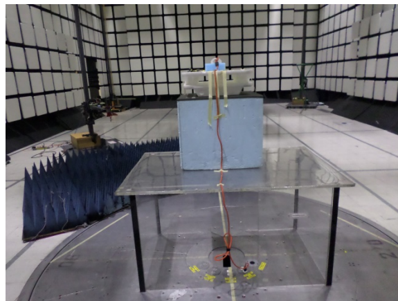
Figure 198: Radiated Spurious Emissions Test Setup, 1GHz-18GHz - Setup Rear View
