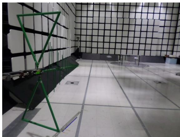
Figure 196: Radiated Spurious Emissions Test Setup, 30MHz-1000MHz - Setup Antenna View
