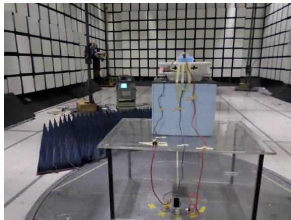
Figure 201: Radiated Spurious Emissions Test Setup, 18GHz-25GHz - Setup Rear View
