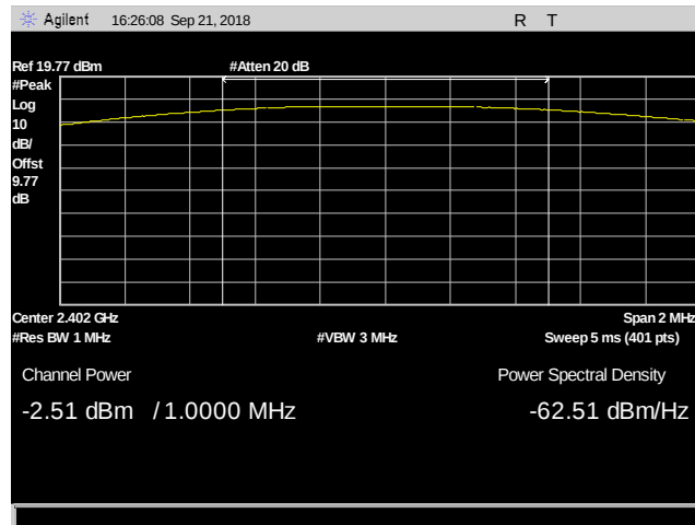
Plot 23. DH1 Peak Power Output, 2402 MHz
