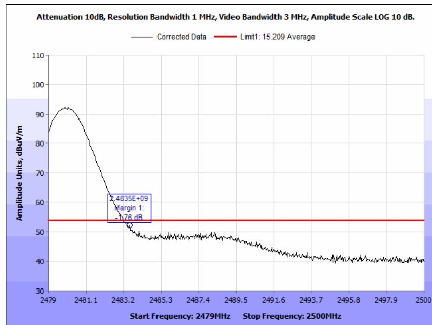
Plot 65. Radiated Restricted Band Edge, 2480 MHz, High, Peak on Average limit
