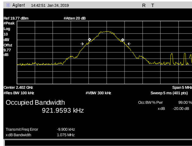
Plot 9. DH5 20 dB Occupied Bandwidth, 2402 MHz
