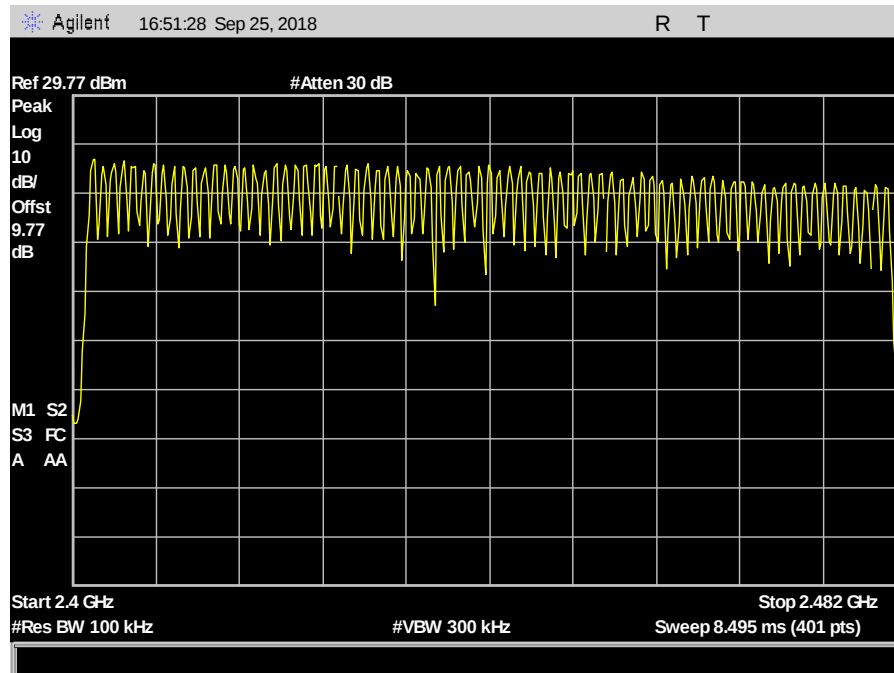
Plot 21. Number of Hopping Channels, 2400 – 2482 MHz, 79
