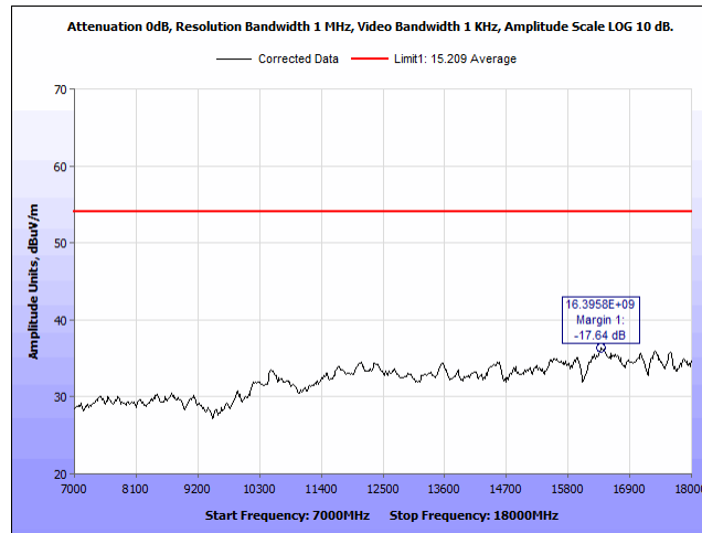
Plot 50. Radiated Spurious Emissions, 2441 MHz, 7 – 18 GHz, V, Average
