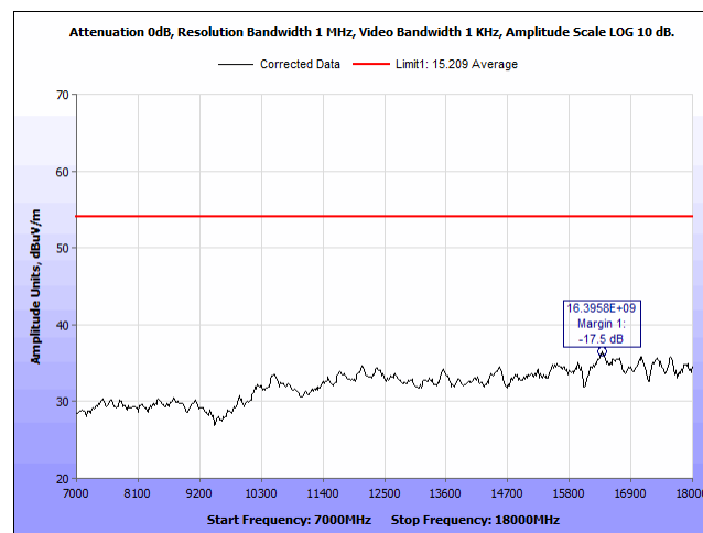
Plot 58. Radiated Spurious Emissions, 2480 MHz, 7 – 18 GHz, H, Average
