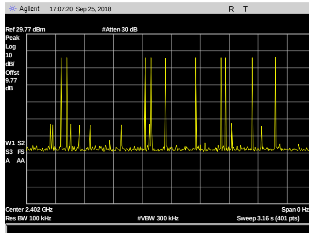
Plot 12. DH1 Dwell Time, 3.16s span, 10 pulses
