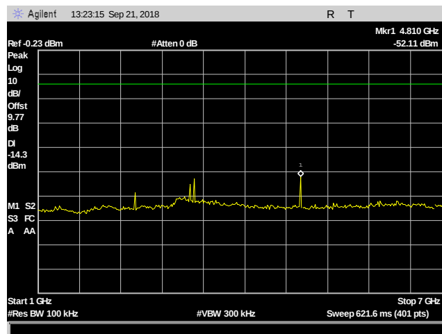
Plot 67. Conducted Spurious Emissions, 2402 MHz, 1 GHz – 7 GHz
