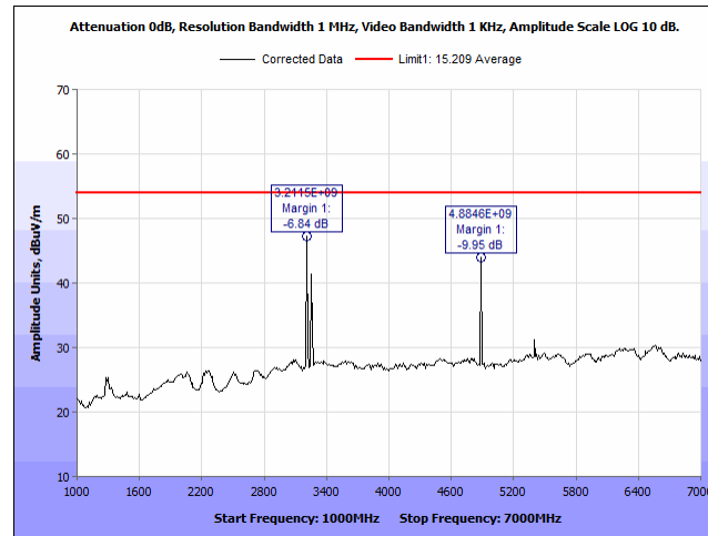
Plot 44. Radiated Spurious Emissions, 2441 MHz, 1 – 7 GHz, H, Average
