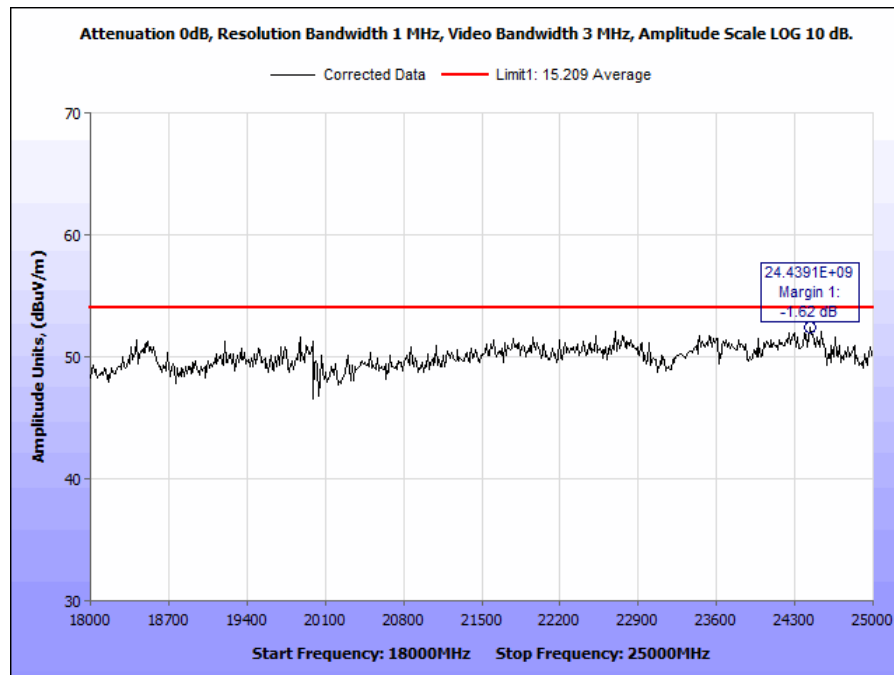
Plot 63. Radiated Spurious Emissions, 18 - 25 GHz, V
