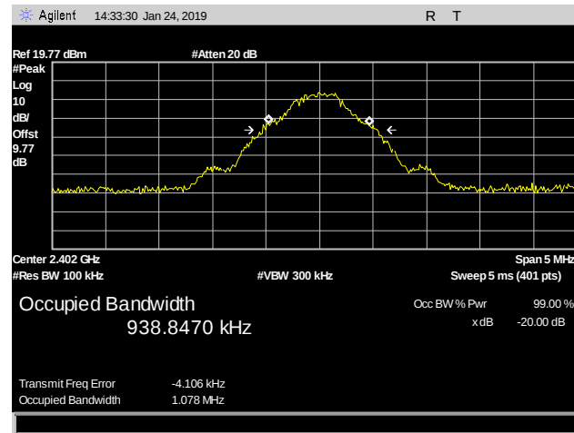
Plot 6. DH3 20 dB Occupied Bandwidth, 2402 MHz
