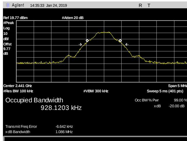
Plot 7. DH3 20 dB Occupied Bandwidth, 2441 MHz
