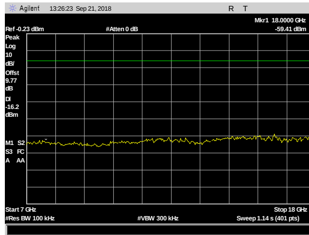
Plot 72. Conducted Spurious Emissions, 2441 MHz, 7 – 18 GHz
