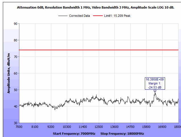
Plot 51. Radiated Spurious Emissions, 2441 MHz, 7 – 18 GHz, V, Peak
