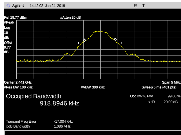
Plot 10. DH5 20 dB Occupied Bandwidth, 2441 MHz
