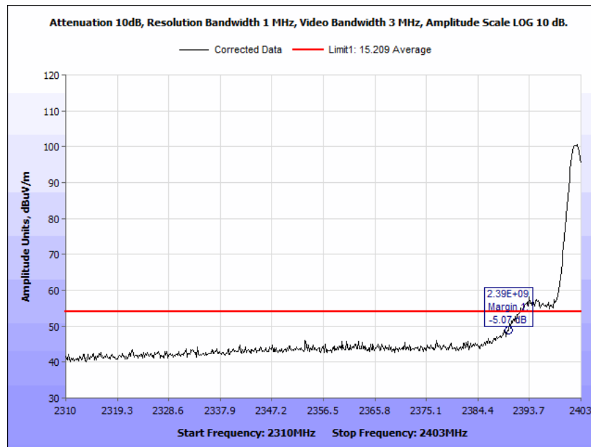
Plot 64. Radiated Restricted Band Edge, 2402 MHz, Low, Peak on Average limit
