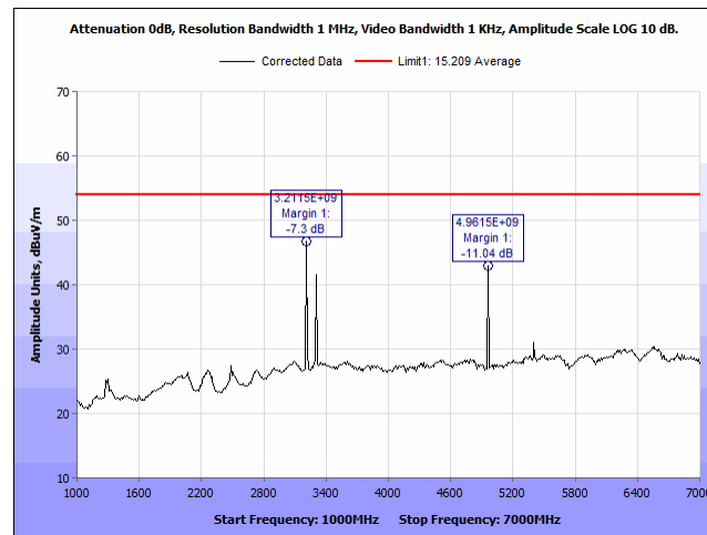
Plot 54. Radiated Spurious Emissions, 2480 MHz, 1 – 7 GHz, H, Average
