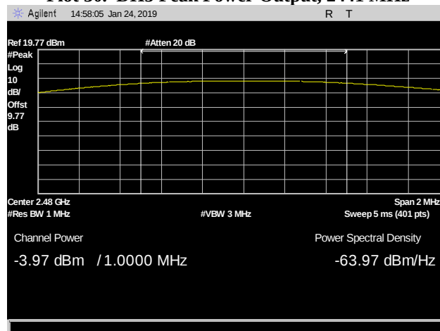
Plot 31. DH5 Peak Power Output, 2480 MHz
