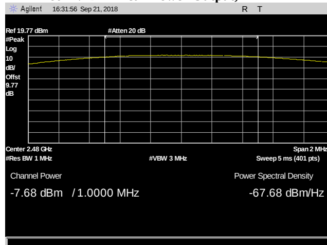
Plot 25. DH1 Peak Power Output, 2480 MHz
