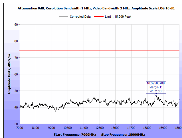
Plot 61. Radiated Spurious Emissions, 2480 MHz, 7 – 18 GHz, V, Peak
