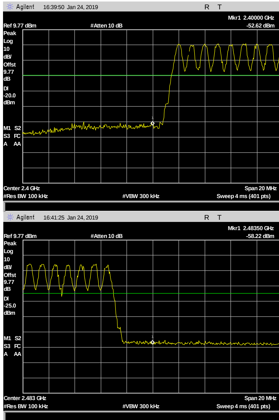
Plot 81. Conducted Bandedge, DH3 Hopping
