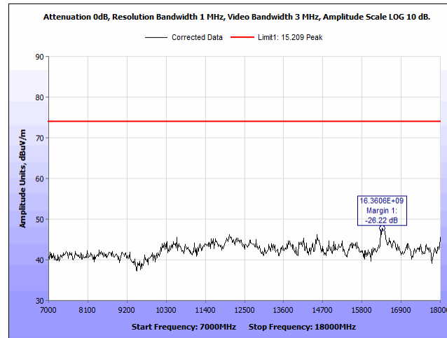
Plot 59. Radiated Spurious Emissions, 2480 MHz, 7 – 18 GHz, H, Peak
