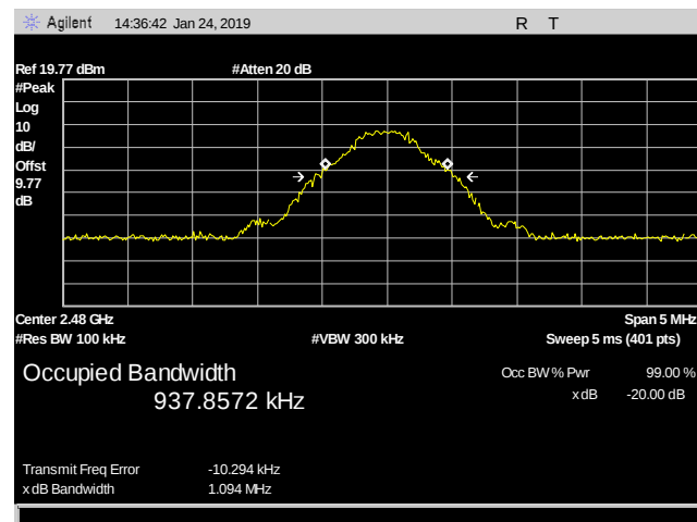
Plot 8. DH3 20 dB Occupied Bandwidth, 2480 MHz
