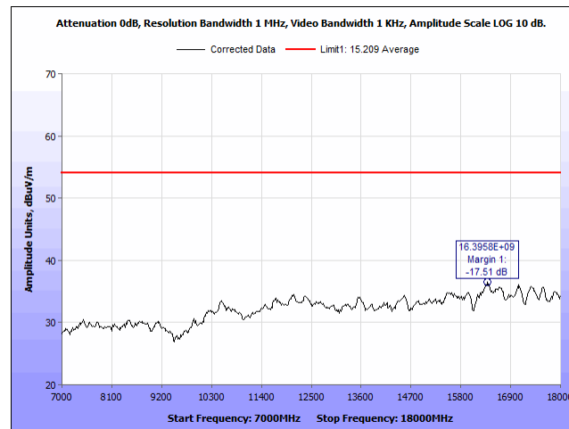
Plot 48. Radiated Spurious Emissions, 2441 MHz, 7 – 18 GHz, H, Average
