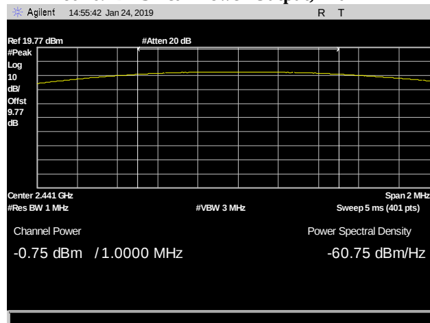
Plot 27. DH3 Peak Power Output, 2441 MHz
