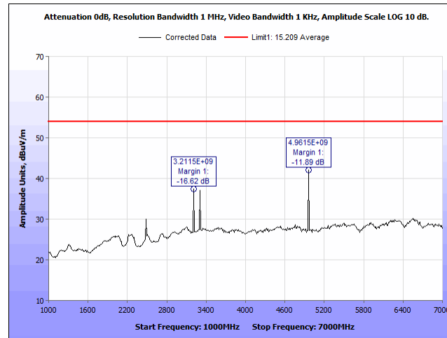
Plot 56. Radiated Spurious Emissions, 2480 MHz, 1 – 7 GHz, V, Average
