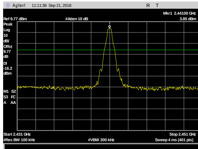
Plot 73. Conducted Spurious Emissions, 2441 MHz, Reference
