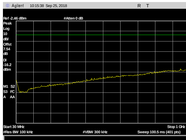
Plot 70. Conducted Spurious Emissions, 2441 MHz, 30 MHz – 1 GHz
