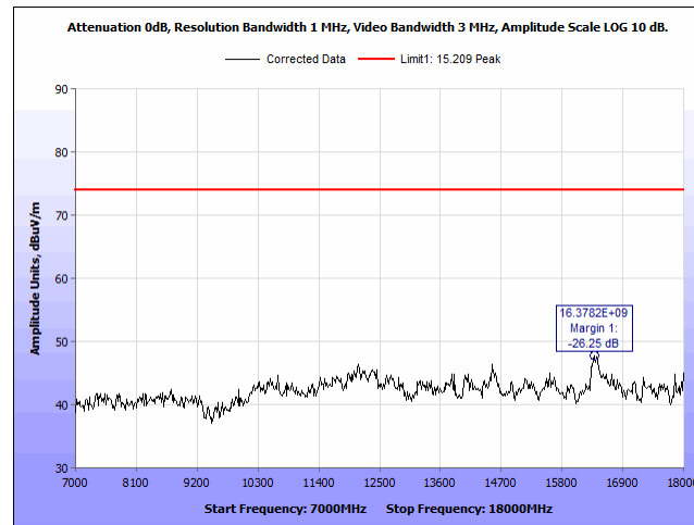
Plot 41. Radiated Spurious Emissions, 2402 MHz, 7 – 18 GHz, V, Peak
