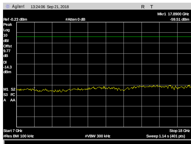
Plot 68. Conducted Spurious Emissions, 2402 MHz, 7 – 18 GHz
