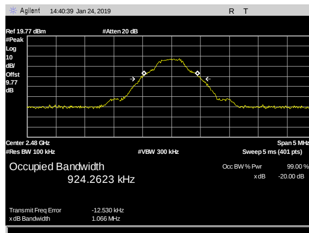
Plot 11. DH5 20 dB Occupied Bandwidth, 2480 MHz
