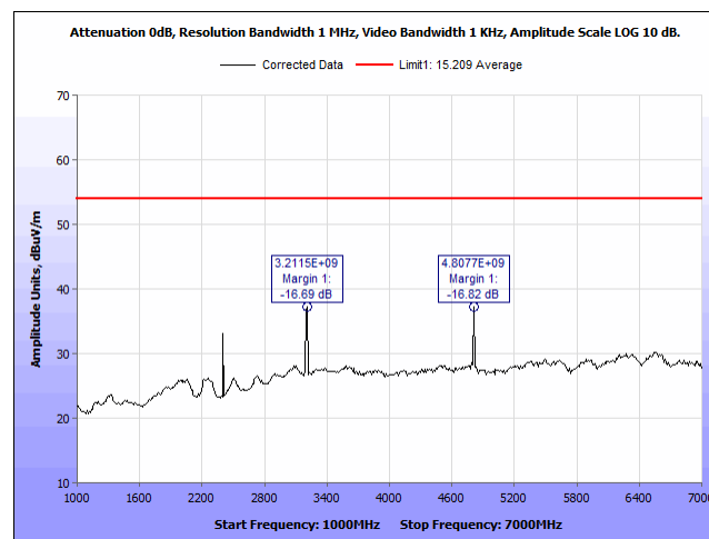
Plot 36. Radiated Spurious Emissions, 2402 MHz 1 – 7 GHz, V, Average
