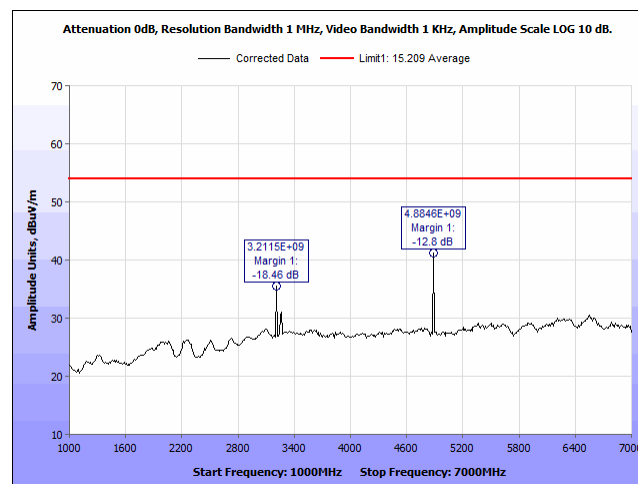
Plot 46. Radiated Spurious Emissions, 2441 MHz, 1 – 7 GHz, V, Average
