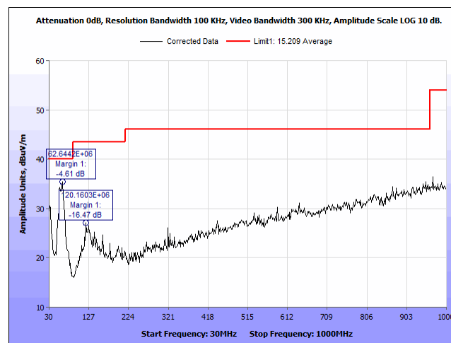
Plot 33. Radiated Spurious Emissions, 2402 MHz, 30 MHz – 1 GHz, V
