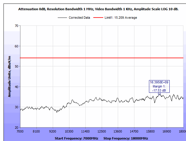
Plot 40. Radiated Spurious Emissions, 2402 MHz, 7 – 18 GHz, V, Average
