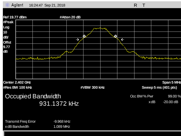
Plot 3. DH1 20 dB Occupied Bandwidth, 2402 MHz
