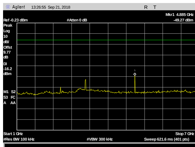
Plot 71. Conducted Spurious Emissions, 2441 MHz, 1 GHz – 7 GHz
