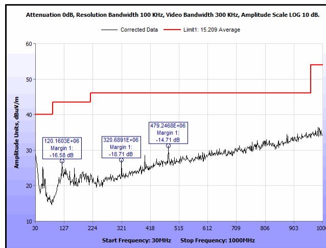
Plot 42. Radiated Spurious Emissions, 2441 MHz, 30 MHz – 1 GHz, H
