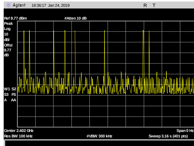
Plot 15. DH3 Dwell Time, 3.16s span, 8 pulses
