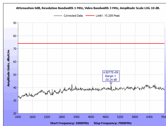
Plot 37. Radiated Spurious Emissions, 2402 MHz, 1 – 7 GHz, V, Peak
