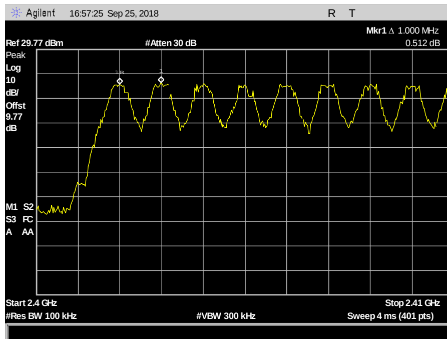
Plot 22. Channel Separation, 1 MHz
