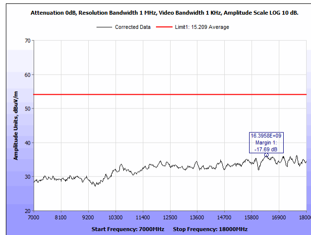
Plot 60. Radiated Spurious Emissions, 2480 MHz, 7 – 18 GHz, V, Average
