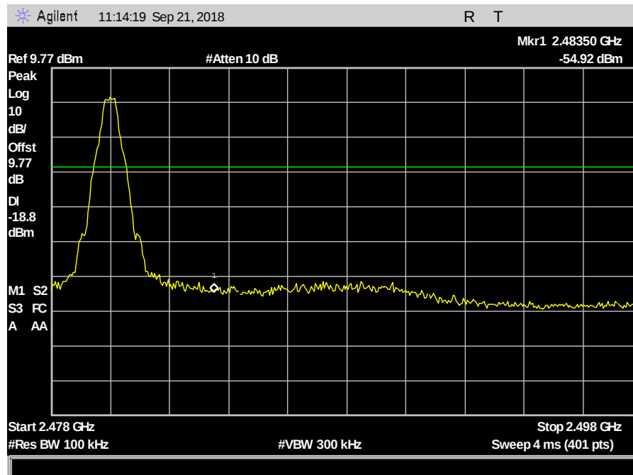
Plot 79. Conducted Band Edge, 2480 MHz, High
