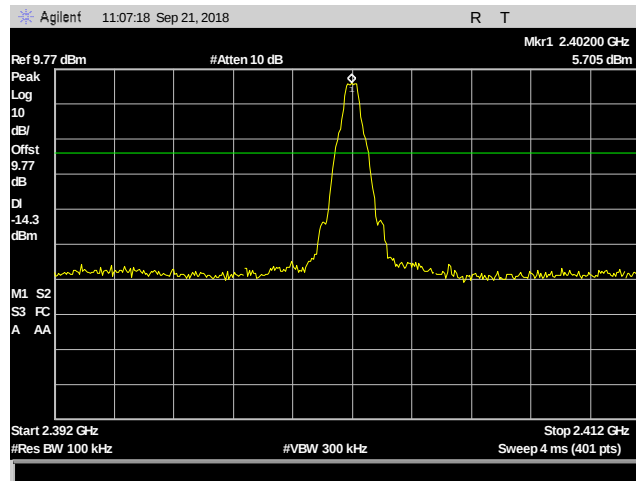
Plot 69. Conducted Spurious Emissions, 2402 MHz, Reference
