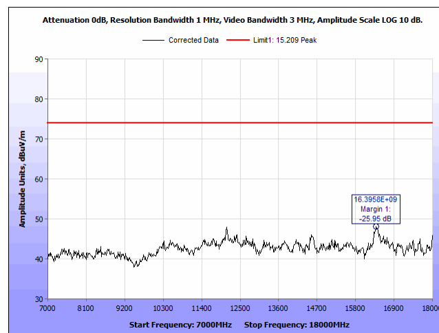
Plot 49. Radiated Spurious Emissions, 2441 MHz, 7 – 18 GHz, H, Peak
