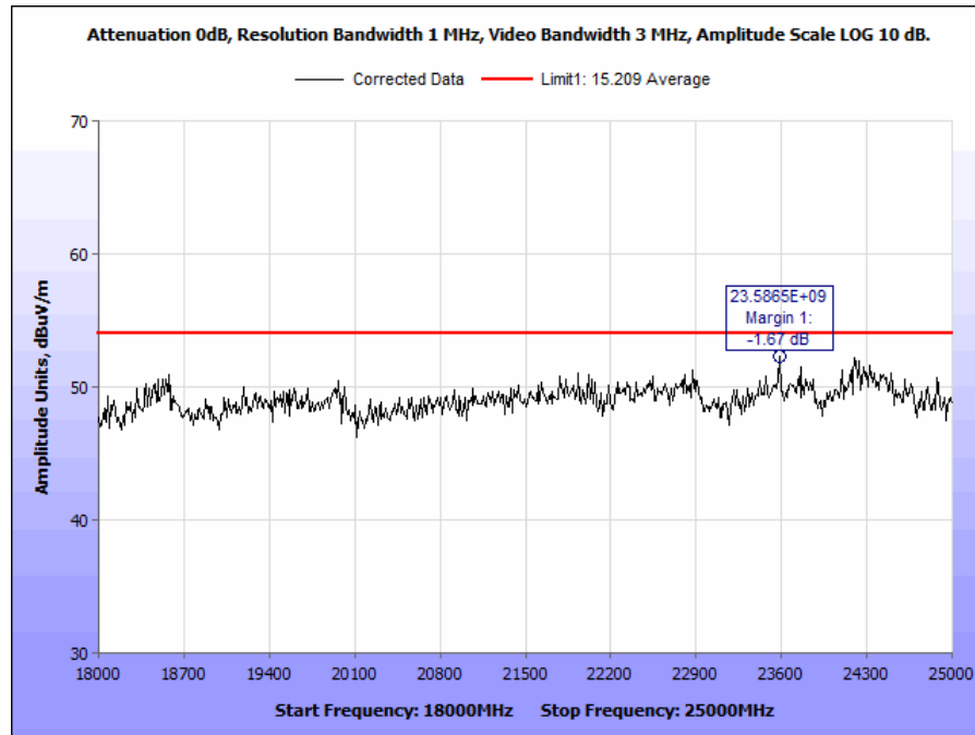
Plot 62. Radiated Spurious Emissions, 18 - 25 GHz, H
