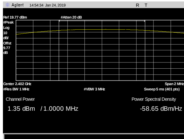
Plot 26. DH3 Peak Power Output, 2402 MHz
