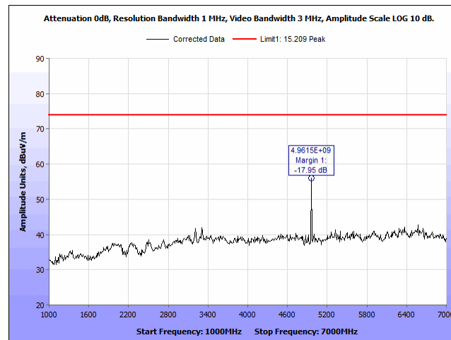
Plot 57. Radiated Spurious Emissions, 2480 MHz, 1 – 7 GHz, V, Peak
