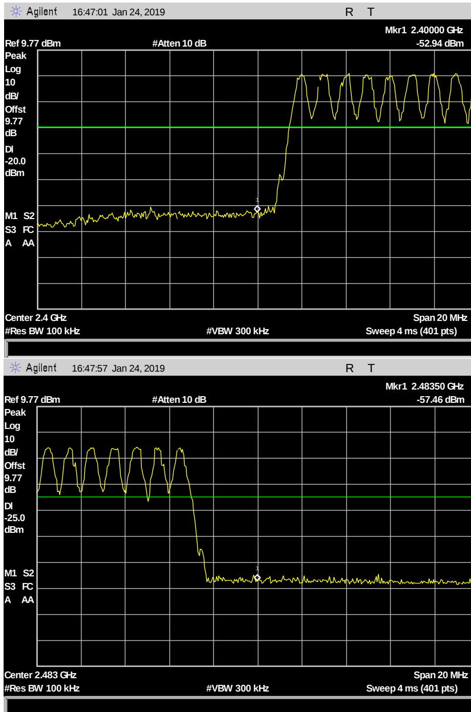
Plot 82. Conducted Bandedge, DH5 Hopping
