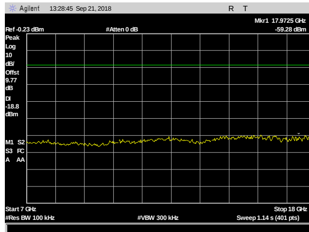
Plot 76. Conducted Spurious Emissions, 2480 MHz, 7 – 18 GHz
