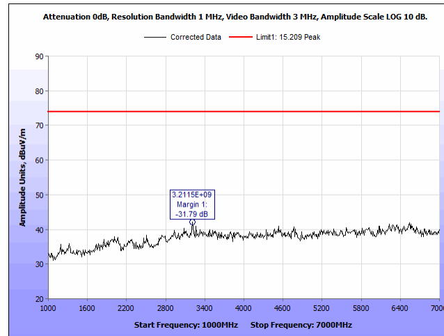
Plot 47. Radiated Spurious Emissions, 2441 MHz, 1 – 7 GHz, V, Peak
