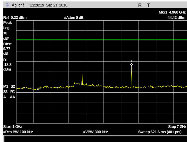
Plot 75. Conducted Spurious Emissions, 2480 MHz, 1 GHz – 7 GHz
