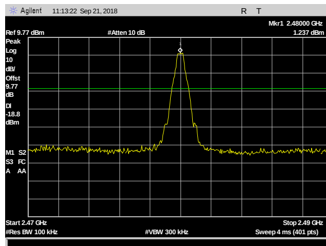
Plot 77. Conducted Spurious Emissions, 2480 MHz, Reference
