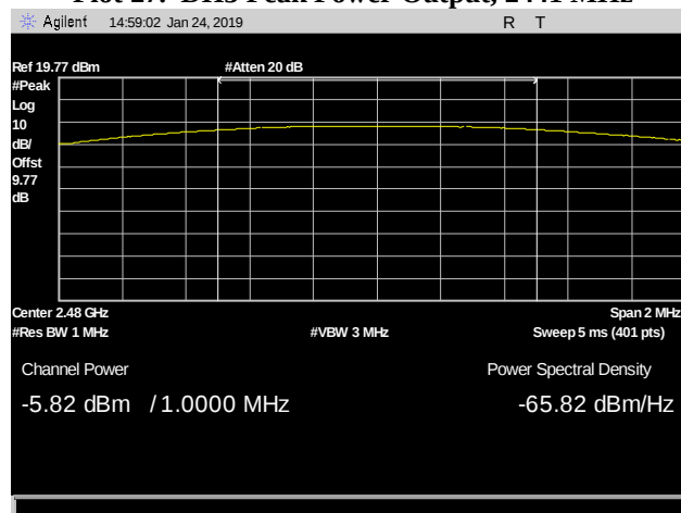
Plot 28. DH3 Peak Power Output, 2480 MHz
