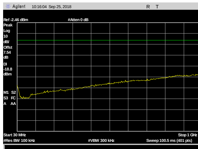
Plot 74. Conducted Spurious Emissions, 2480 MHz, 30 MHz – 1 GHz
