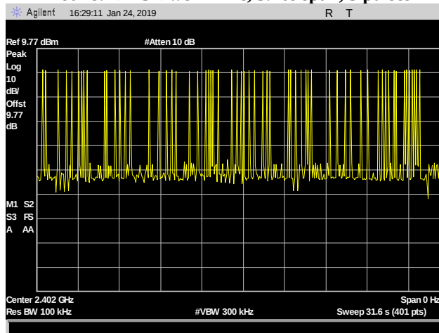
Plot 19. DH5 Dwell Time, 31.6s span
