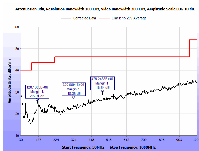
Plot 52. Radiated Spurious Emissions, 2480 MHz, 30 MHz – 1 GHz, H
