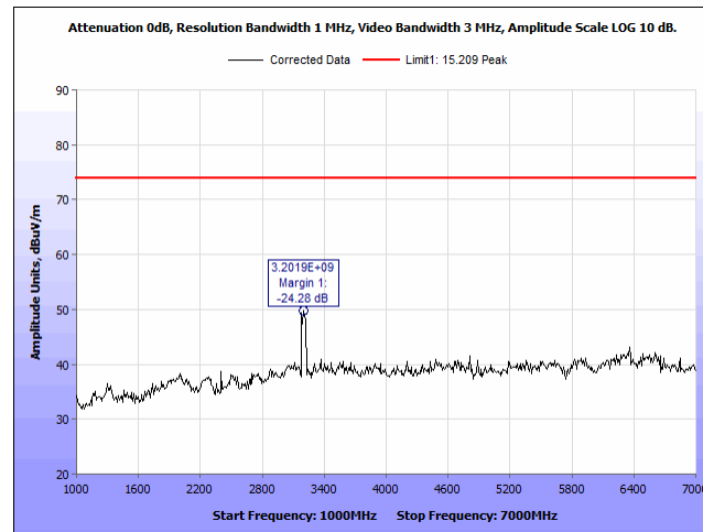
Plot 35. Radiated Spurious Emissions, 2402 MHz, 1 – 7 GHz, H, Peak
