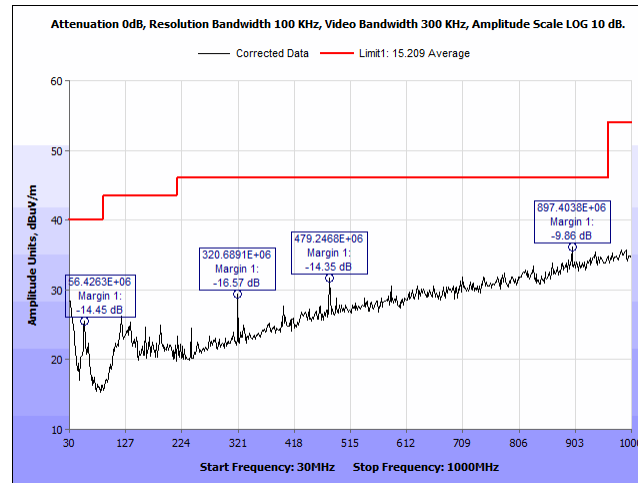
Plot 32. Radiated Spurious Emissions, 2402 MHz, 30 MHz – 1 GHz, H
