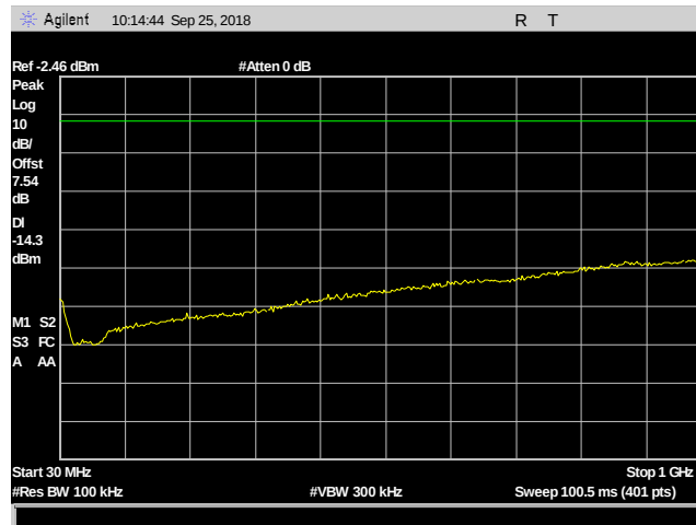
Plot 66. Conducted Spurious Emissions, 2402 MHz, 30 MHz – 1 GHz
