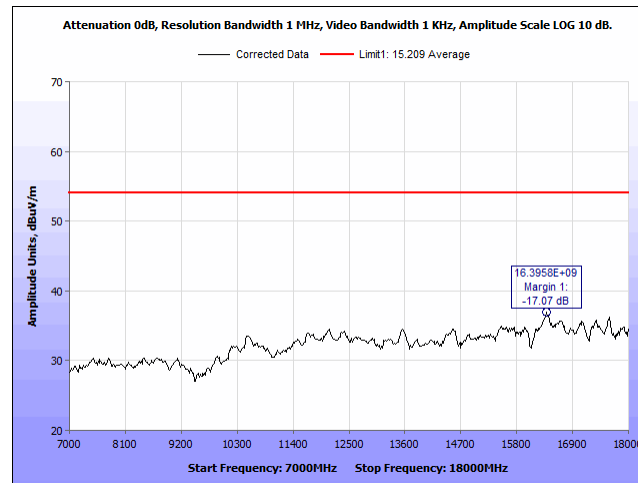
Plot 38. Radiated Spurious Emissions, 2402 MHz, 7 – 18 GHz, H, Average
