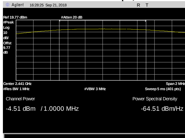
Plot 24. DH1 Peak Power Output, 2441 MHz
