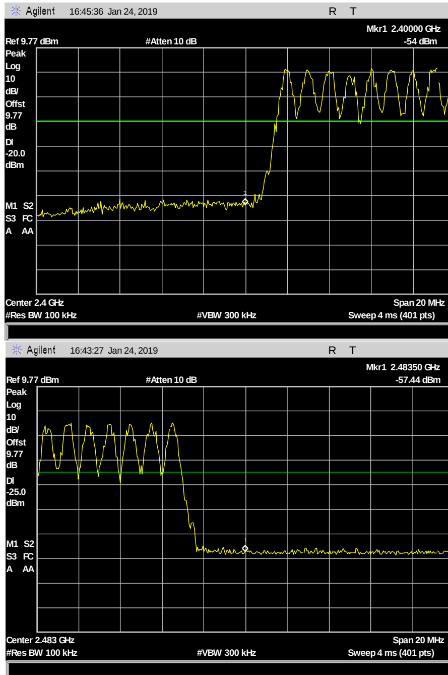
Plot 80. Conducted Bandedge, DH1 Hopping
