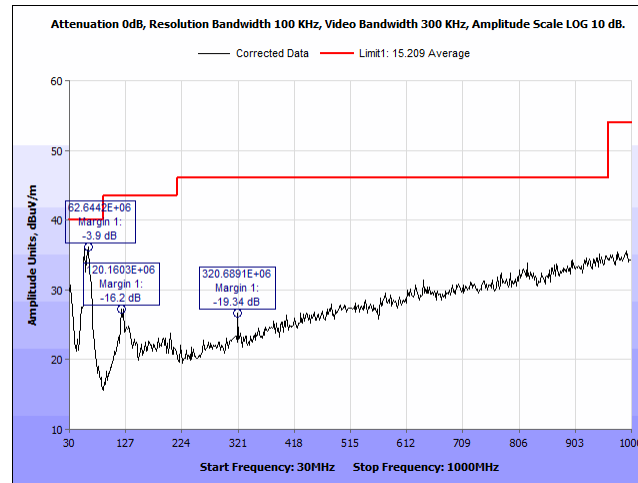
Plot 53. Radiated Spurious Emissions, 2480 MHz, 30 MHz – 1 GHz, V
