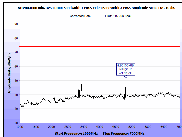
Plot 55. Radiated Spurious Emissions, 2480 MHz, 1 – 7 GHz, H, Peak
