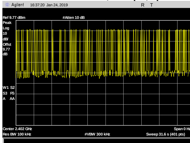
Plot 16. DH3 Dwell Time, 31.6s span
