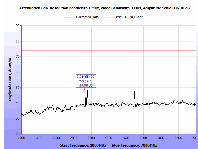
Plot 45. Radiated Spurious Emissions, 2441 MHz, 1 – 7 GHz, H, Peak
