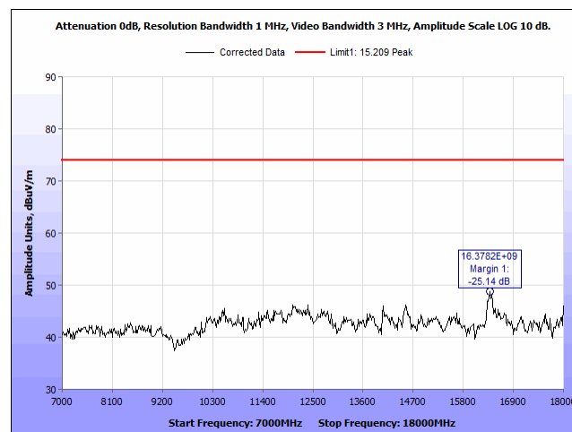
Plot 39. Radiated Spurious Emissions, 2402 MHz, 7 – 18GHz, H, Peak
