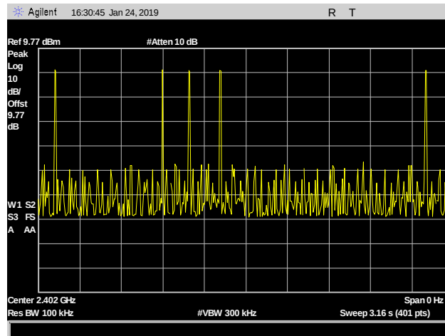
Plot 18. DH5 Dwell Time, 3.16s span, 5 pulses
