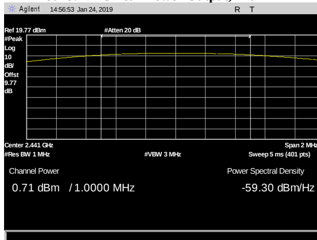
Plot 30. DH5 Peak Power Output, 2441 MHz
