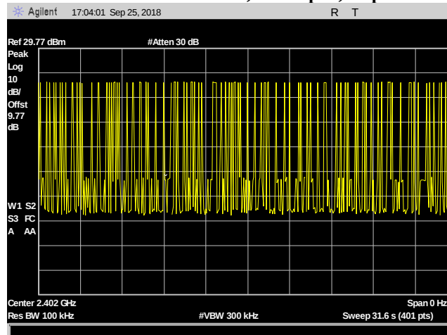
Plot 13. DH1 Dwell Time, 31.6s span
