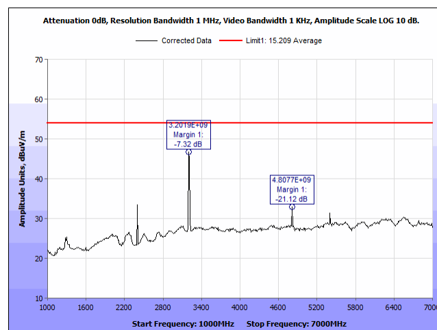
Plot 34. Radiated Spurious Emissions, 2402 MHz, 1 – 7 GHz, H, Average
