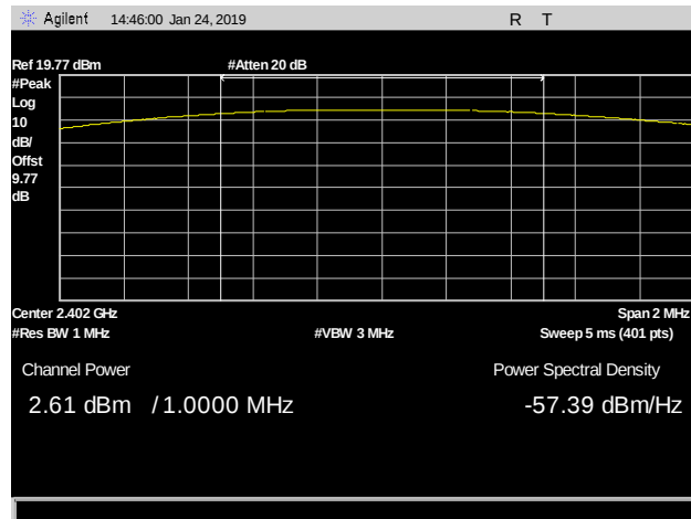
Plot 29. DH5 Peak Power Output, 2402 MHz
