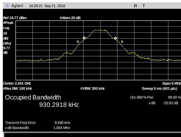
Plot 4. DH1 20 dB Occupied Bandwidth, 2441 MHz
