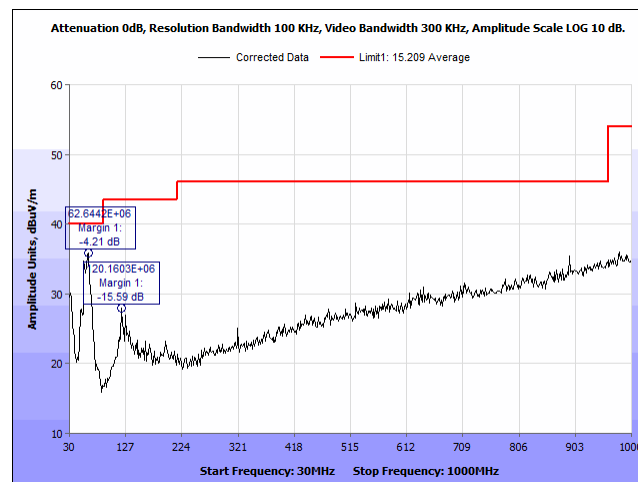
Plot 43. Radiated Spurious Emissions, 2441 MHz, 30 MHz – 1 GHz, V
