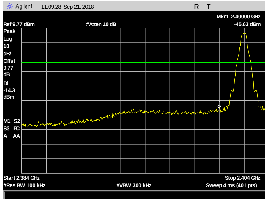
Plot 78. Conducted Band Edge, 2402 MHz, Low
