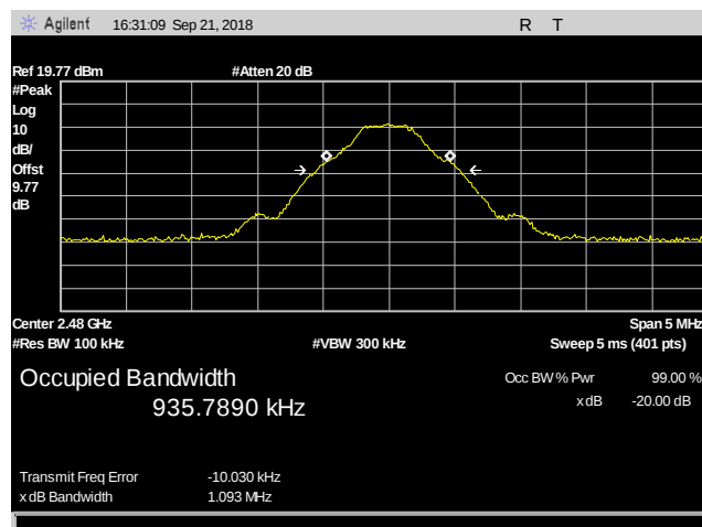
Plot 5. DH1 20 dB Occupied Bandwidth, 2480 MHz
