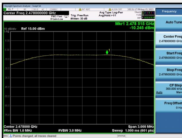
GFSK HIGHCHANNEL
