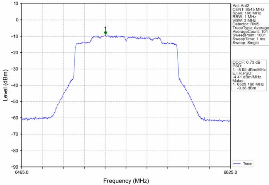
802.11ax(HEW80)_HCH_6545MHz_RU996_Left_MIMO_NTNV
