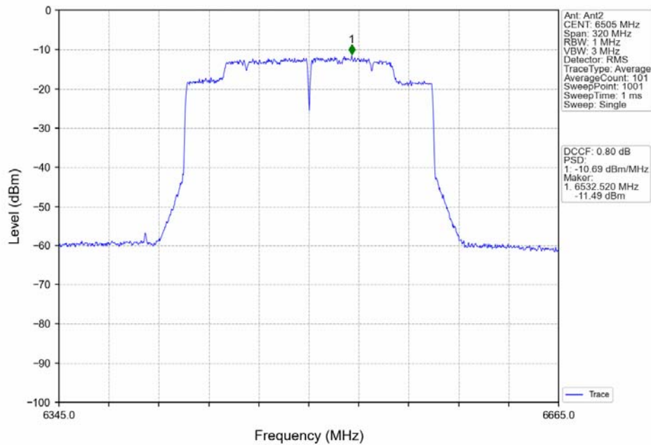
802.11ax(HEW160)_HCH_6505MHz_2xRU996_Left_Ant2_NTNV
