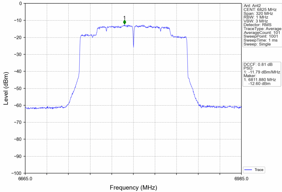
802.11ax(HEW160)_HCH_6825MHz_2xRU996_Left_MIMO_NTNV
