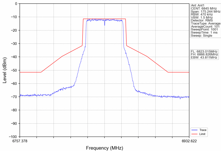
802.11ax(HEW40)_HCH_6845MHz_RU484_Left_Ant1_NTNV
