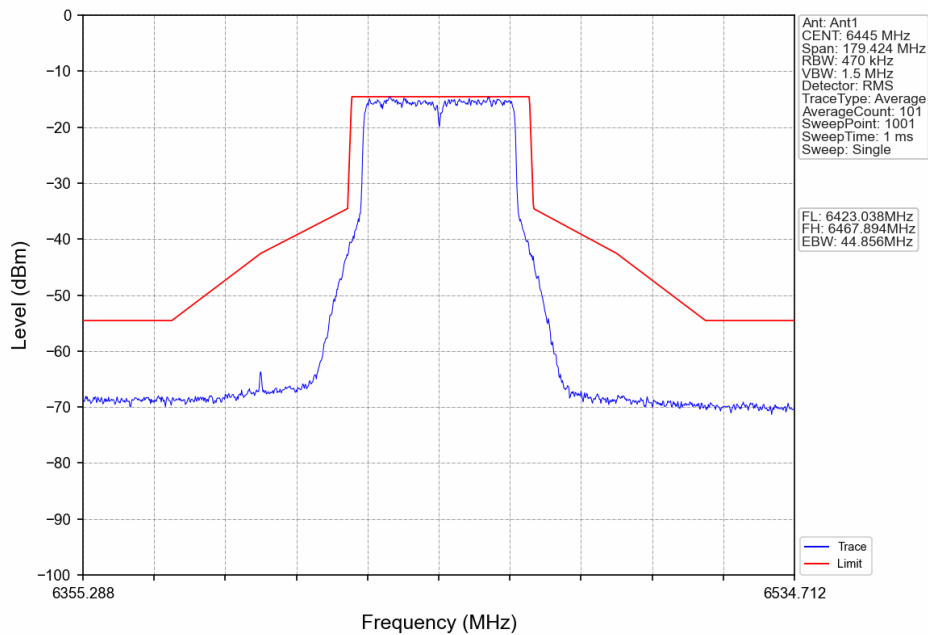
802.11ax(HEW40)_LCH_6445MHz_RU484_Left_Ant1_NTNV
