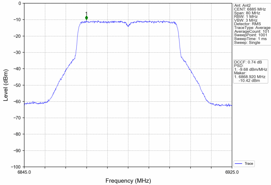
802.11ax(HEW40)_HCH_6885MHz_RU484_Left_MIMO_NTNV
