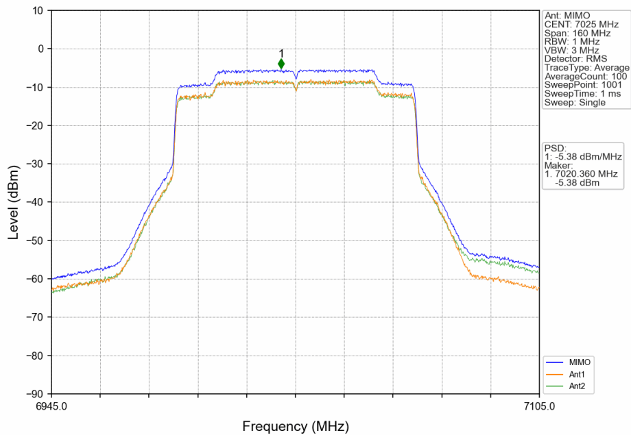
802.11ax(HEW80)_HCH_7025MHz_RU996_Left_MIMO_NTNV
