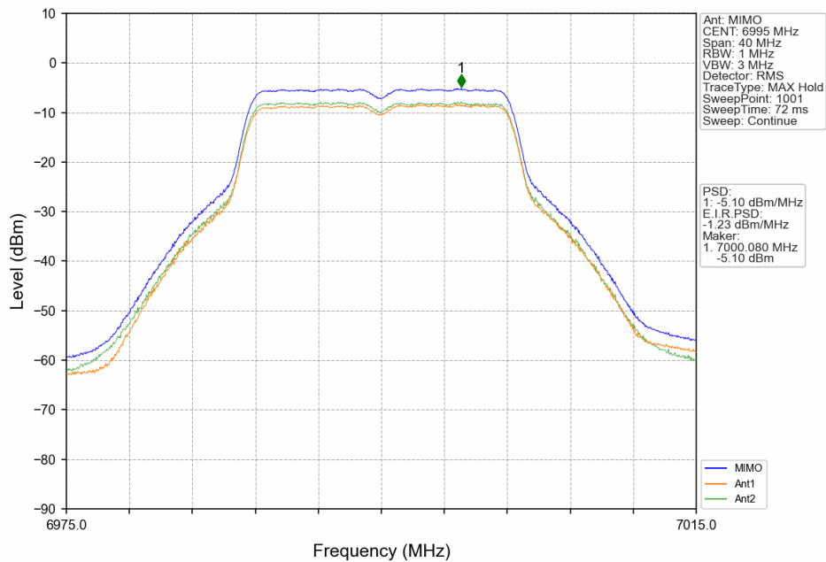
802.11ax(HEW20)_MCH_6995MHz_RU242_Left_MIMO_NTNV
