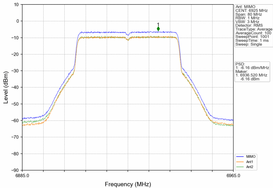
802.11ax(HEW40)_LCH_6925MHz_RU484_Left_MIMO_NTNV
