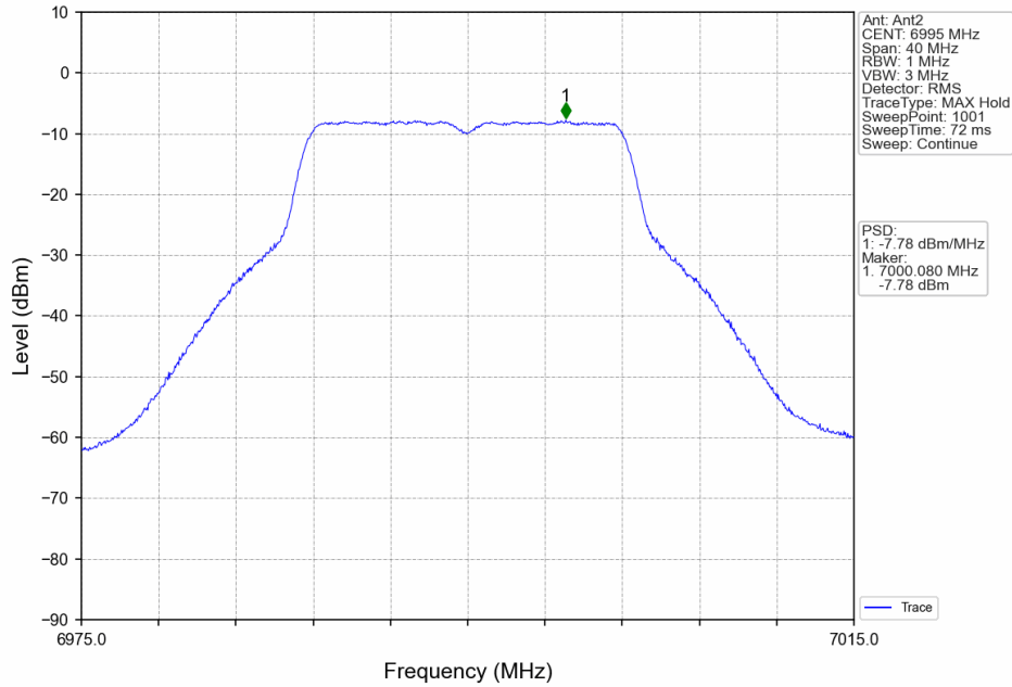
802.11ax(HEW20)_MCH_6995MHz_RU242_Left_MIMO_NTNV
