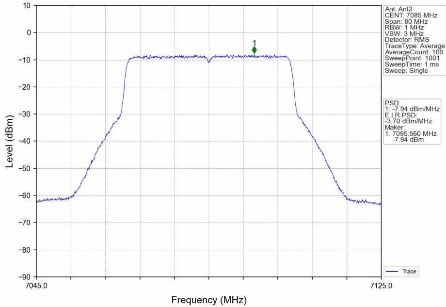
802.11ax(HEW40)_HCH_7085MHz_RU484_Left_MIMO_NTNV
