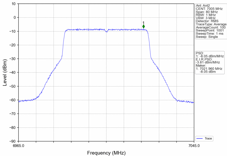
802.11ax(HEW40)_MCH_7005MHz_RU484_Left_Ant2_NTNV
