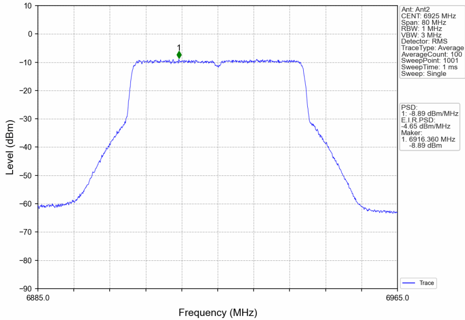
802.11ax(HEW40)_LCH_6925MHz_RU484_Left_MIMO_NTNV
