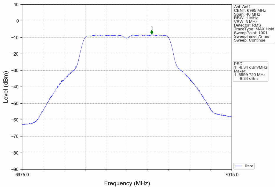
802.11ax(HEW20)_MCH_6995MHz_RU242_Left_Ant1_NTNV
