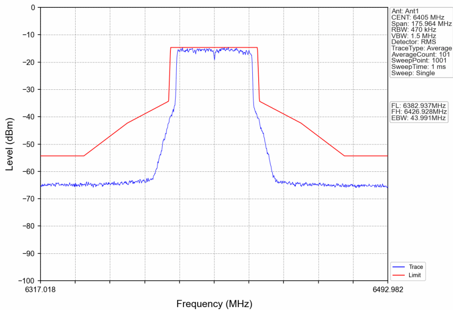
802.11ax(HEW40)_HCH_6405MHz_RU484_Left_Ant1_NTNV
