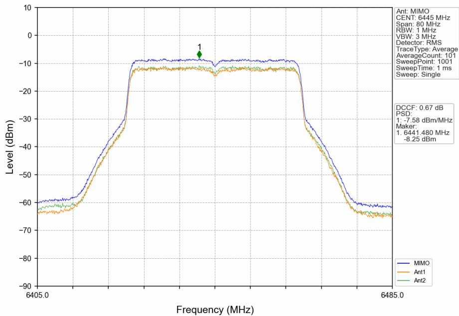
802.11ax(HEW40)_LCH_6445MHz_RU484_Left_MIMO_NTNV
