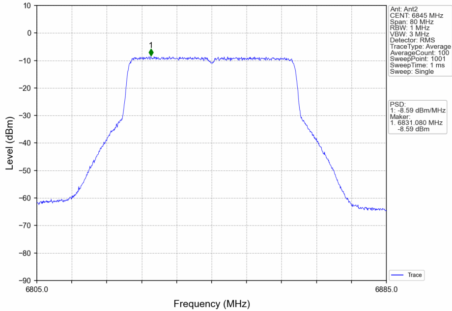
802.11ax(HEW40)_HCH_6845MHz_RU484_Left_MIMO_NTNV
