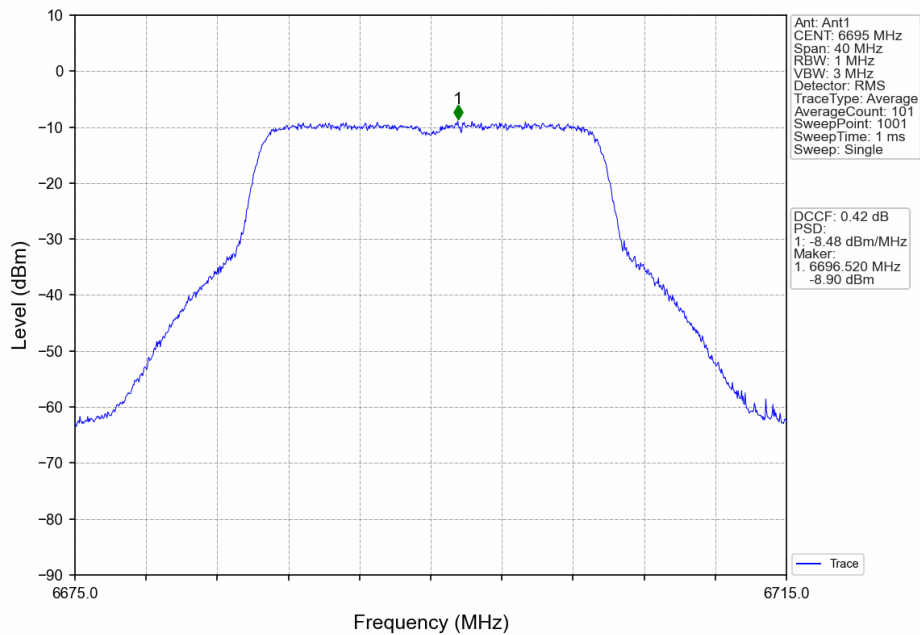
802.11ax(HEW20)_MCH_6695MHz_RU242_Left_Ant1_NTNV
