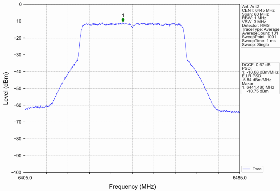
802.11ax(HEW40)_LCH_6445MHz_RU484_Left_MIMO_NTNV
