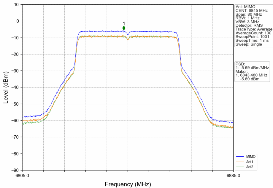
802.11ax(HEW40)_HCH_6845MHz_RU484_Left_MIMO_NTNV
