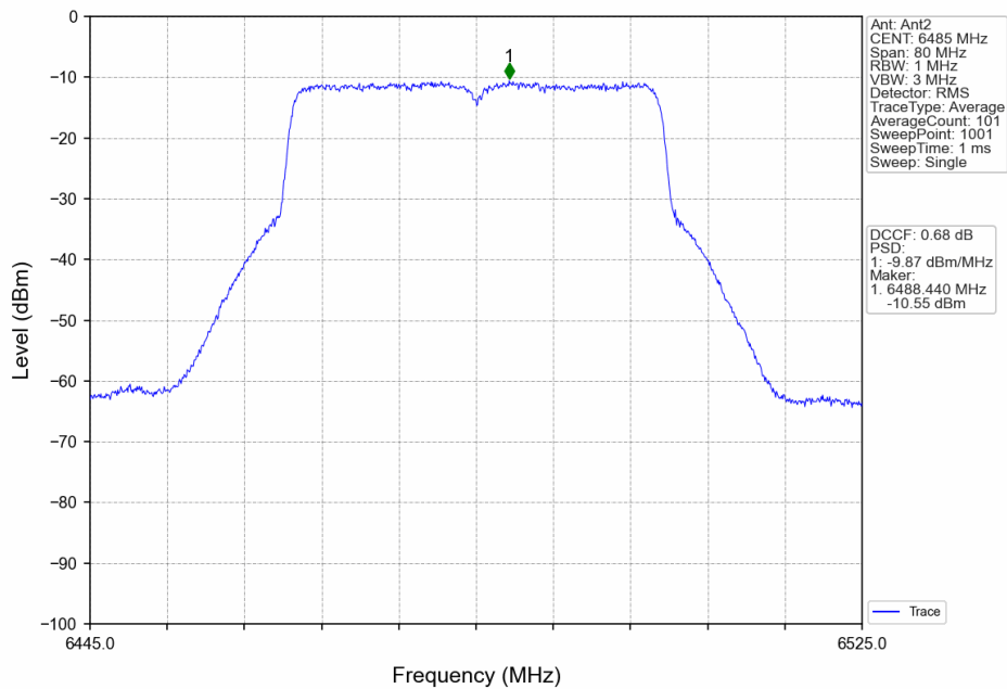
802.11ax(HEW40)_MCH_6485MHz_RU484_Left_Ant2_NTNV
