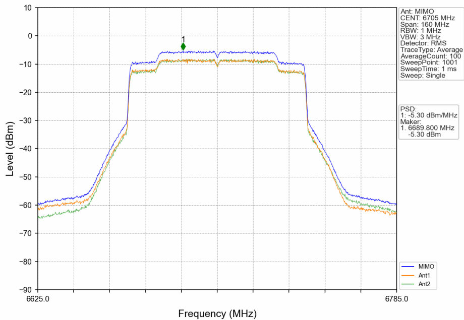
802.11ax(HEW80)_MCH_6705MHz_RU996_Left_MIMO_NTNV
