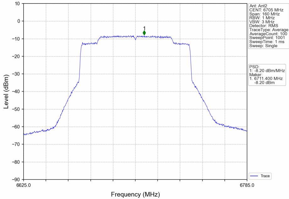
802.11ax(HEW80)_MCH_6705MHz_RU996_Left_MIMO_NTNV
