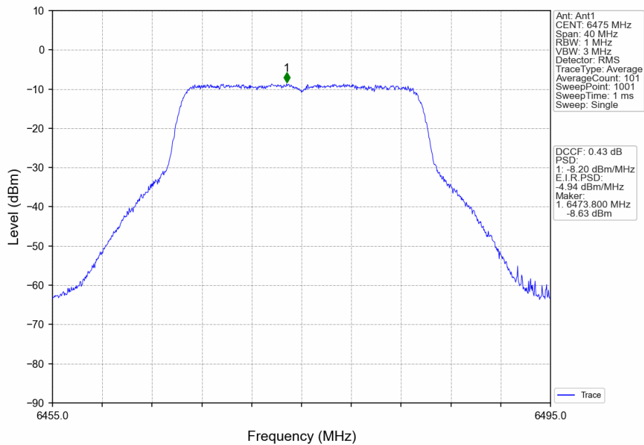
802.11ax(HEW20)_MCH_6475MHz_RU242_Left_Ant1_NTNV
