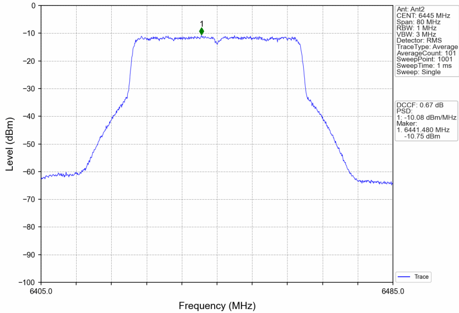
802.11ax(HEW40)_LCH_6445MHz_RU484_Left_MIMO_NTNV
