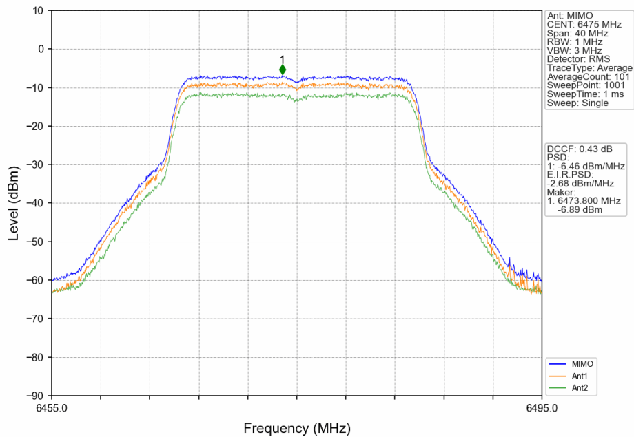
802.11ax(HEW20)_MCH_6475MHz_RU242_Left_MIMO_NTNV
