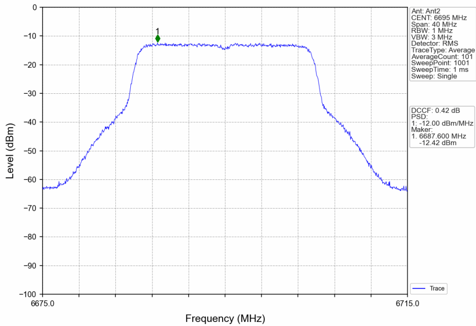
802.11ax(HEW20)_MCH_6695MHz_RU242_Left_MIMO_NTNV
