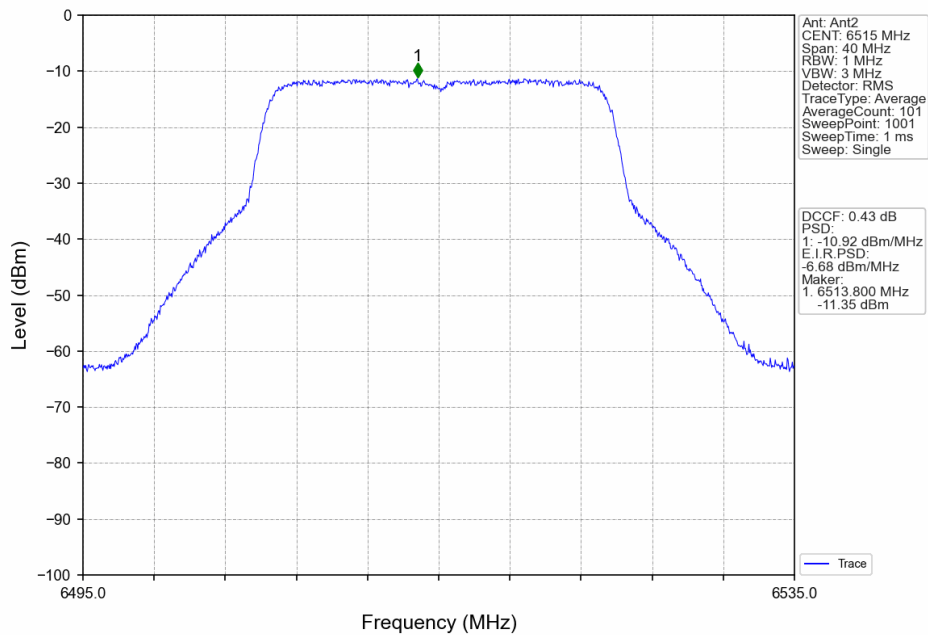
802.11ax(HEW20)_HCH_6515MHz_RU242_Left_Ant2_NTNV
