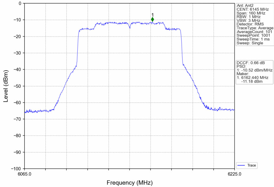
802.11ax(HEW80)_MCH_6145MHz_RU996_Left_MIMO_NTNV
