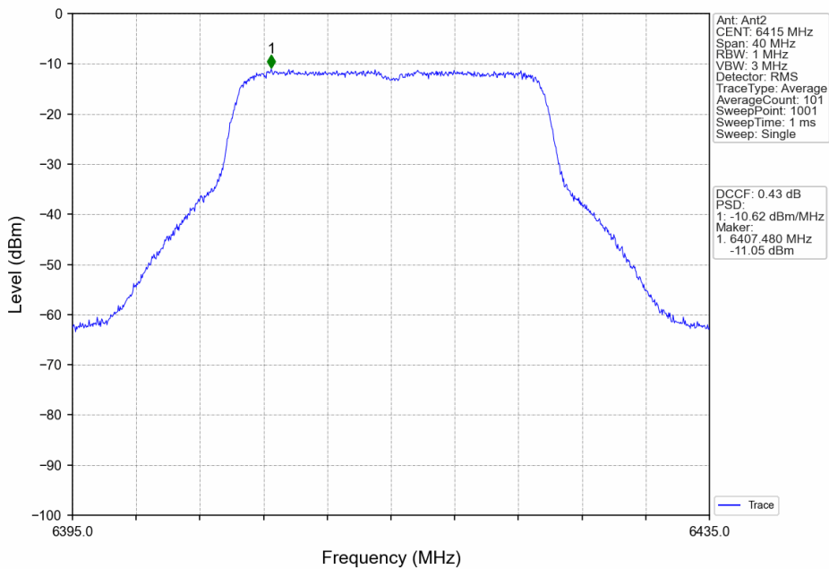
802.11ax(HEW20)_HCH_6415MHz_RU242_Left_Ant2_NTNV
