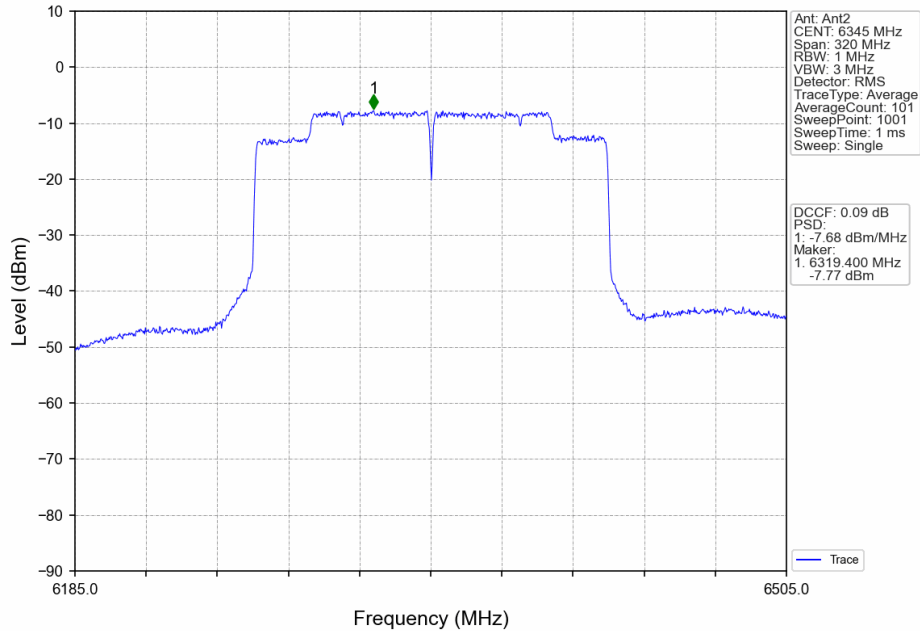
802.11ax(HEW160)_HCH_6345MHz_2xRU996_Left_MIMO_NTNV
