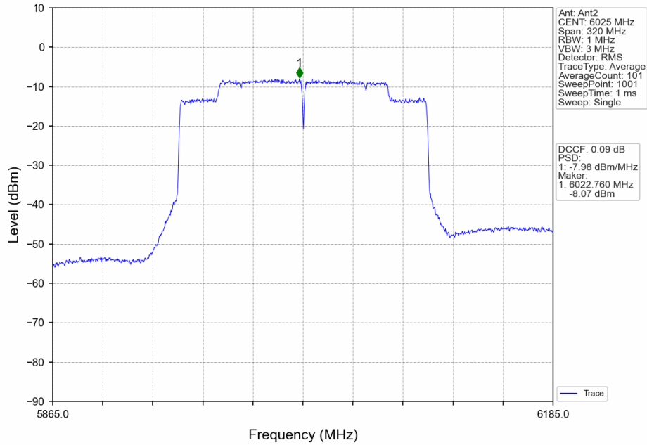
802.11ax(HEW160)_LCH_6025MHz_2xRU996_Left_MIMO_NTNV
