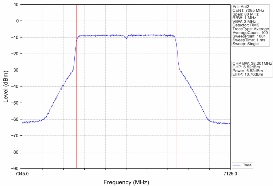
802.11ax(HEW40)_HCH_7085MHz_RU484_Left_Ant2_NTNV
