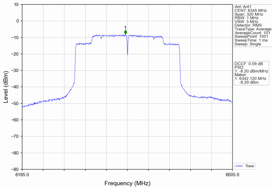
802.11ax(HEW160)_HCH_6345MHz_2xRU996_Left_Ant1_NTNV
