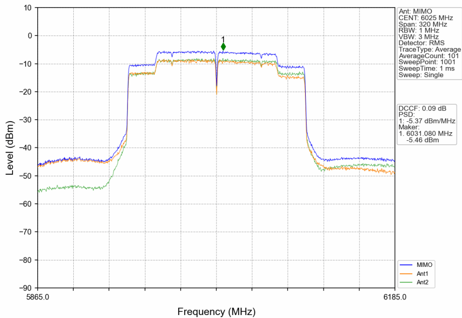
802.11ax(HEW160)_LCH_6025MHz_2xRU996_Left_MIMO_NTNV
