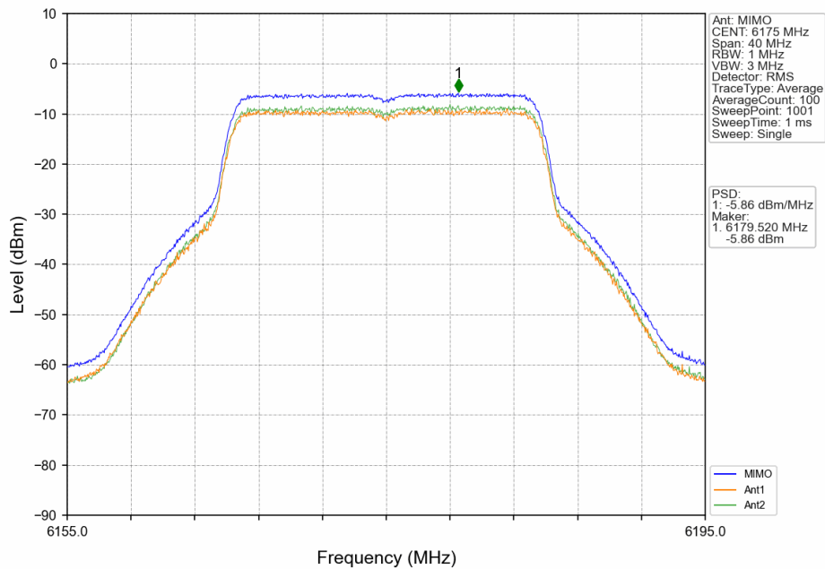
802.11ax(HEW20)_MCH_6175MHz_RU242_Left_MIMO_NTNV
