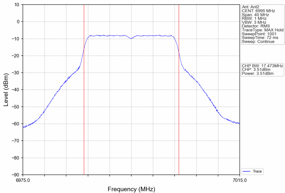
802.11ax(HEW20)_MCH_6995MHz_RU242_Left_Ant2_NTNV
