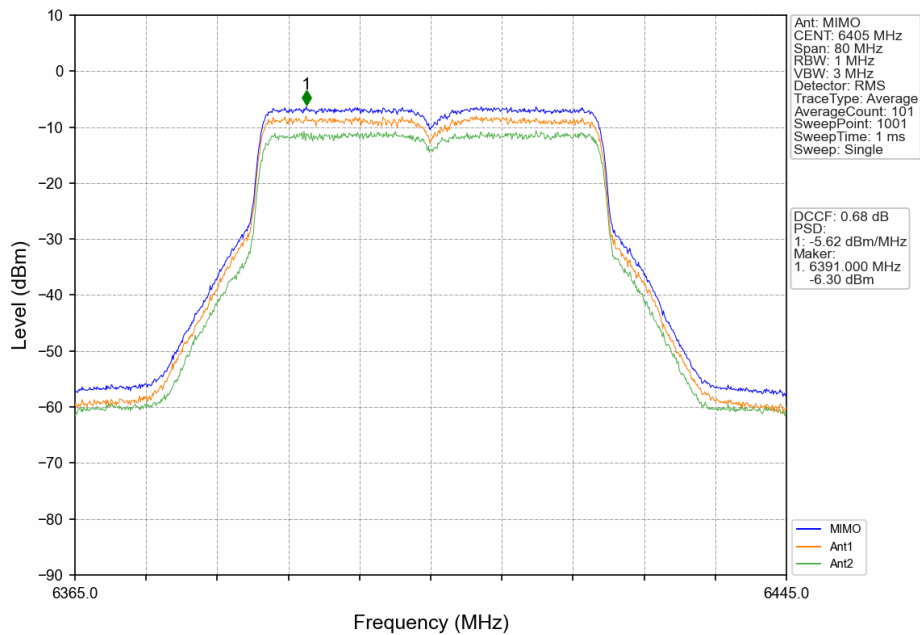
802.11ax(HEW40)_HCH_6405MHz_RU484_Left_MIMO_NTNV
