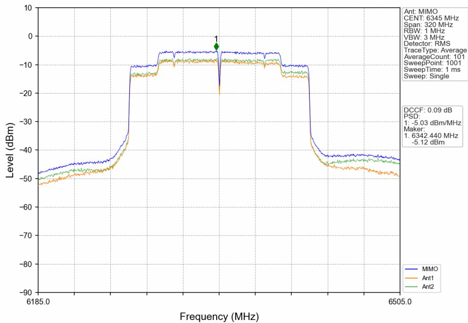
802.11ax(HEW160)_HCH_6345MHz_2xRU996_Left_MIMO_NTNV
