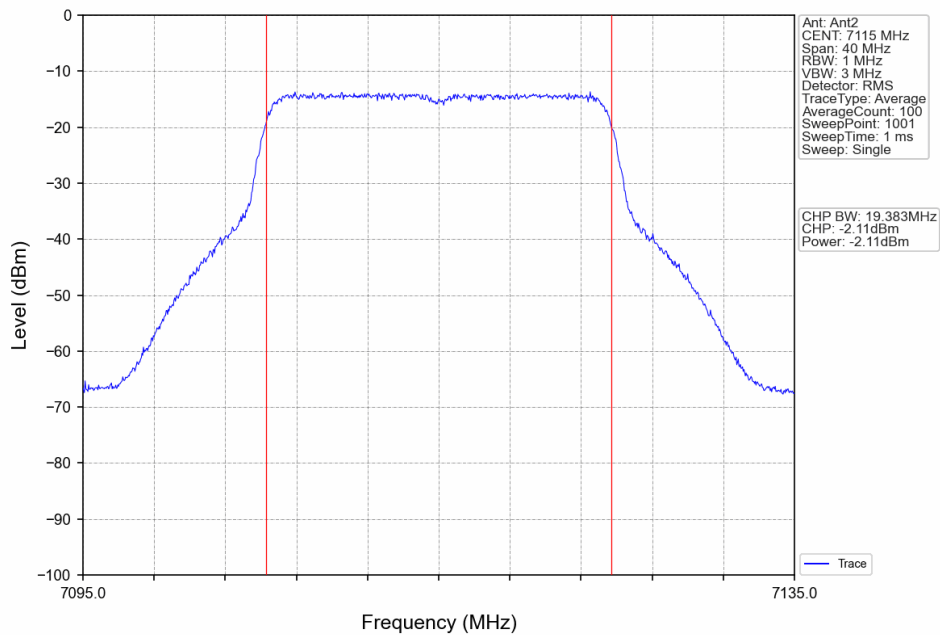
802.11ax(HEW20)_HCH_7115MHz_RU242_Left_Ant2_NTNV
