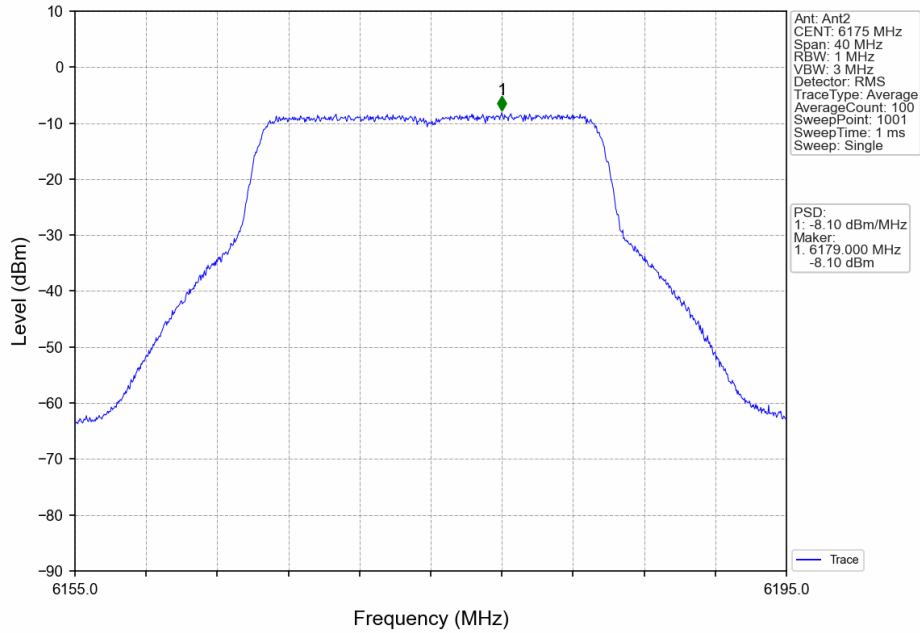
802.11ax(HEW20)_MCH_6175MHz_RU242_Left_MIMO_NTNV
