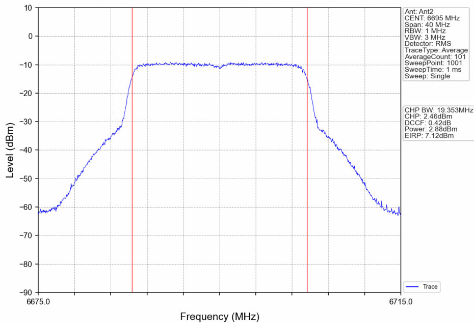
802.11ax(HEW20)_MCH_6695MHz_RU242_Left_Ant2_NTNV
