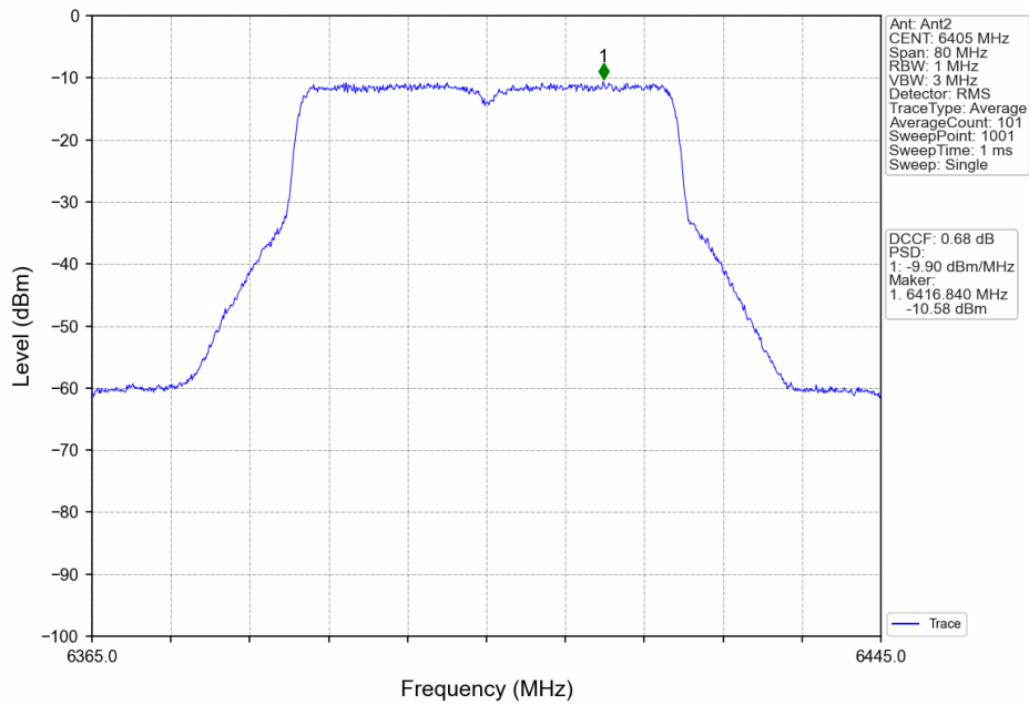
802.11ax(HEW40)_HCH_6405MHz_RU484_Left_MIMO_NTNV
