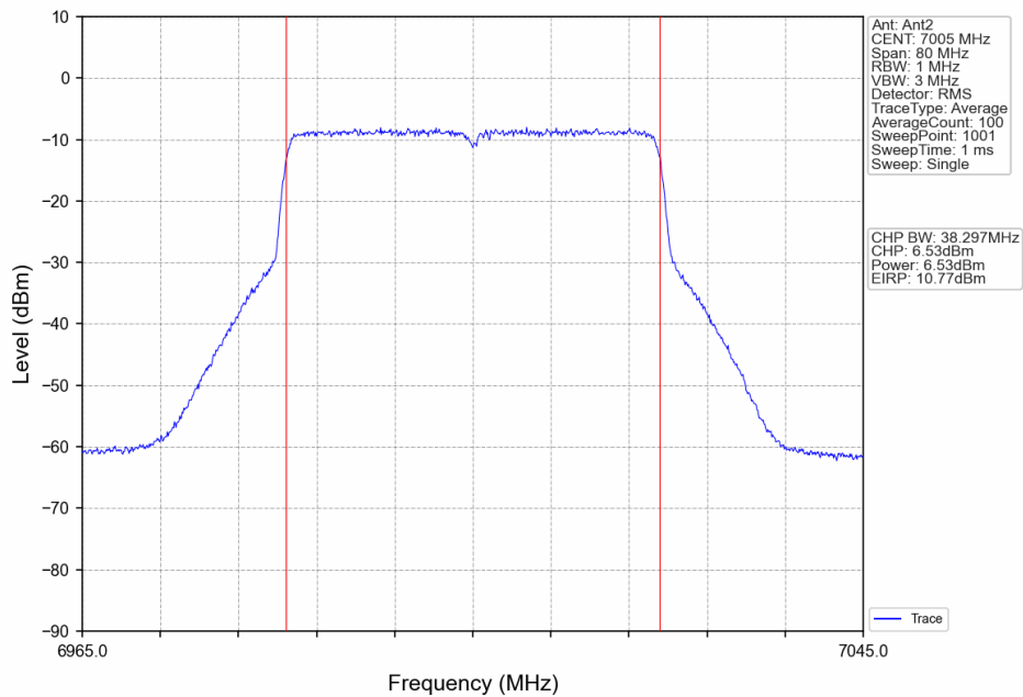
802.11ax(HEW40)_MCH_7005MHz_RU484_Left_Ant2_NTNV
