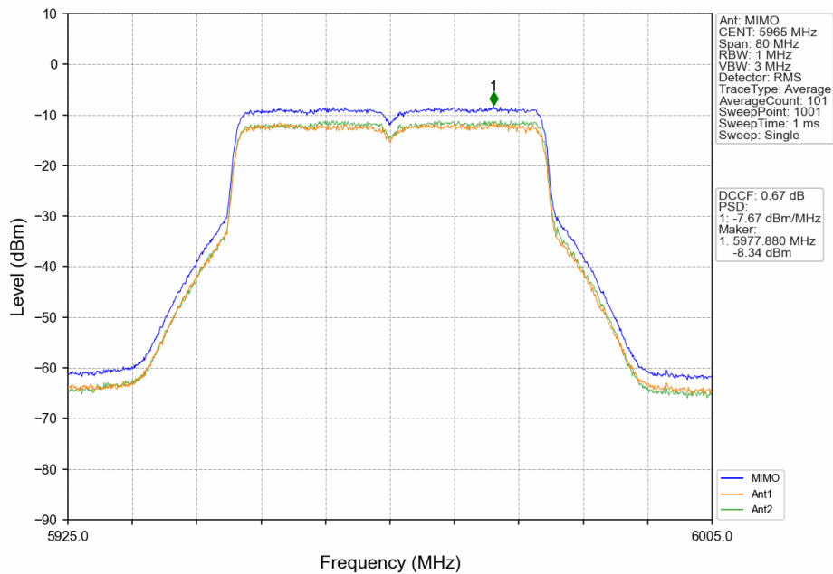
802.11ax(HEW40)_LCH_5965MHz_RU484_Left_MIMO_NTNV
