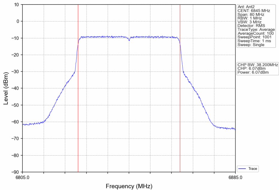
802.11ax(HEW40)_HCH_6845MHz_RU484_Left_Ant2_NTNV
