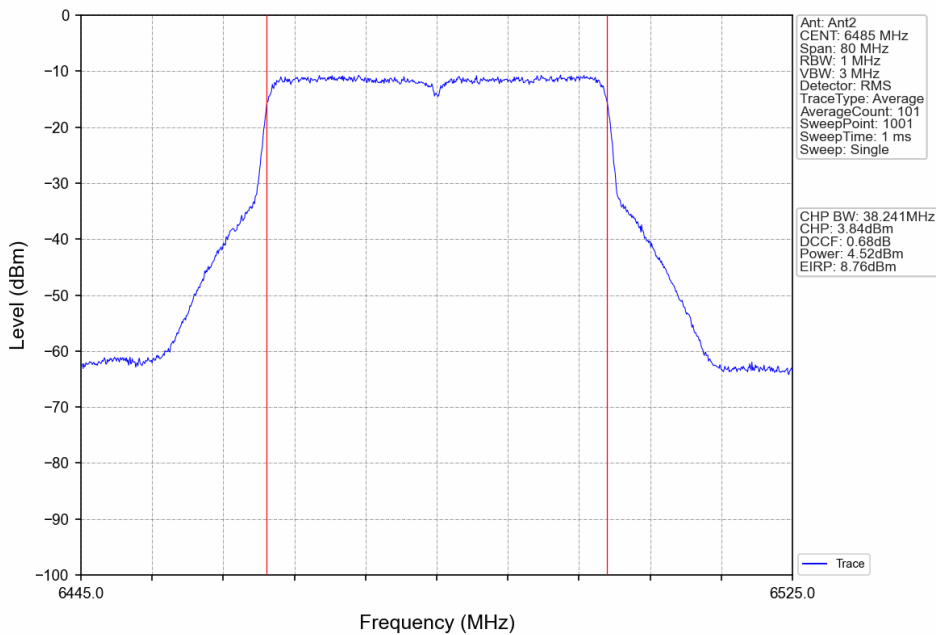
802.11ax(HEW40)_MCH_6485MHz_RU484_Left_Ant2_NTNV
