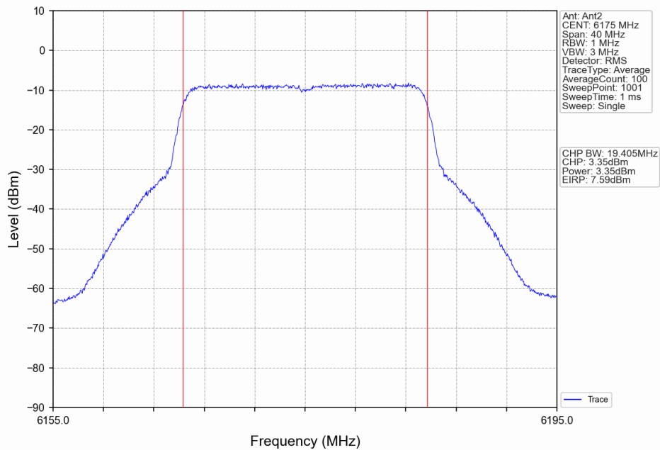
802.11ax(HEW20)_MCH_6175MHz_RU242_Left_Ant2_NTNV
