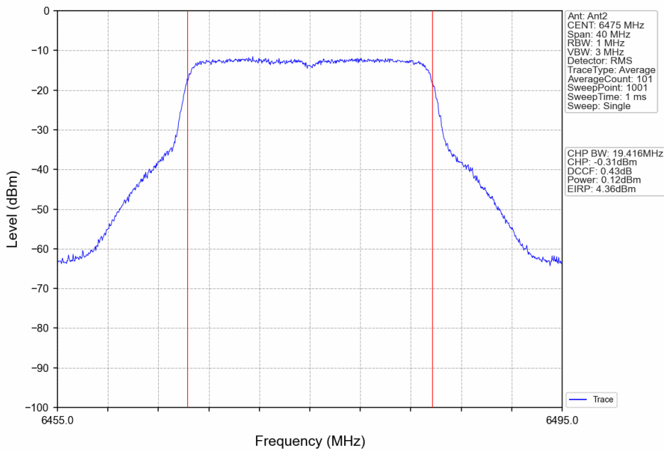
802.11ax(HEW20)_MCH_6475MHz_RU242_Left_Ant2_NTNV
