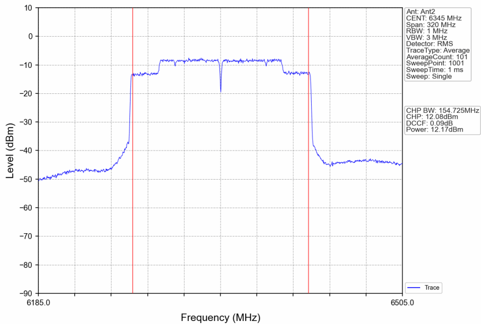
802.11ax(HEW160)_HCH_6345MHz_2xRU996_Left_Ant2_NTNV
