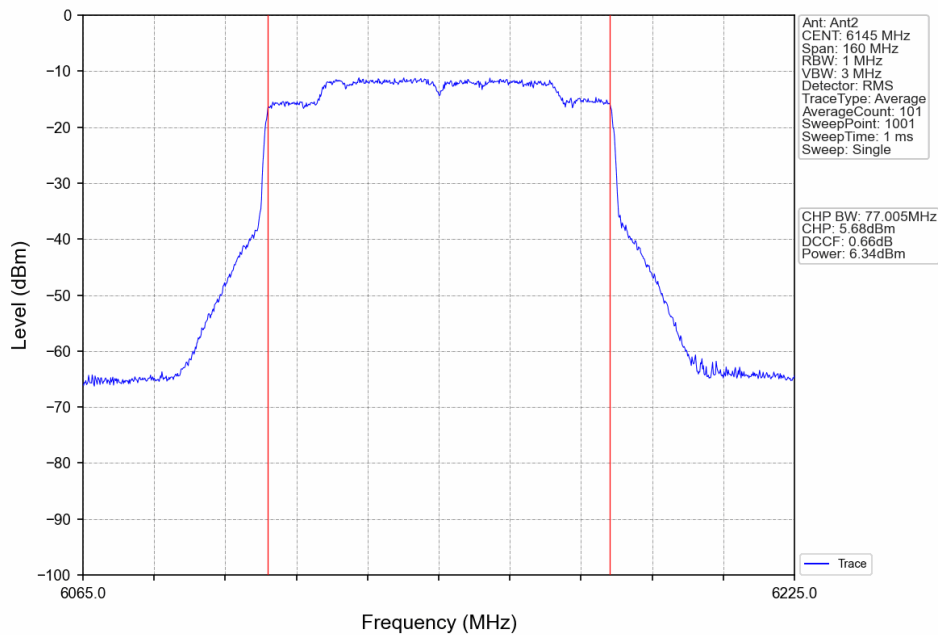
802.11ax(HEW80)_MCH_6145MHz_RU996_Left_Ant2_NTNV
