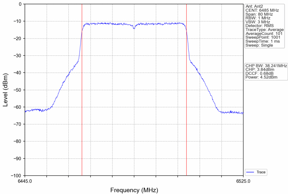
802.11ax(HEW40)_MCH_6485MHz_RU484_Left_Ant2_NTNV
