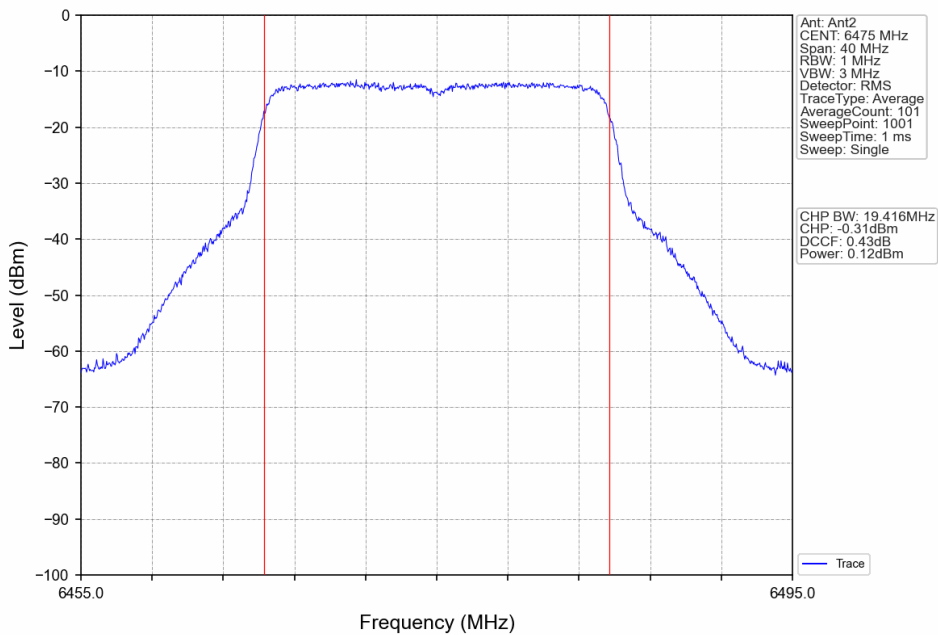
802.11ax(HEW20)_MCH_6475MHz_RU242_Left_Ant2_NTNV
