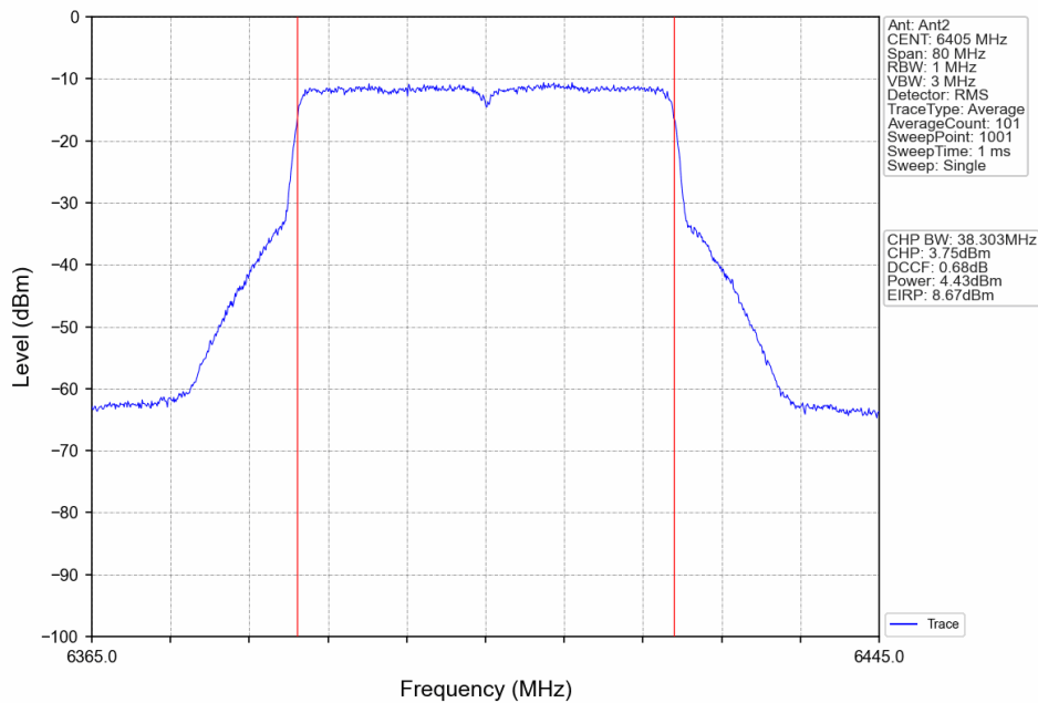
802.11ax(HEW40)_HCH_6405MHz_RU484_Left_Ant2_NTNV
