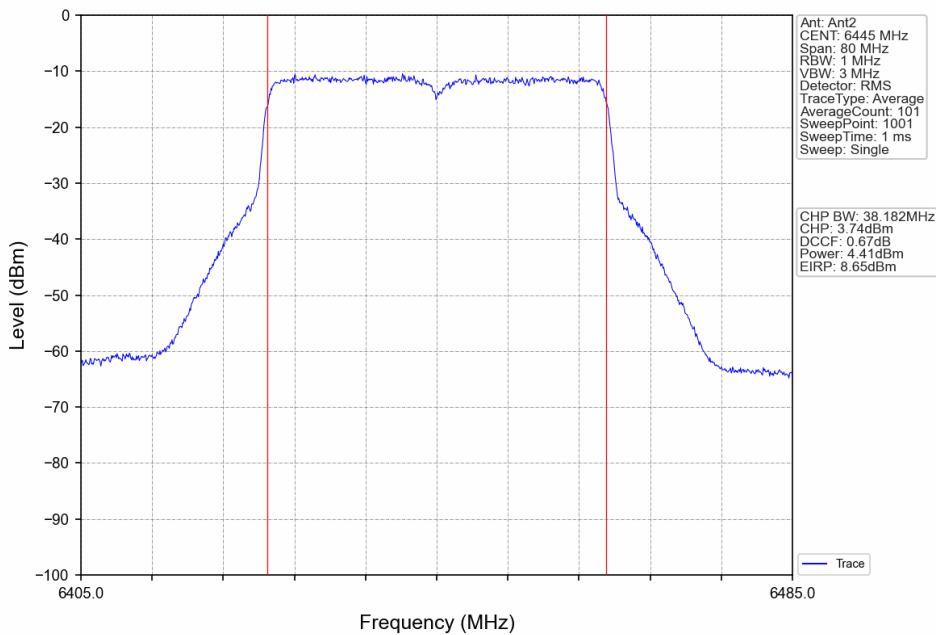
802.11ax(HEW40)_LCH_6445MHz_RU484_Left_Ant2_NTNV
