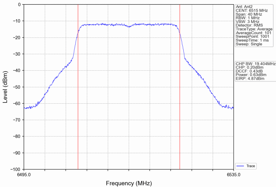
802.11ax(HEW20)_HCH_6515MHz_RU242_Left_Ant2_NTNV
