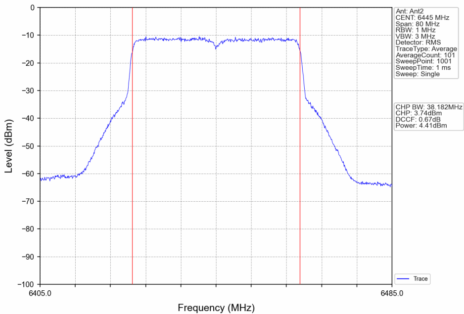
802.11ax(HEW40)_LCH_6445MHz_RU484_Left_Ant2_NTNV
