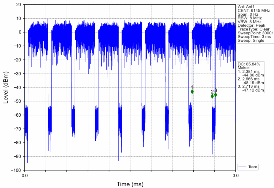
802.11ax(HEW80)_MCH_6145MHz_RU996_Left_Ant1_NTNV
