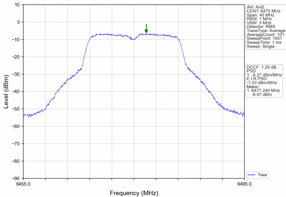
802.11ax(HEW20)_MCH_6475MHz_RU242_Left_Ant2_NTNV
