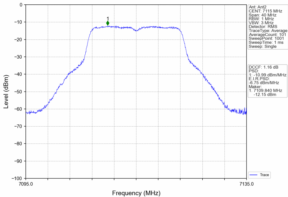
802.11ax(HEW20)_HCH_7115MHz_RU242_Left_Ant2_NTNV
