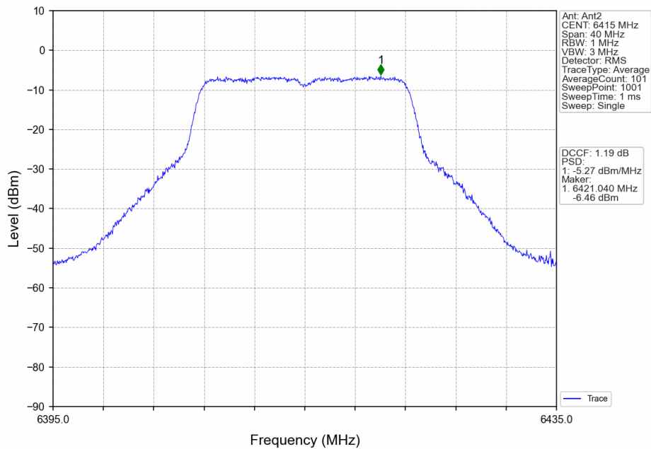
802.11ax(HEW20)_HCH_6415MHz_RU242_Left_Ant2_NTNV
