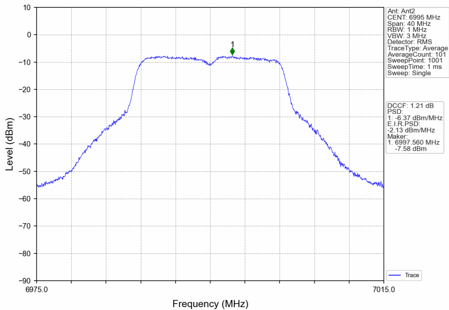
802.11ax(HEW20)_MCH_6995MHz_RU242_Left_Ant2_NTNV
