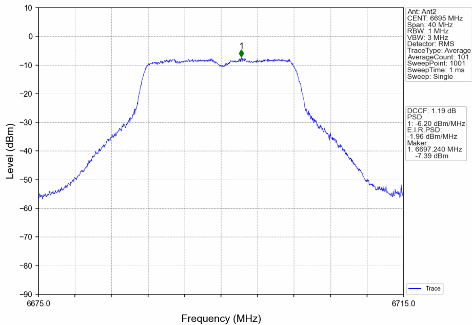
802.11ax(HEW20)_MCH_6695MHz_RU242_Left_Ant2_NTNV
