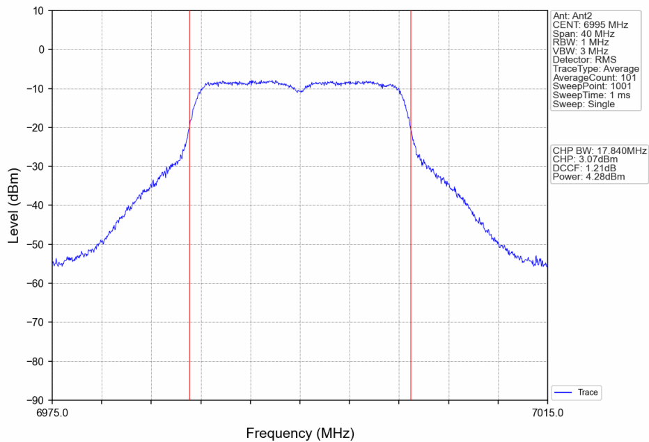
802.11ax(HEW20)_MCH_6995MHz_RU242_Left_Ant2_NTNV
