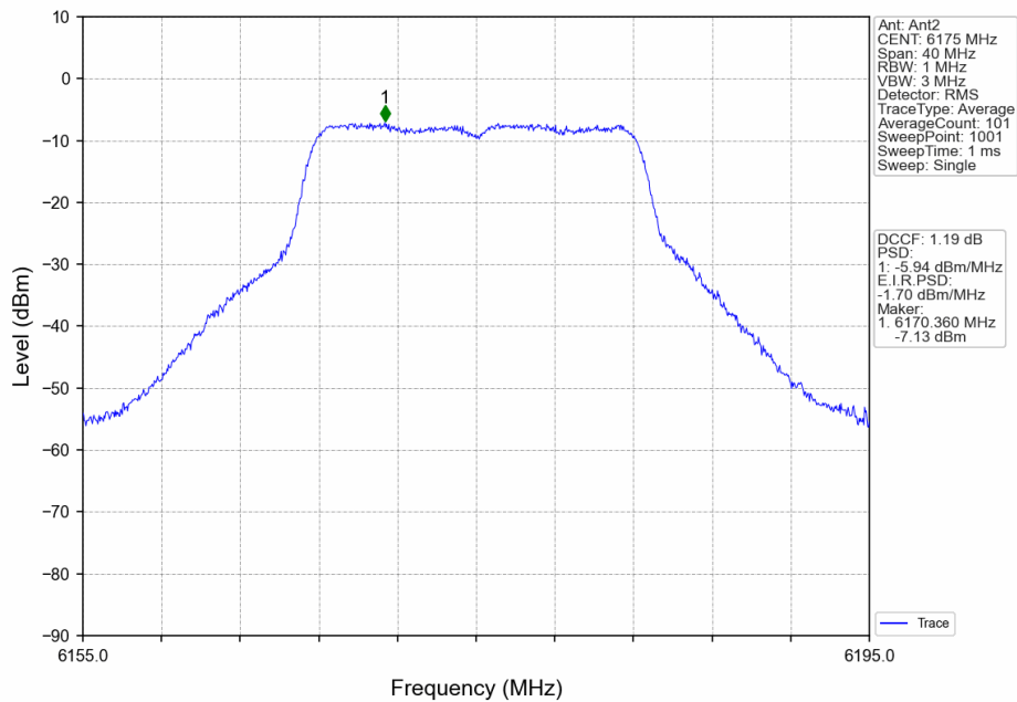
802.11ax(HEW20)_MCH_6175MHz_RU242_Left_Ant2_NTNV
