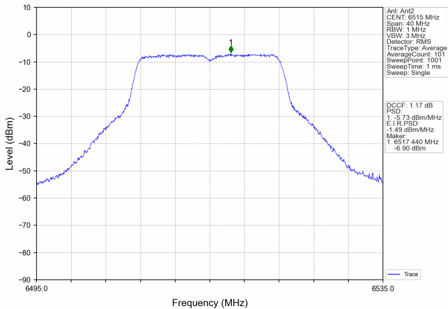
802.11ax(HEW20)_HCH_6515MHz_RU242_Left_Ant2_NTNV
