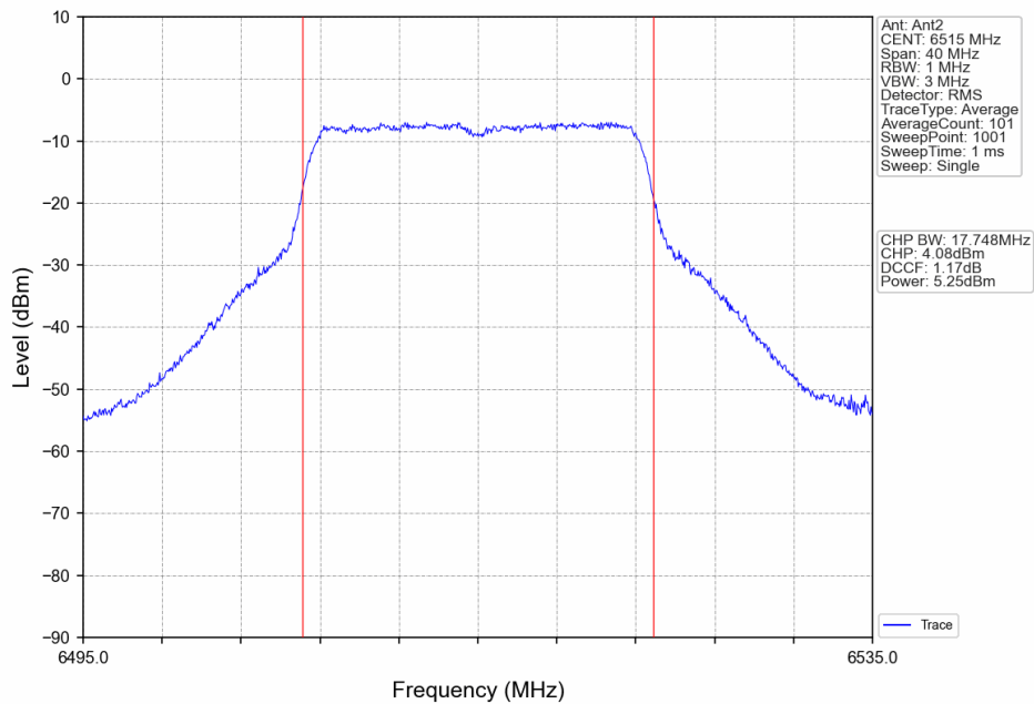
802.11ax(HEW20)_HCH_6515MHz_RU242_Left_Ant2_NTNV
