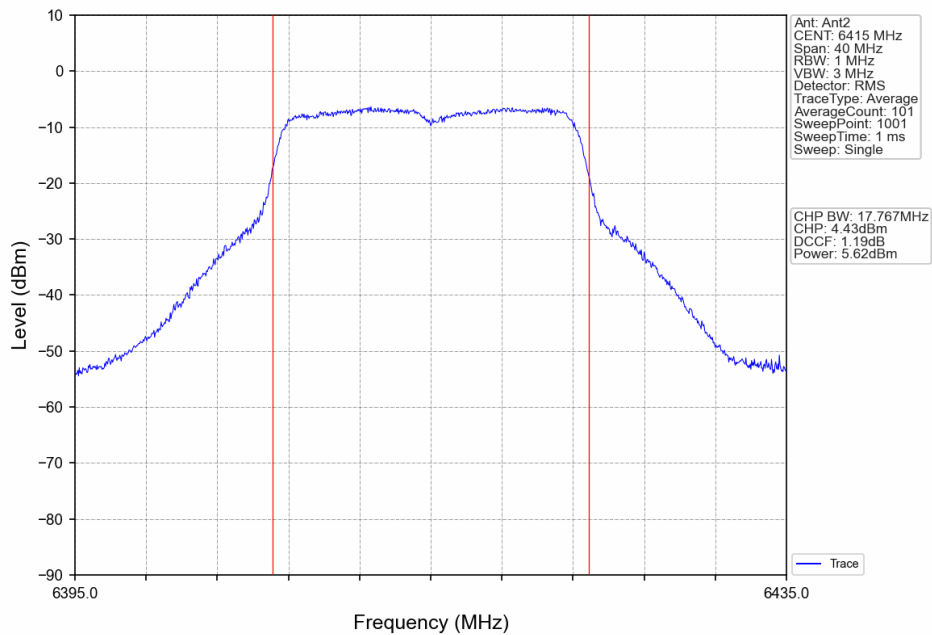
802.11ax(HEW20)_HCH_6415MHz_RU242_Left_Ant2_NTNV
