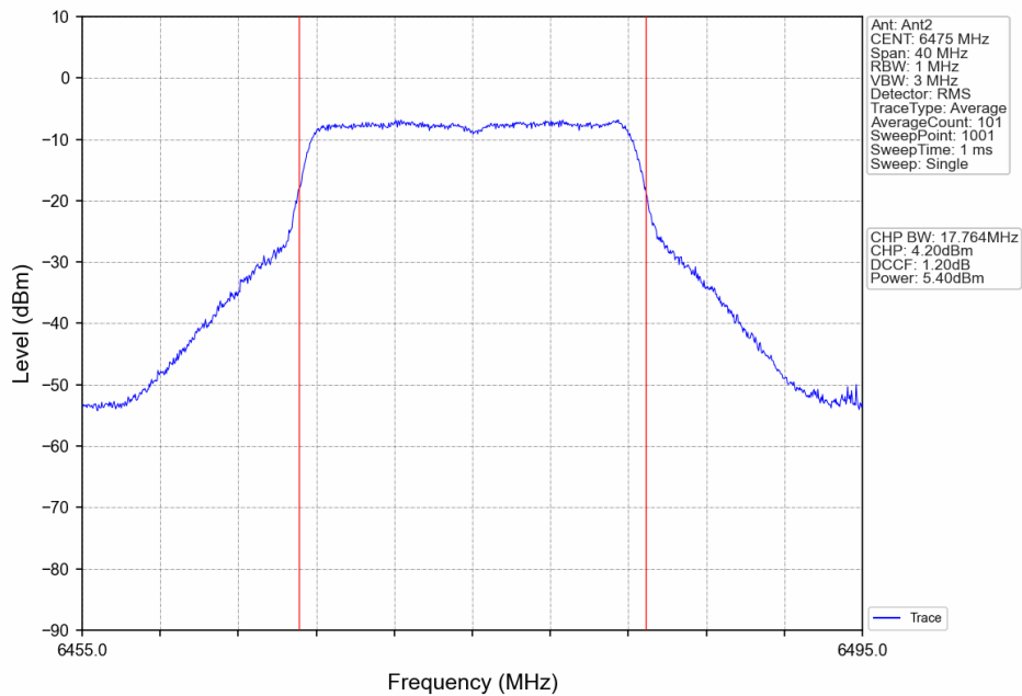
802.11ax(HEW20)_MCH_6475MHz_RU242_Left_Ant2_NTNV
