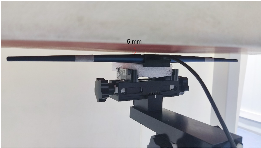
Open-0° (5mm)
