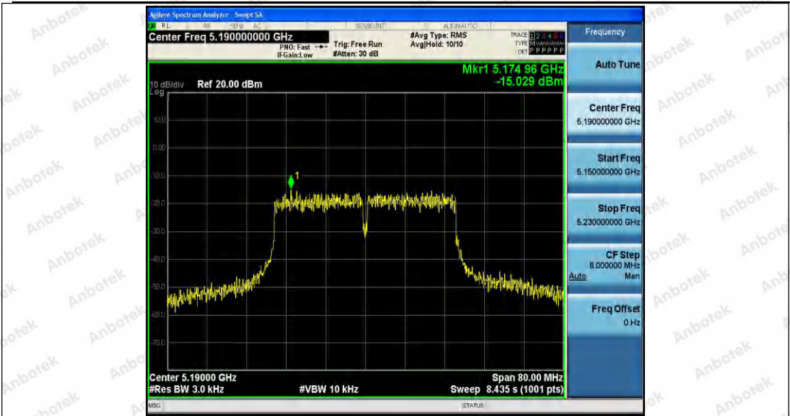
11N40SISO_Ant2_5190
