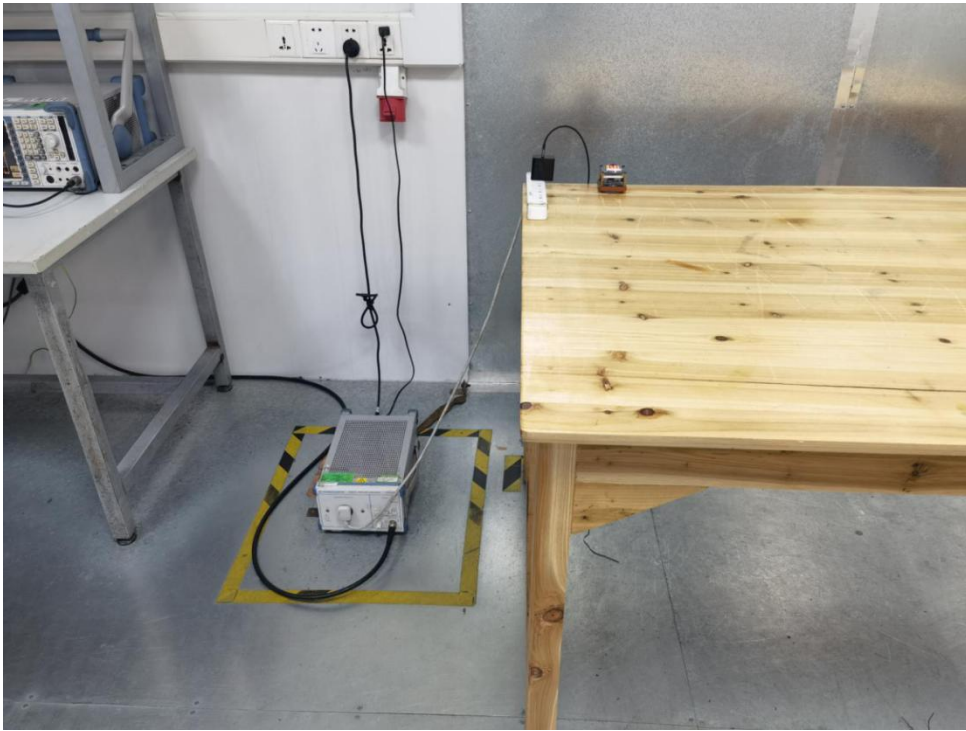
FCC ID: 2AQI5-CD245 Photo of Conducted Emission Measurement
